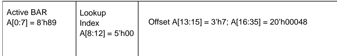
Figure 6: PCI/X Path Address Translation Process, 36-bit Processor
