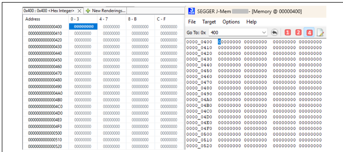
Figure 42. Secure Data Region is not Viewable
