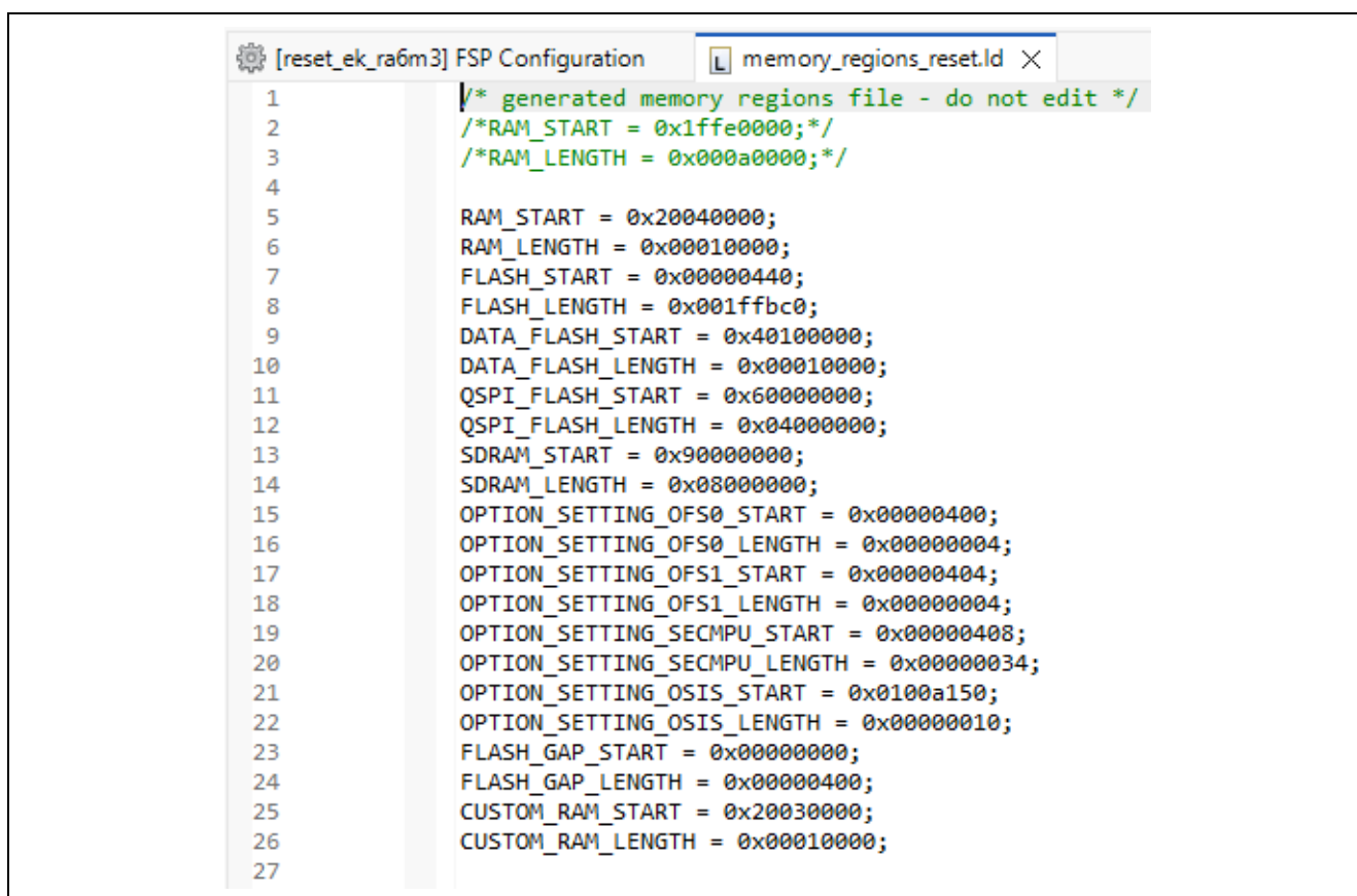
Figure 43. Customized Linker Script for reset_ek_ra6m3 Project
