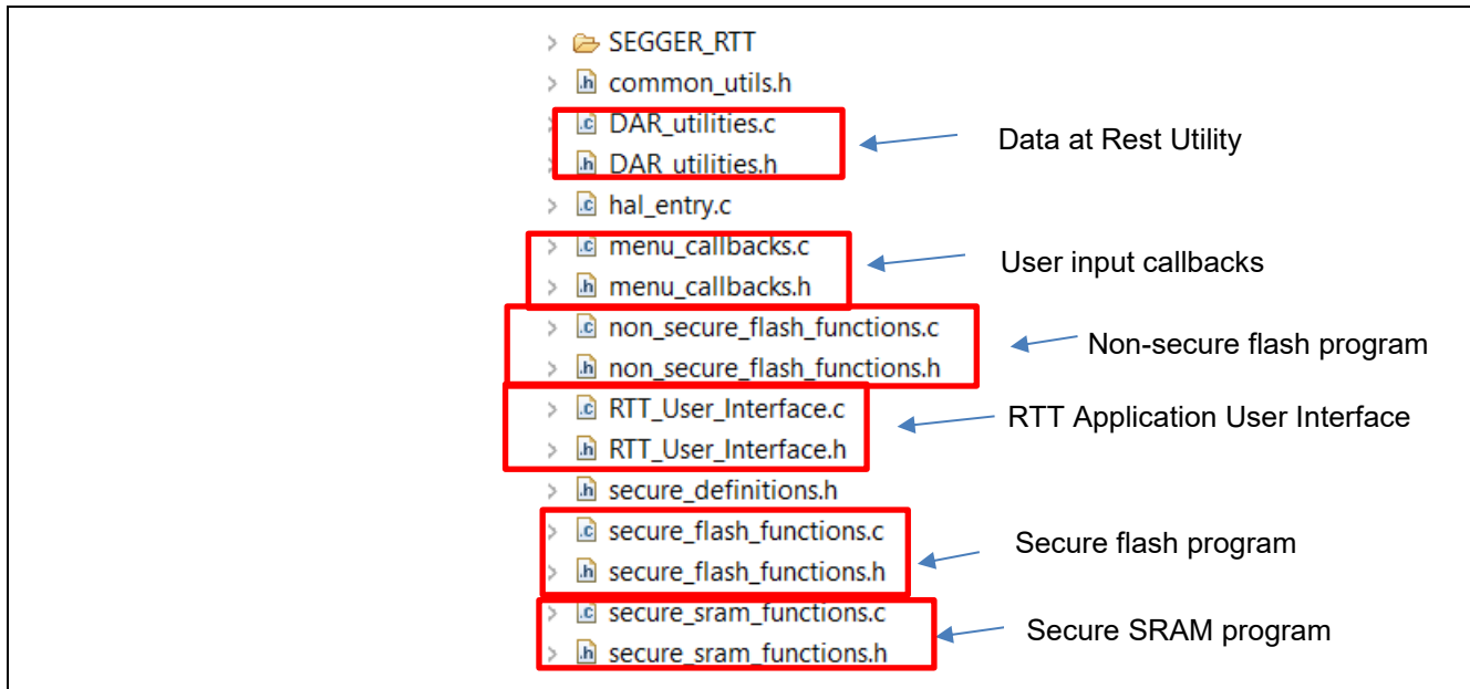
Figure 23. Source Code
