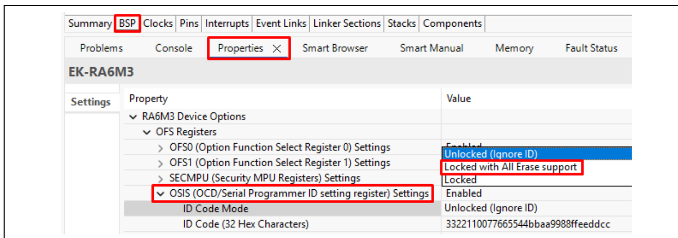
Figure 13. Setting up OSIS ID using RA MCU Configurator
