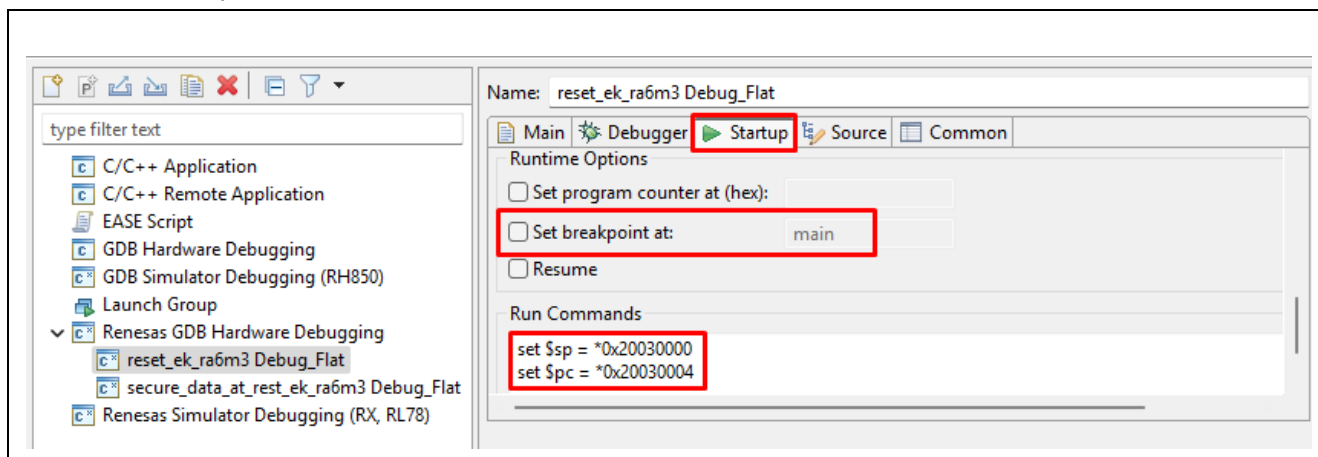
Figure 44. Set up the SP and PC
