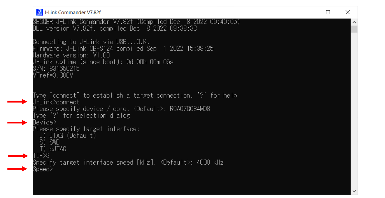
Figure 5-2 Connection conditions (1/2)
