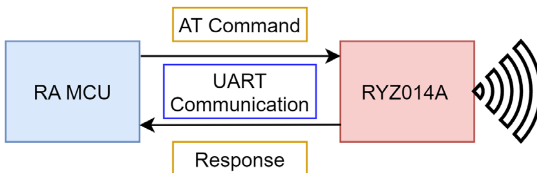
Figure 2. Communication of RYZ014A and host MCU
