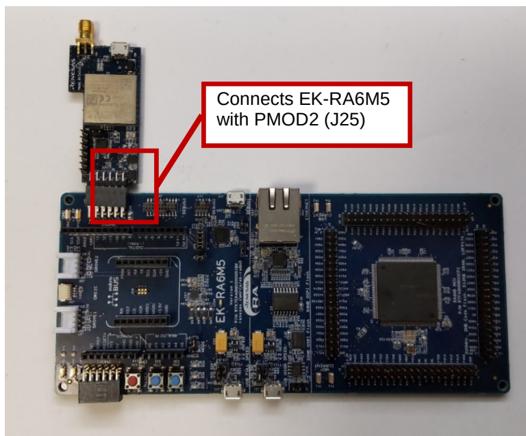
Figure 3. Connect EK-RA6M5 and RYZ014A
