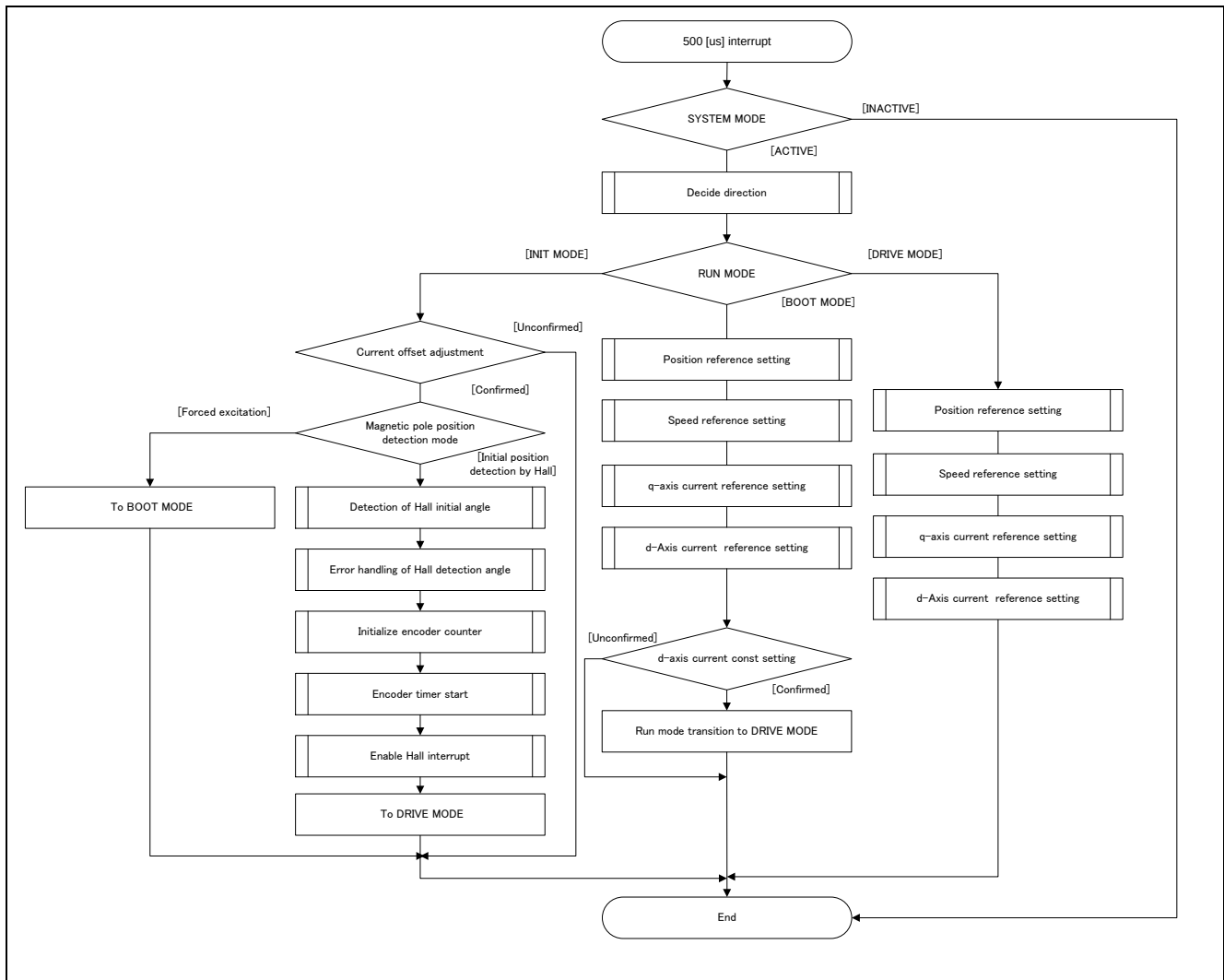
Figure 3-11 500 [μs] Interrupt Handling
