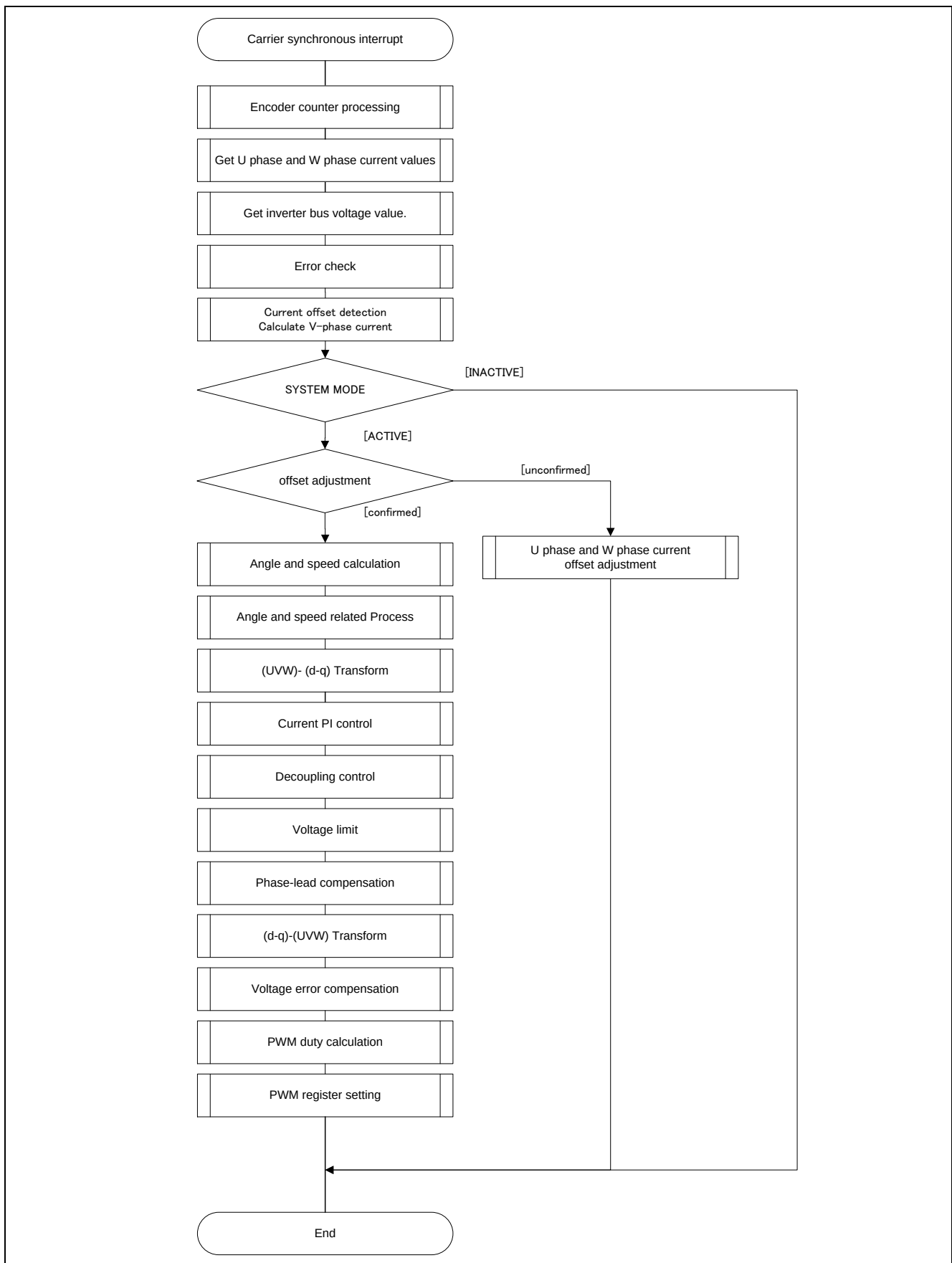
Figure 3-10 50 [μs] Cycle Interrupt Handling
