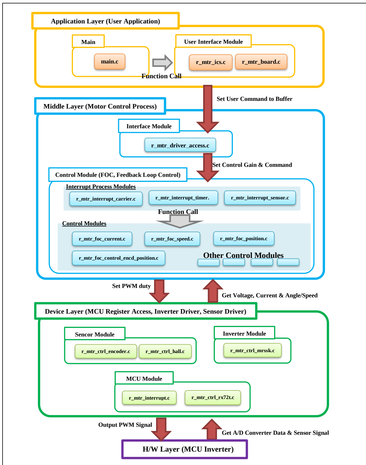
Figure 2-3 Module Configuration
