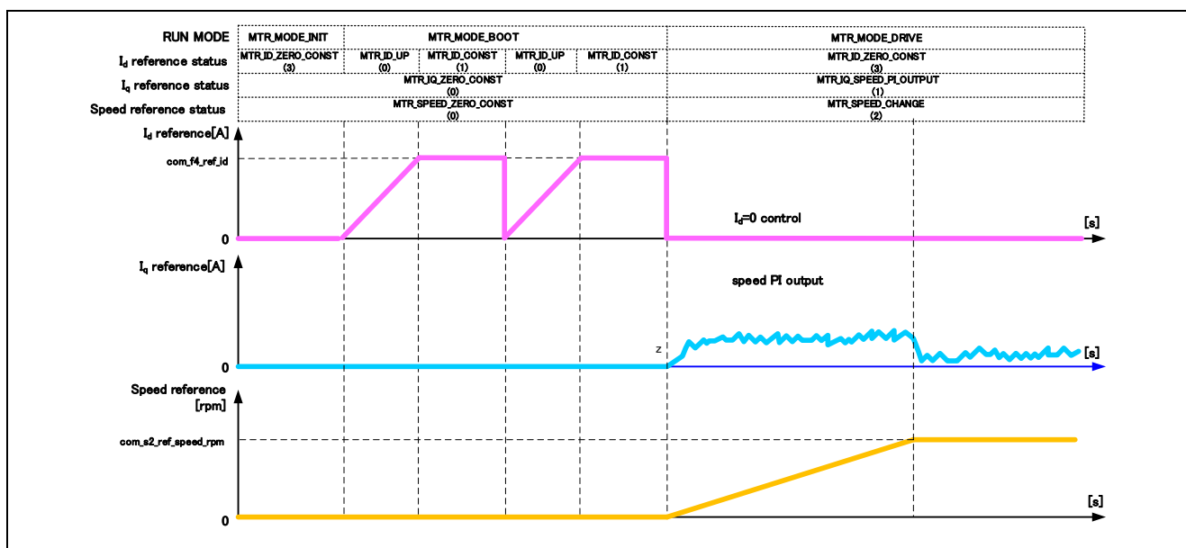
Figure 3-7 Startup Speed Control of Vector Control PMSM with Encoder Software
