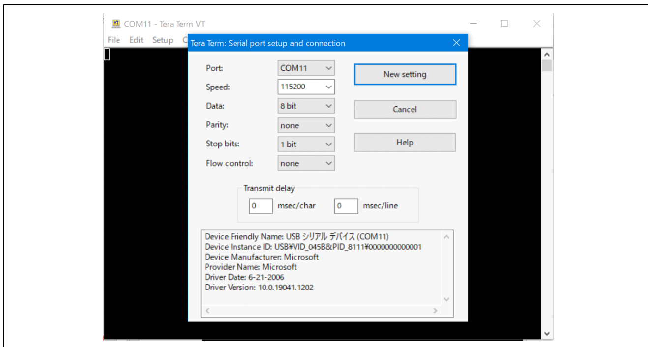
図 8-21 Tera Term
