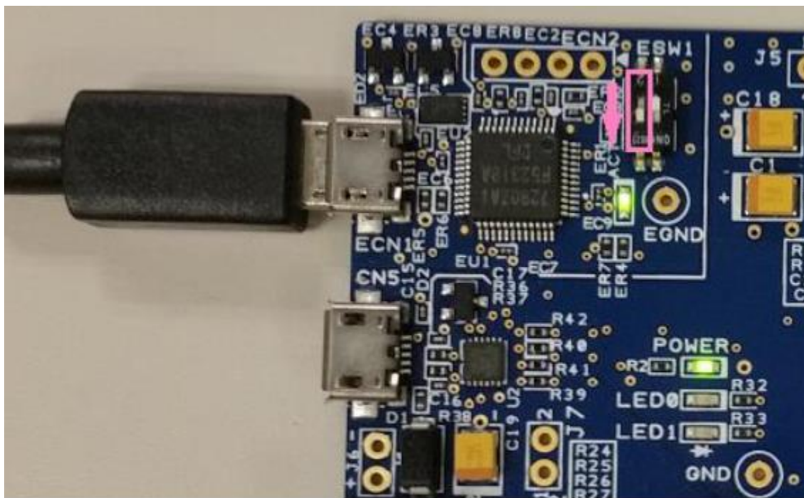
Figure 5.1 Write programs
