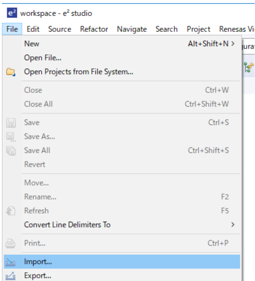
Figure 5.8 File menu
