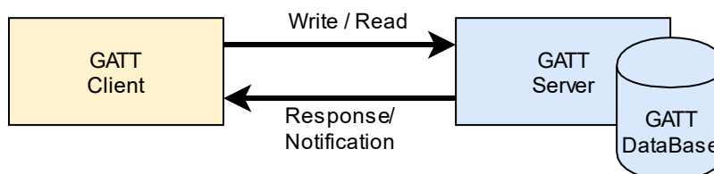
Figure 3.11 GATT architecture
