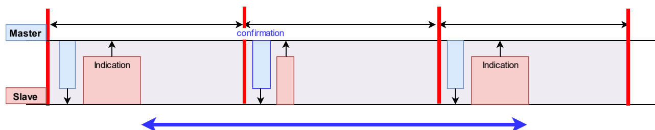
Figure 3.16 Schematic diagram of Link Layer during Indication operation
