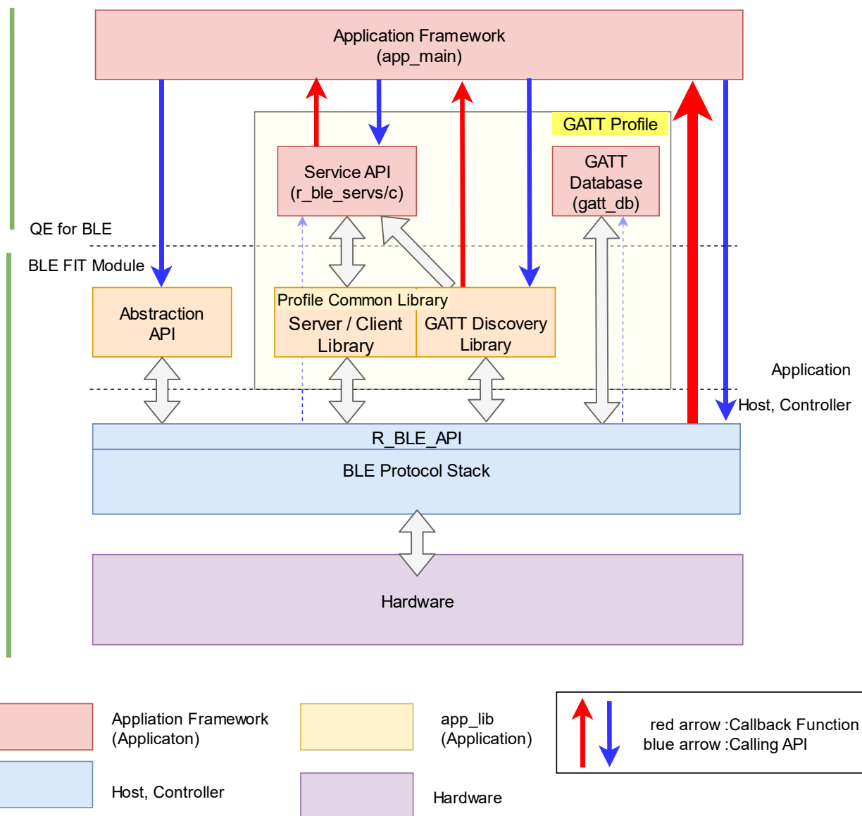
Figure 4.2 Application framework generated by QE for BLE
