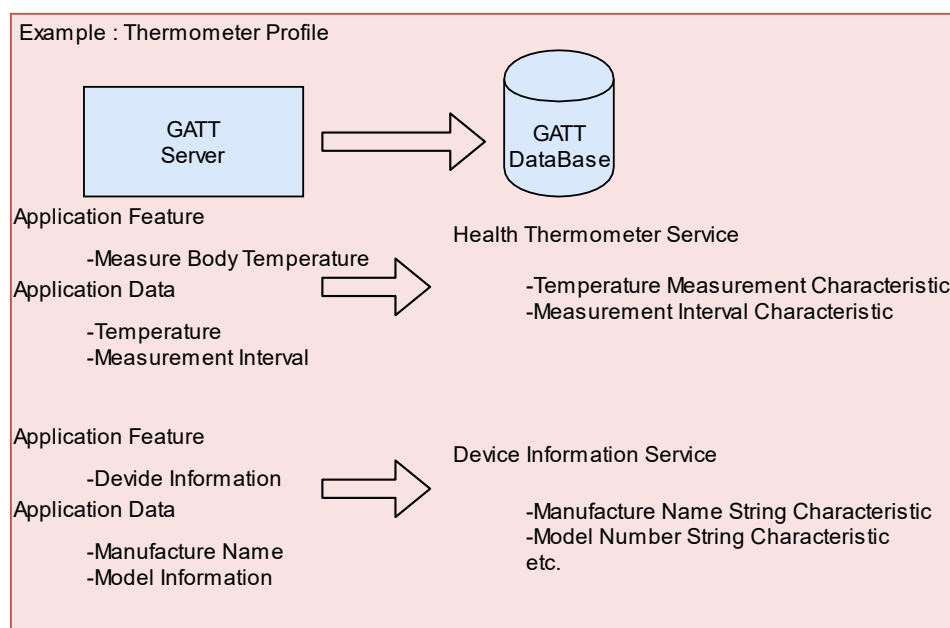
Figure 3.12 Application Data and GATT database
