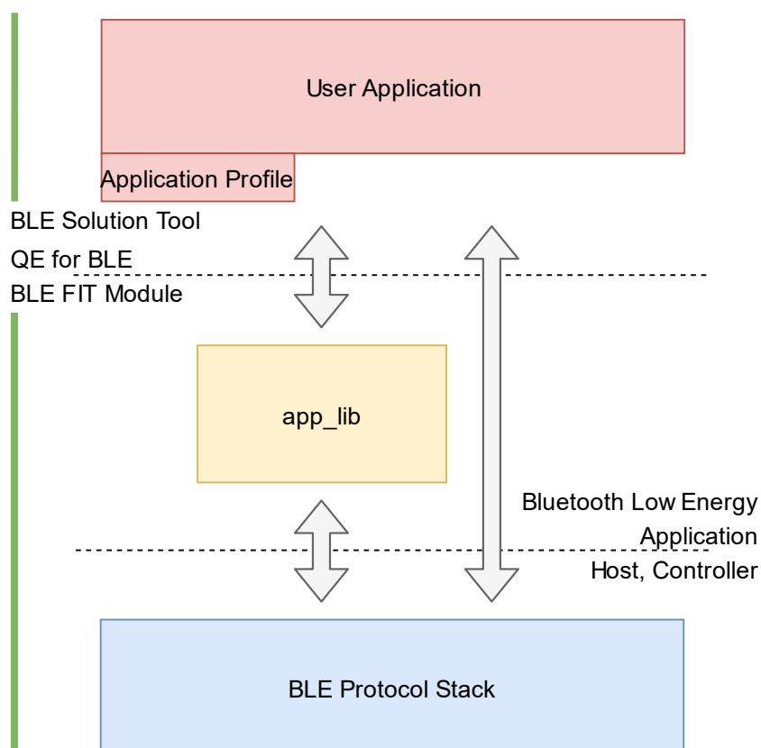
Figure 4.1 BLE Solution Tools and Bluetooth Low Energy Application Configuration
