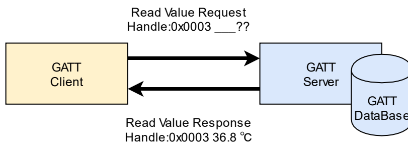
Figure 3.14 Read operation
