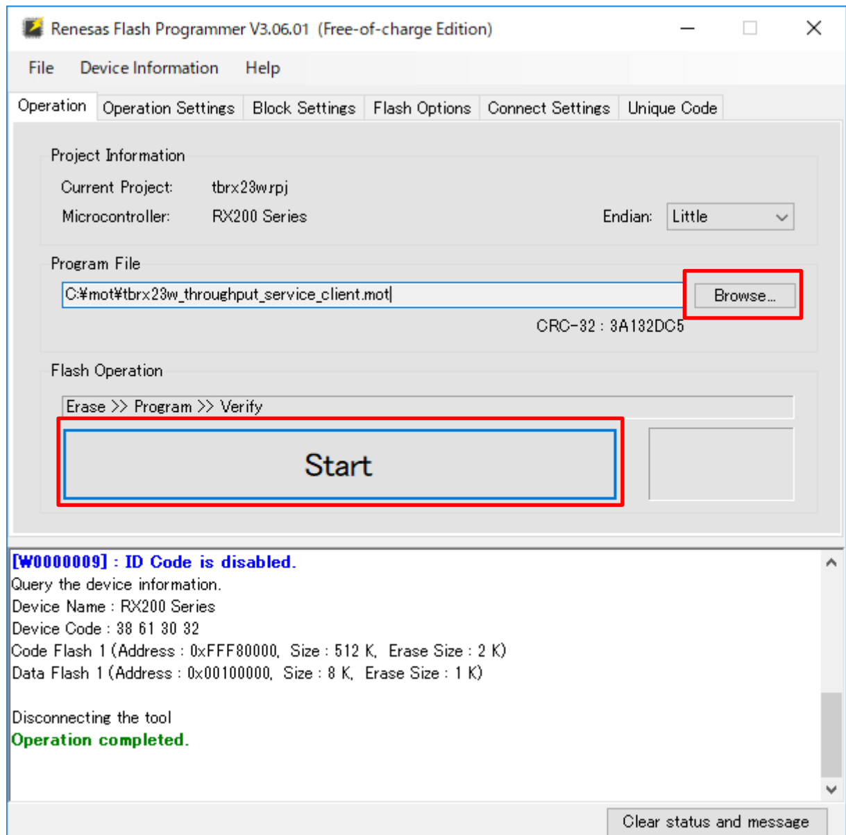
Figure 5.6 Programming Firmware
