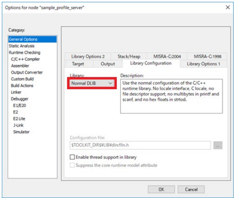
Figure 4-49 : Library Configuration
