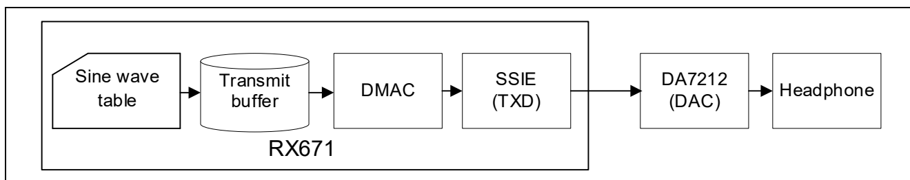
Figure 1.2 Sine wave generation block diagram
