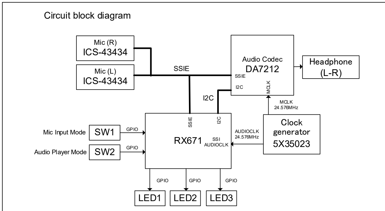
Figure 1.1 Block diagram
