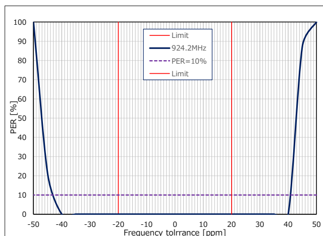
Figure 48 RF Frequency tolerance vs. Packet Error Rate (Frequency = 924.2MHz)
