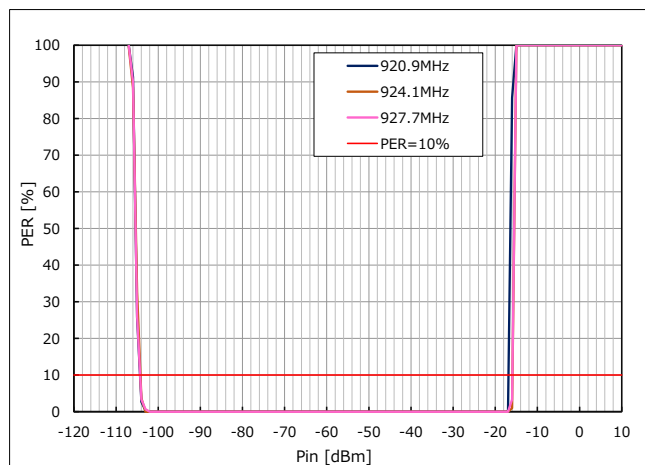
Figure 36 RF Input Level vs. Packet Error Rate (Frequency = 920.9 / 924.1 / 927.7MHz)
