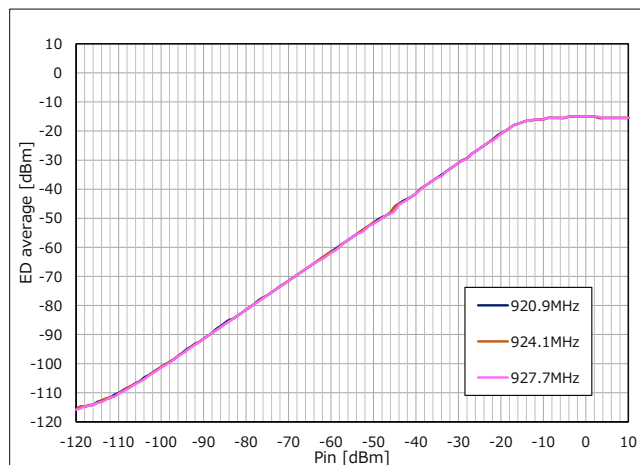
Figure 32 RF Input Level vs. ED average (Frequency = 920.9 / 924.1 / 927.7MHz)
