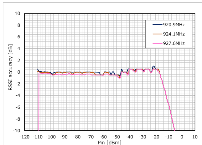
Figure 31 RF Input Level vs. RSSI accuracy (Frequency = 920.9 / 924.1 / 927.7MHz)
