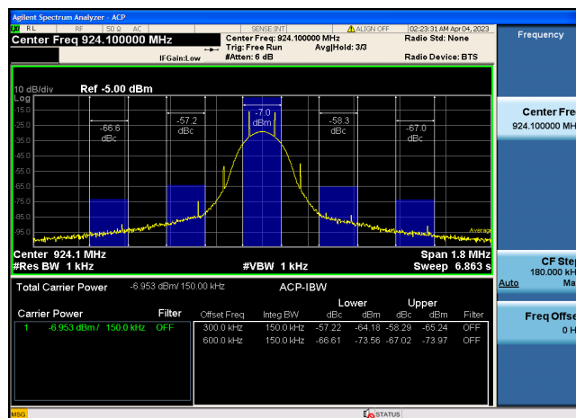
Figure 8 Transmit Spectrum (Frequency = 924.1MHz)
