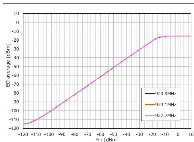
Figure 39 RF Input Level vs. ED average (Frequency = 920.9 / 924.1 / 927.7MHz)
