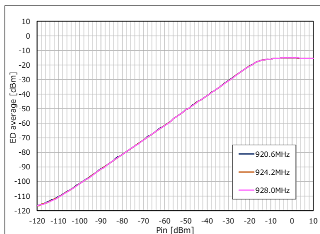
Figure 46 RF Input Level vs. ED average (Frequency = 920.6 / 924.2 / 928.0MHz)
