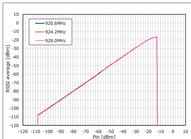
Figure 44 RF Input Level vs. RSSI average (Frequency = 920.6 / 924.2 / 928.0MHz)
