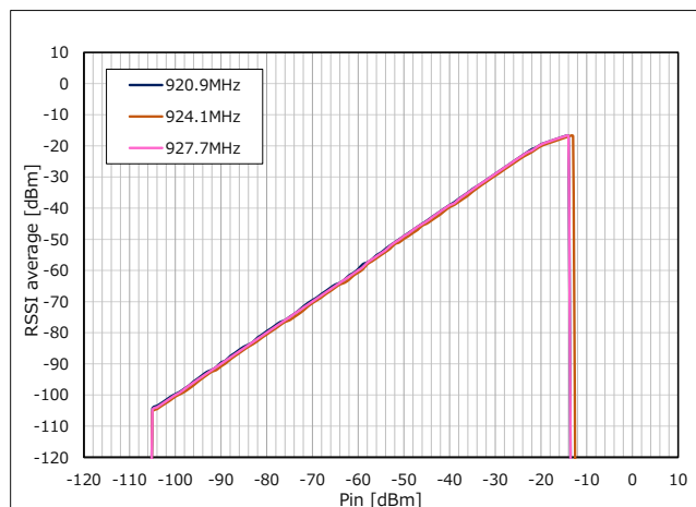
Figure 37 RF Input Level vs. RSSI average (Frequency = 920.9 / 924.1 / 927.7MHz)
