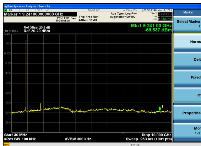
Figure 10 TX Spurious emission (Frequency = 924.1MHz)
