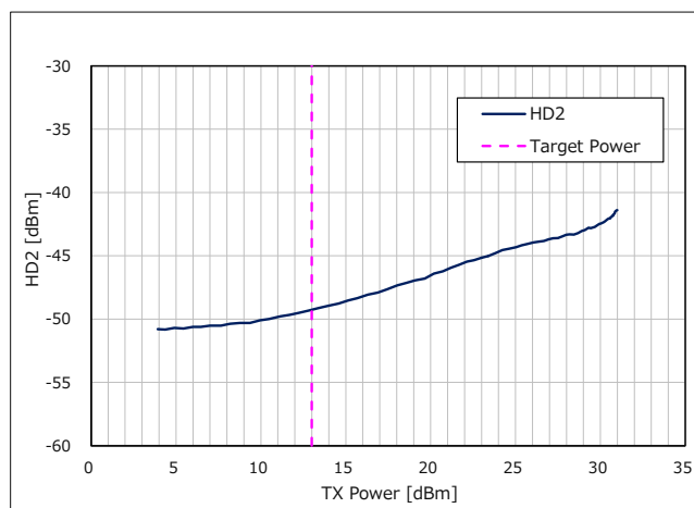
Figure 23 TX Power vs. 2nd Harmonics (Frequency = 924.2MHz)
