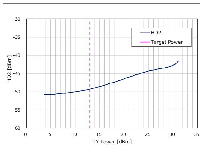
Figure 14 TX Power vs. 2nd Harmonics (Frequency = 924.1MHz)
