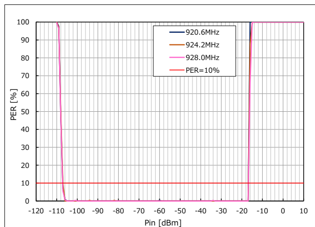
Figure 43 RF Input Level vs. Packet Error Rate (Frequency = 920.6 / 924.2 / 928.0MHz)
