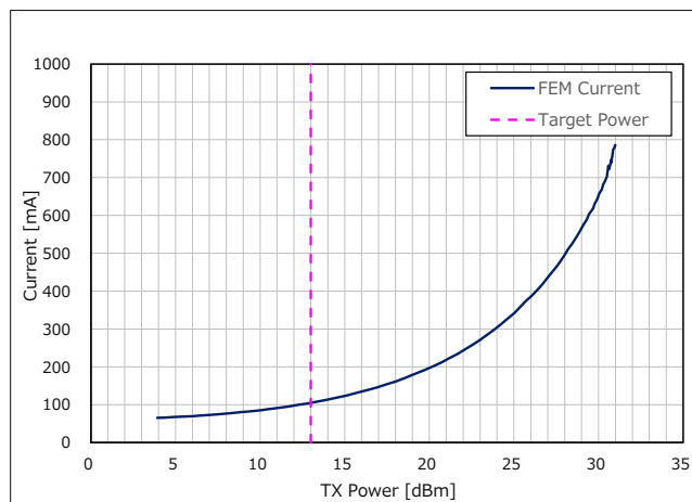
Figure 21 TX Power vs. Current of V_{FEM} for TX mode (Frequency = 924.2MHz)
