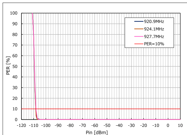
Figure 29 RF Input Level vs. Packet Error Rate (Frequency = 920.9 / 924.1 / 927.7MHz)
