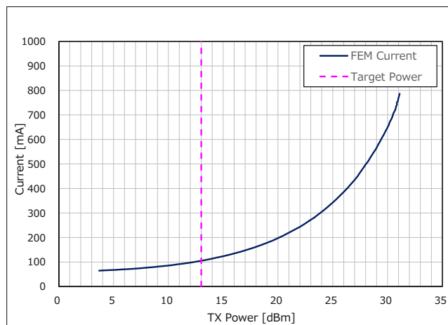
Figure 12 TX Power vs. Current of V_{FEM} for TX mode (Frequency = 924.1MHz)
