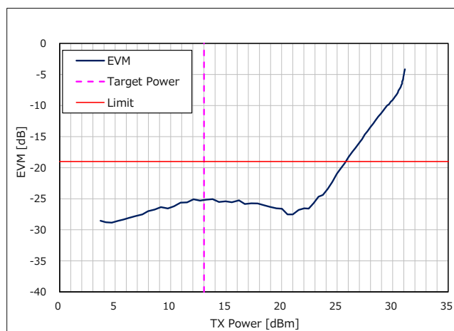
Figure 16 TX Power vs. EVM (Frequency = 924.1MHz)
