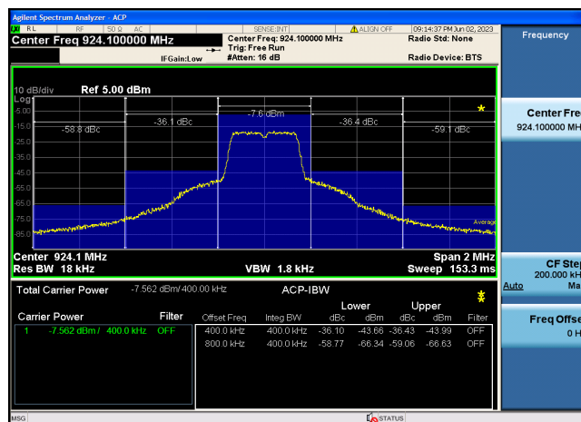
Figure 18 Transmit Spectrum (Frequency = 924.1MHz)
