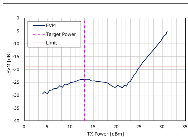
Figure 25 TX Power vs. EVM (Frequency = 924.2MHz)
