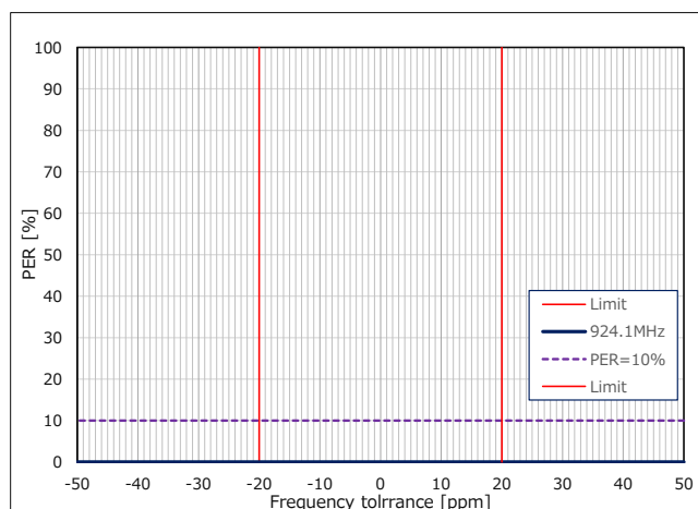
Figure 34 RF Frequency tolerance vs. Packet Error Rate (Frequency = 924.1MHz)
