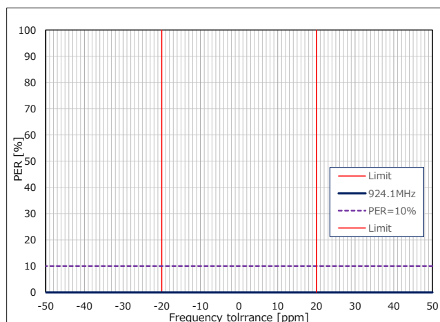
Figure 41 RF Frequency tolerance vs. Packet Error Rate (Frequency = 924.1MHz)
