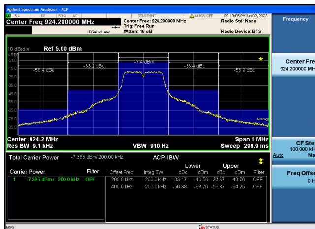
Figure 27 Transmit Spectrum (Frequency = 924.2MHz)
