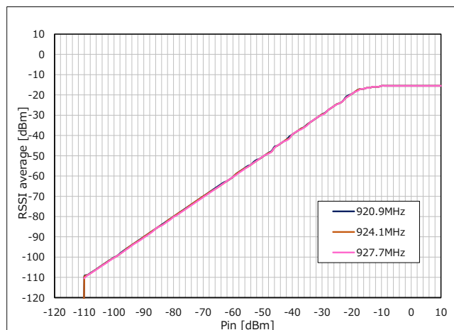
Figure 30 RF Input Level vs. RSSI average (Frequency = 920.9 / 924.1 / 927.7MHz)
