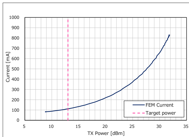
Figure 3 TX Power vs. Current of V_{FEM} for TX mode (Frequency =924.1MHz)
