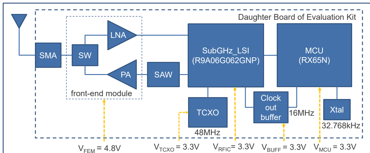
Figure 1 System Configuration
