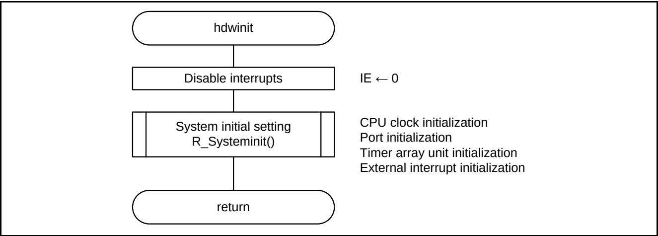
Figure 5.2 Initialization Function
