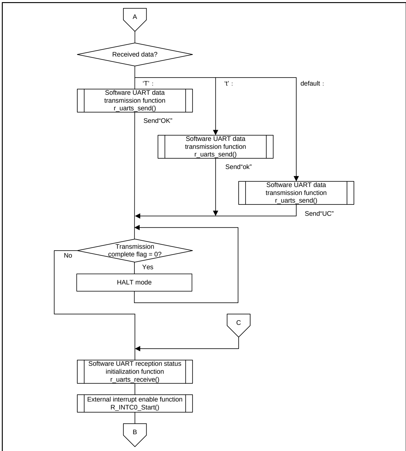
Figure 5.9 Main Processing (2/2)
