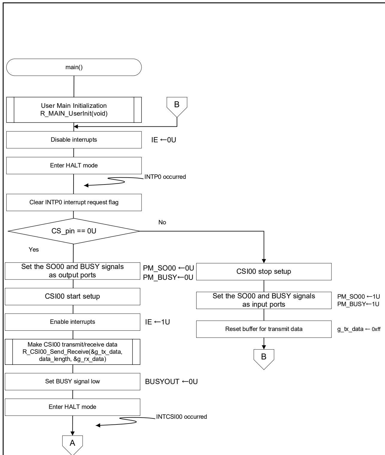
Figure 5-8 Main Processing 1/2
