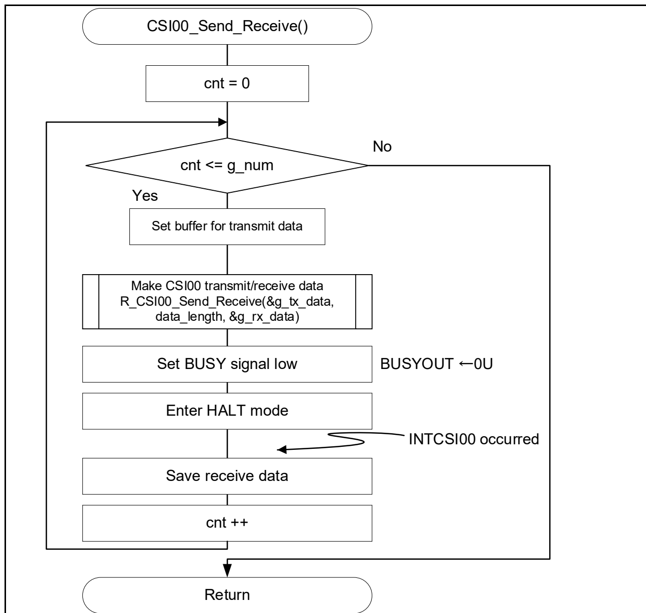
Figure 5-15 CSI Transmission/Reception
