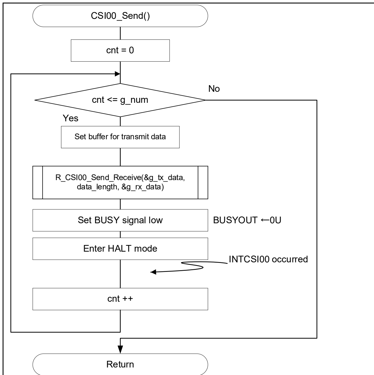
Figure 5-16 CSI Transmission
