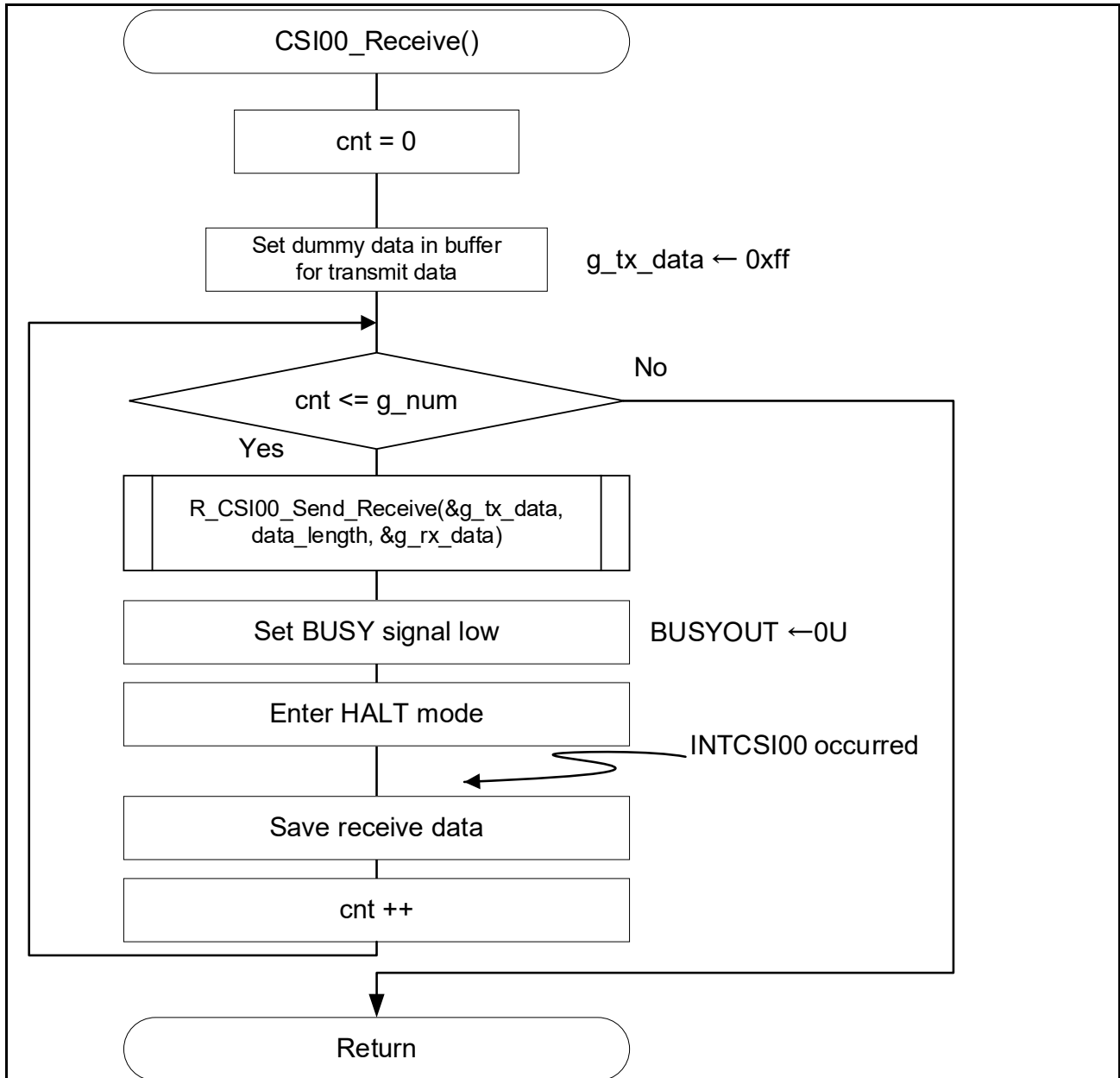
Figure 5-17 CSI Reception
