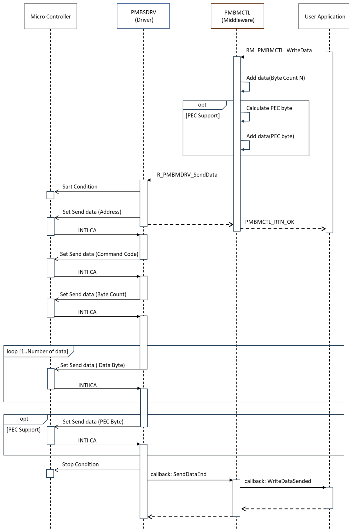
図 5-4 Block Write sequence
