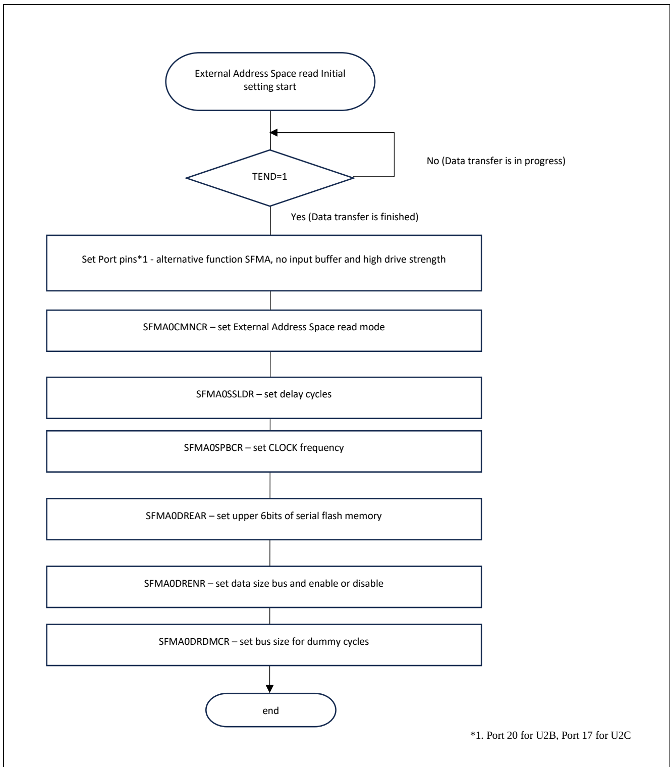
Figure 8 External address space initial setting flow
