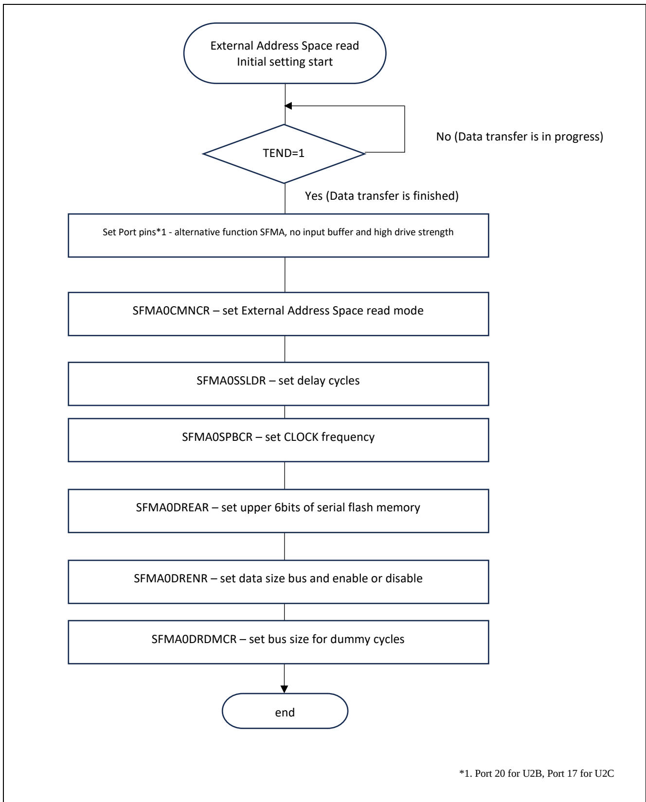
Figure 4 SPI initial setting flow
