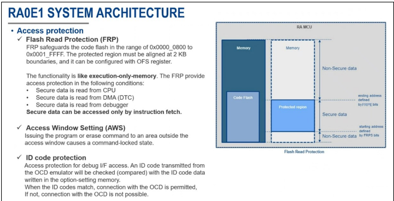
Figure 5 RA0E1 Access Protection
