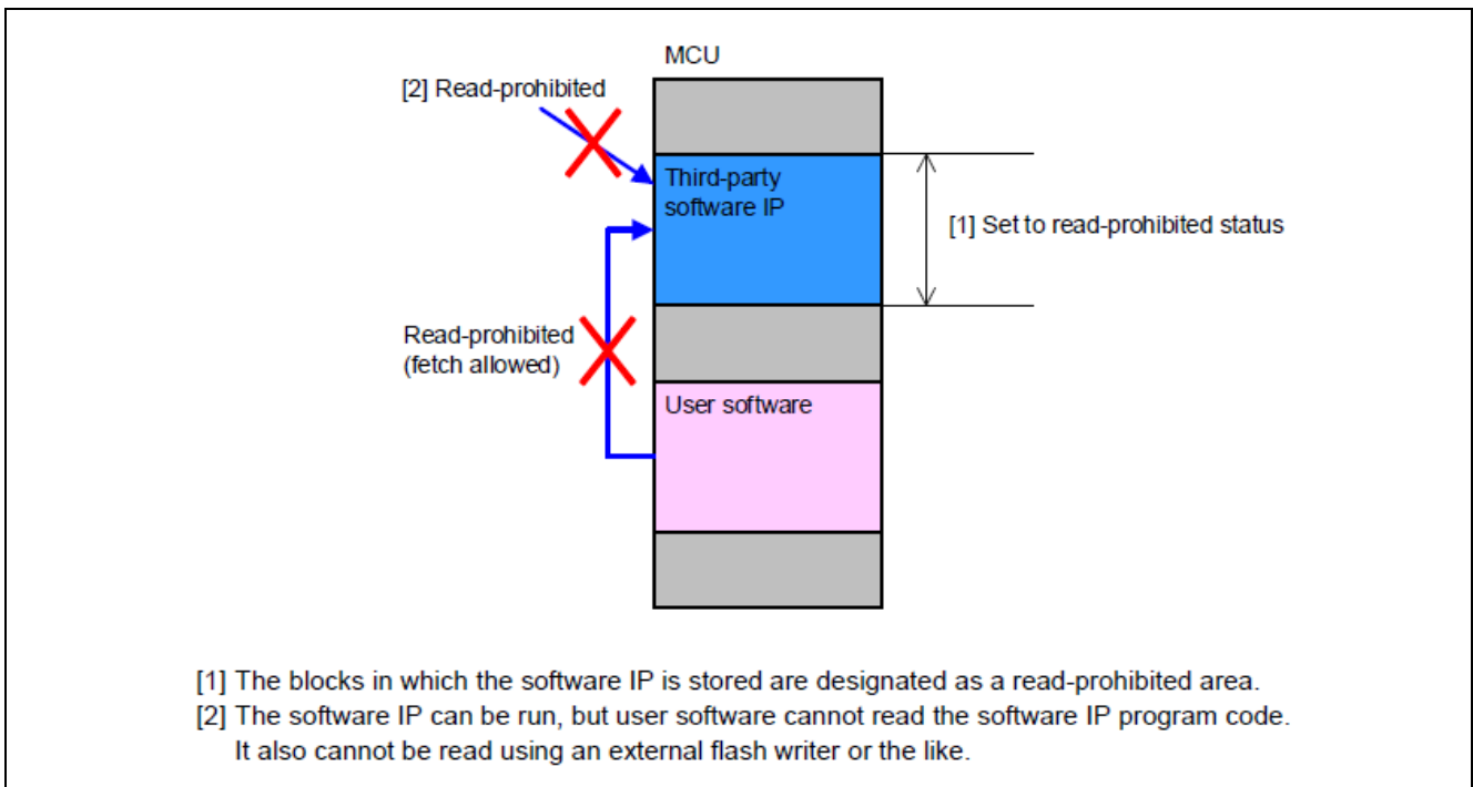
Figure 1 Flash Read Protection
