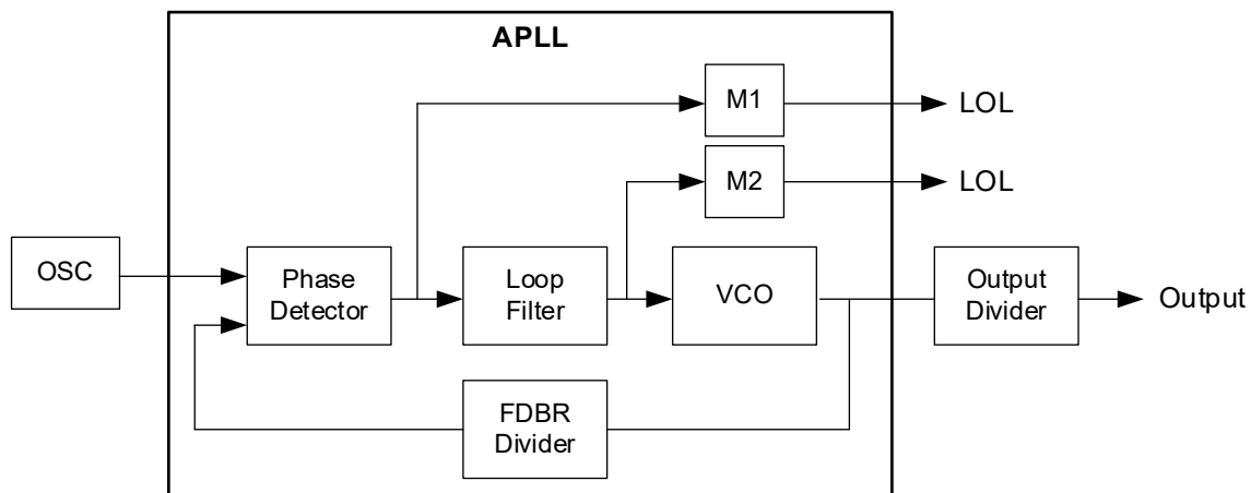
Figure 5. APLL LOL
