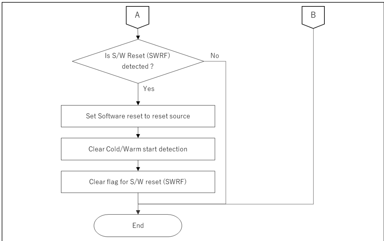
Figure 4-8 R_BSP_WarmStart () (4/4)
