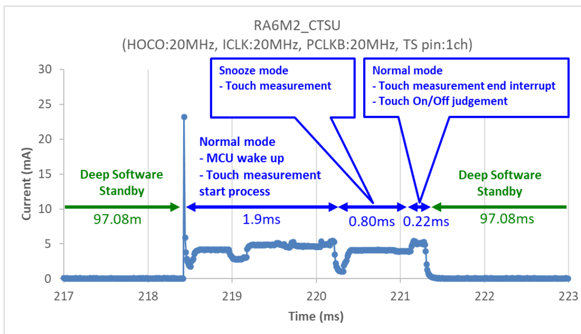
Figure 5-6 Current consumption waveform (2/2)
