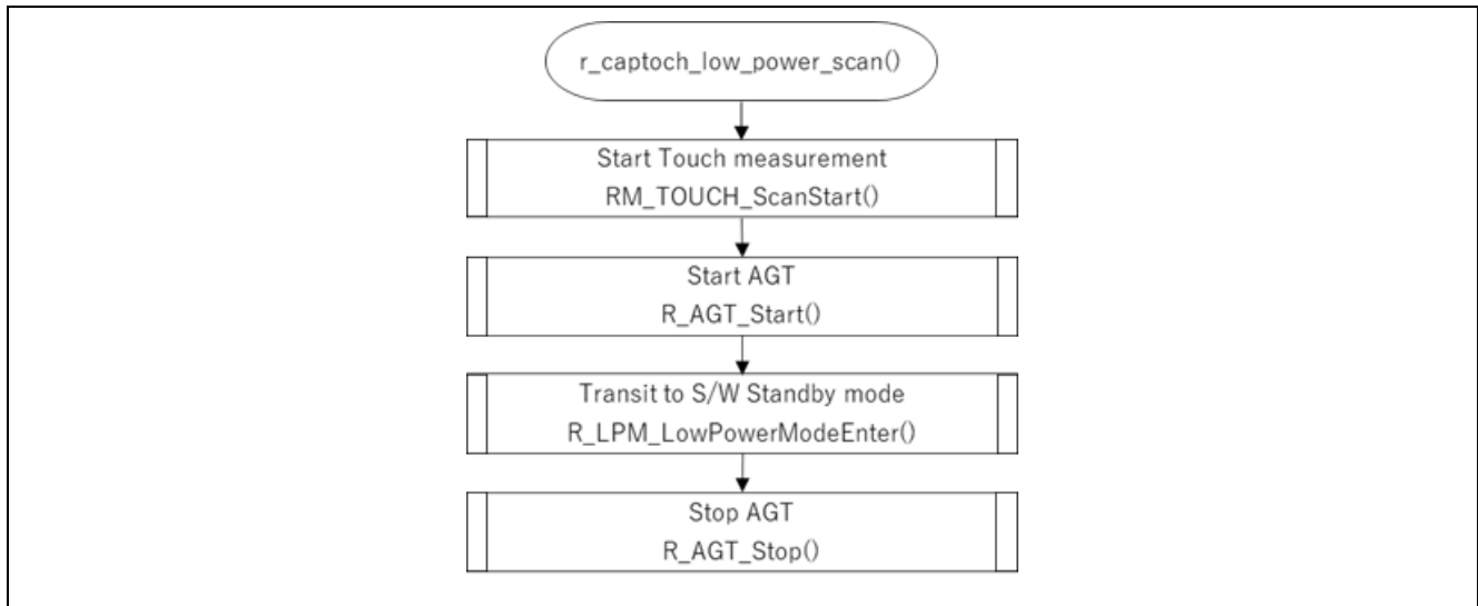
Figure 4-3 r_captouch_low_power_scan ()
