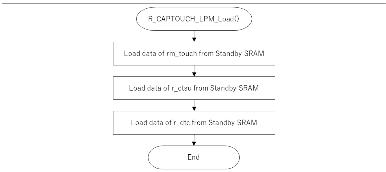
Figure 4-10 R_CAPTOUCH_LPM_Load ()
