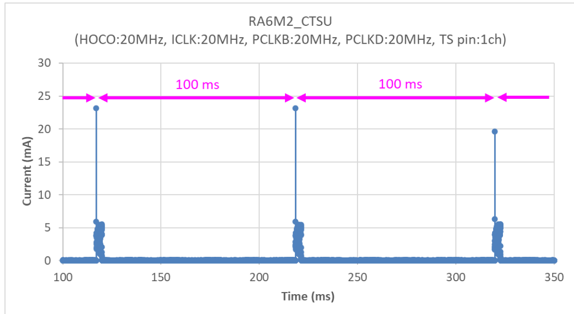
Figure 5-5 Current consumption waveform (1/2)
