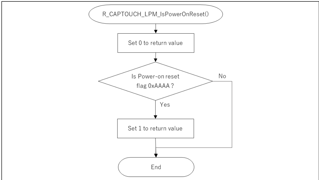
Figure 4-11 R_CAPTOUCH_LPM_IsPowerOnReset ()
