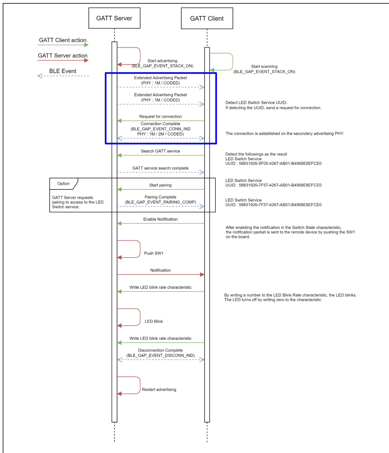
Figure 1. Message sequence chart of the demo project
