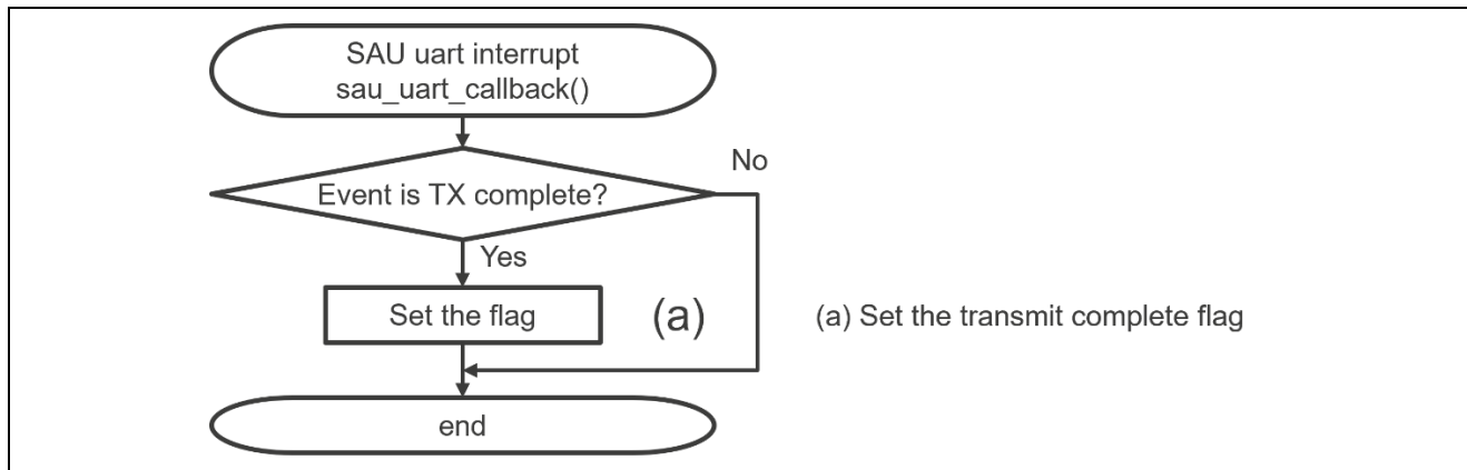
Figure 26 SAU Interrupt Processing
