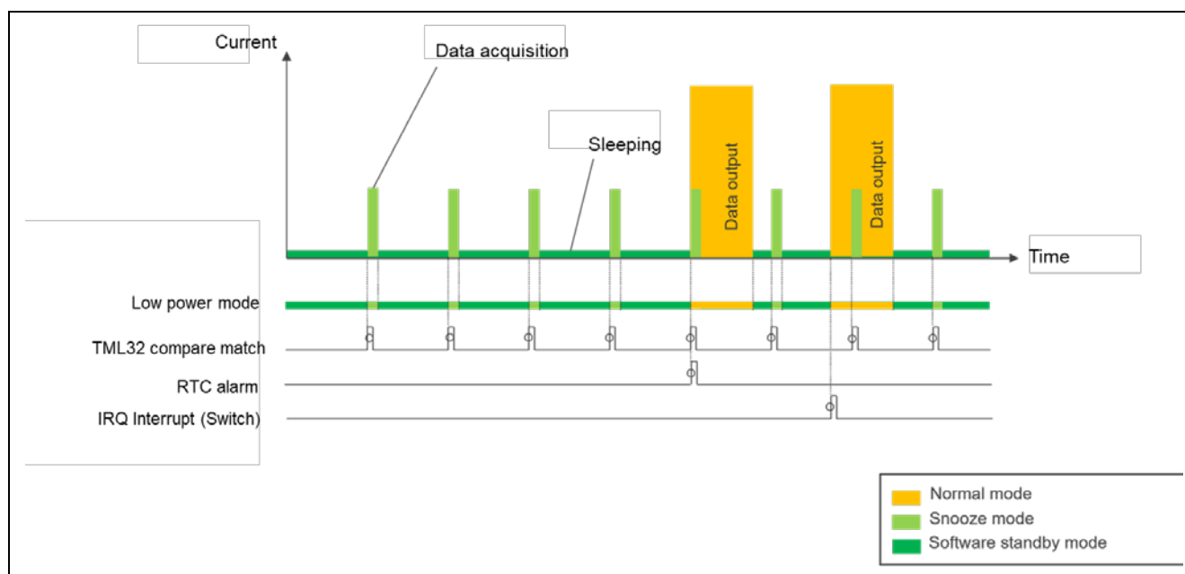
Figure 2 RA0E1 Conceptual Diagram of Operation Mode and Current Consumption
