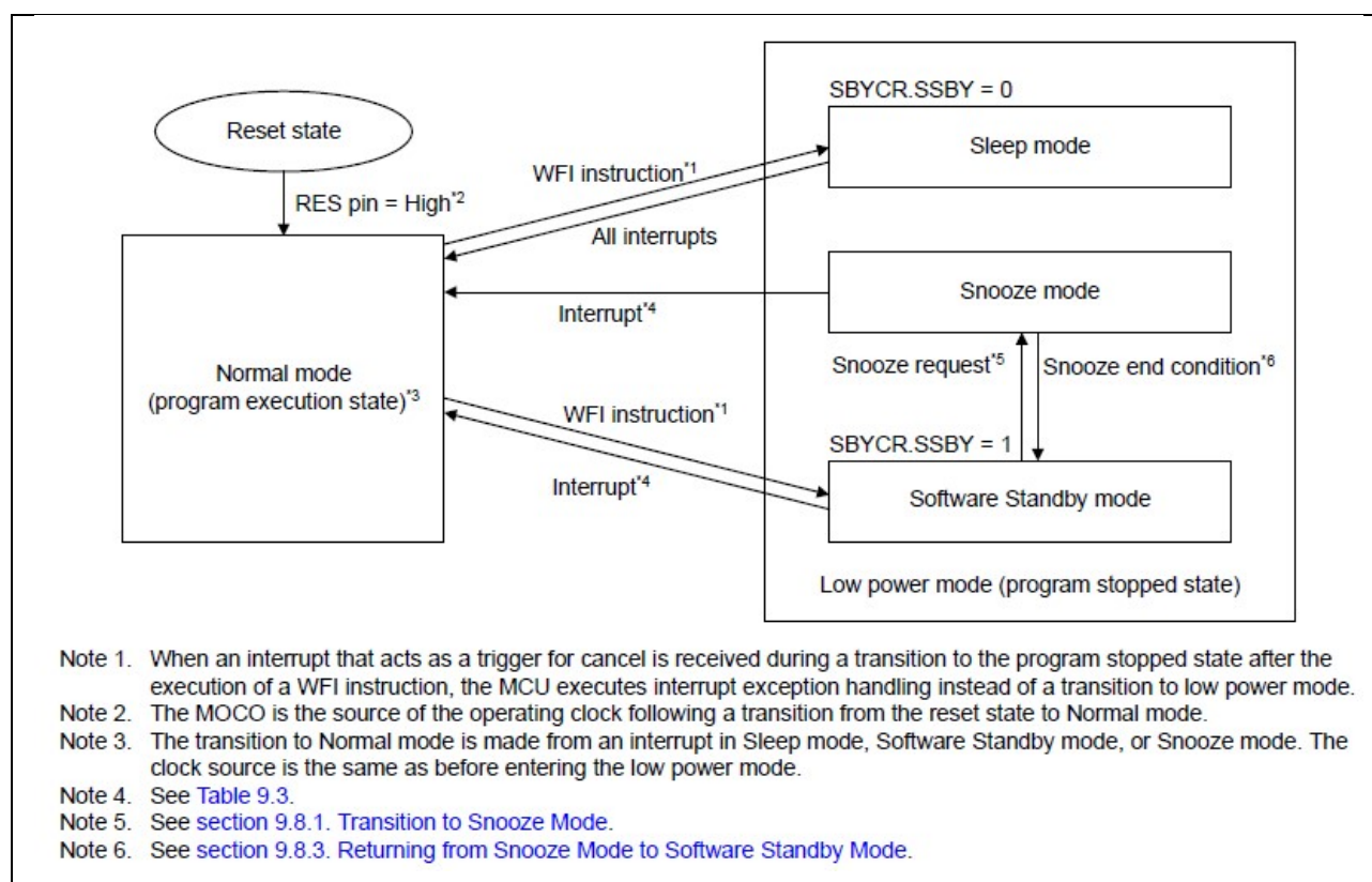
Figure 5 Schematic Diagram of Low Power Mode Transitions
