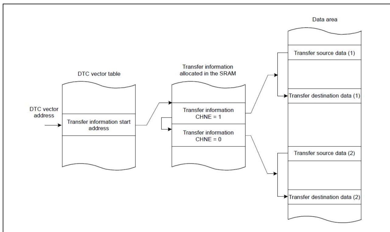
Figure 12 Chain Transfer Operation
