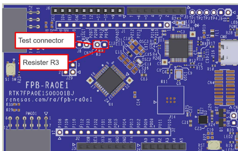
Figure 31 MCU Current Measuring Points
