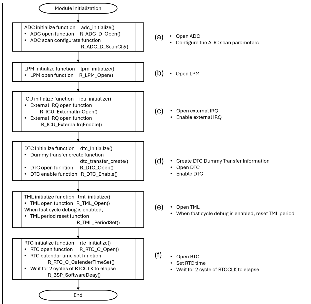
Figure 20 Module initialization Processing
