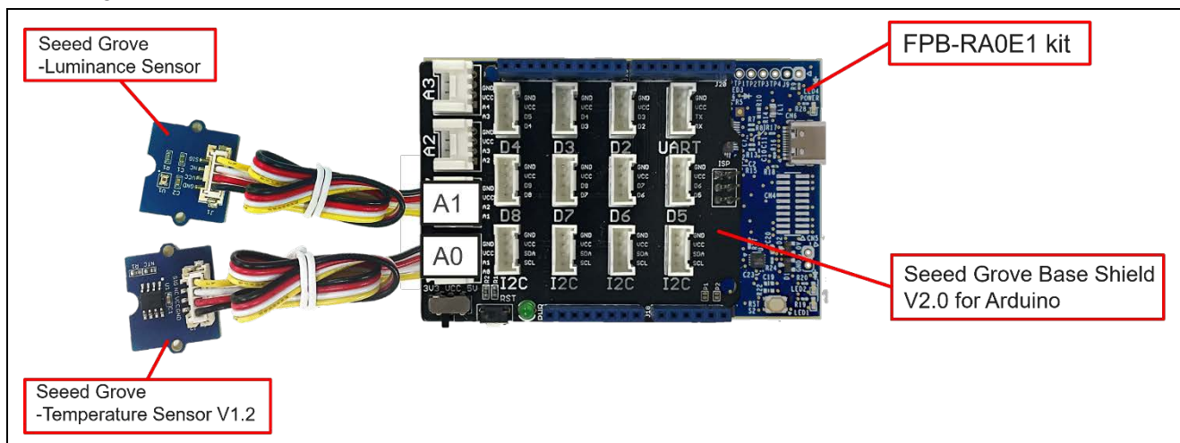
Figure 16 FPB-RA0E1 Sensor Connection
