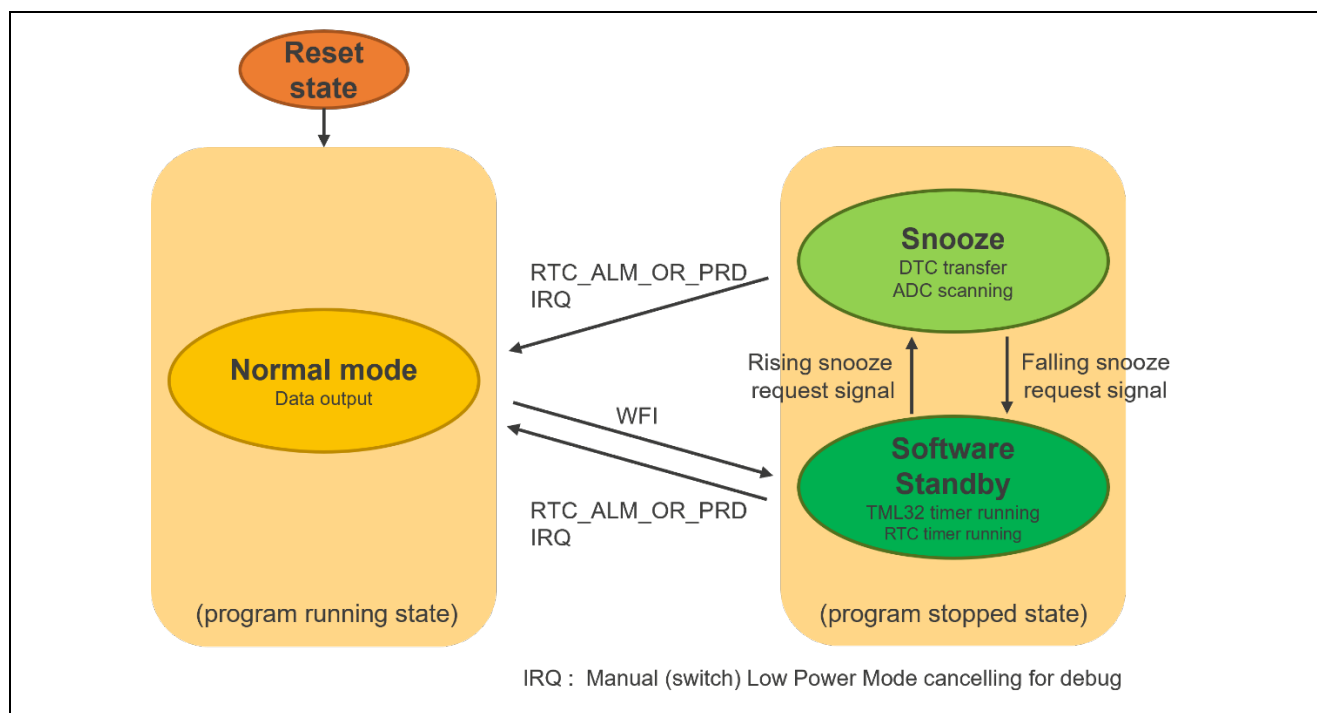
Figure 1 MCU Status and Mode Transition Events RA0E1
