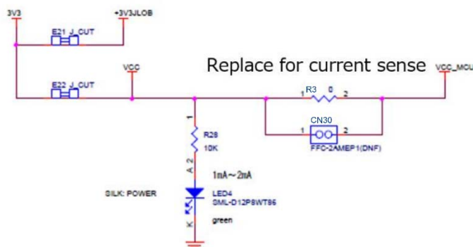
Figure 30 MCU Current Measuring Points (Circuit Diagram)
