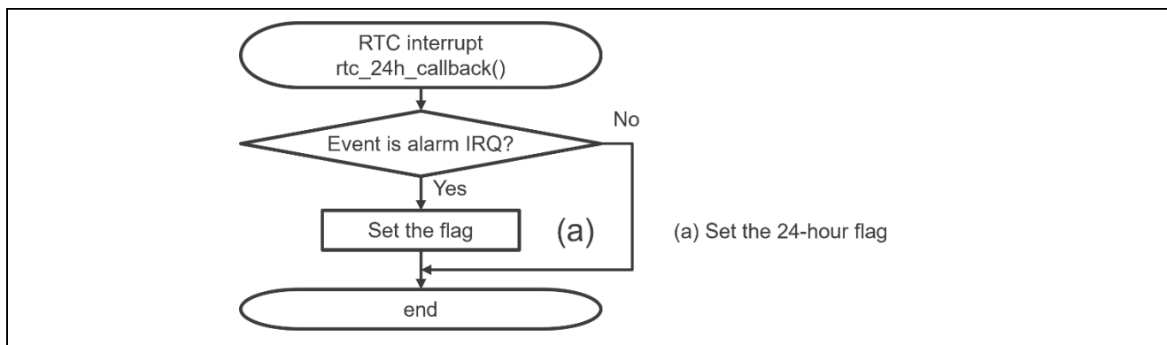
Figure 24 RTC Alarm Interrupt Processing
