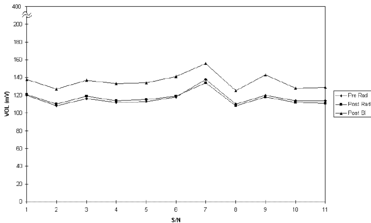
FIGURE 7. COMPARISON OF 64K PROM OUTPUT DRIVE VOLTAGE LOW ( V_{OL} )
