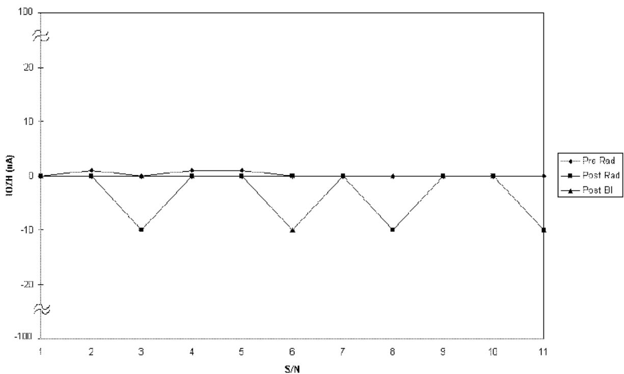
FIGURE 5. COMPARISON OF 64K PROM OUTPUT DRIVE CURRENT HIGH ( I_{OZH} )
