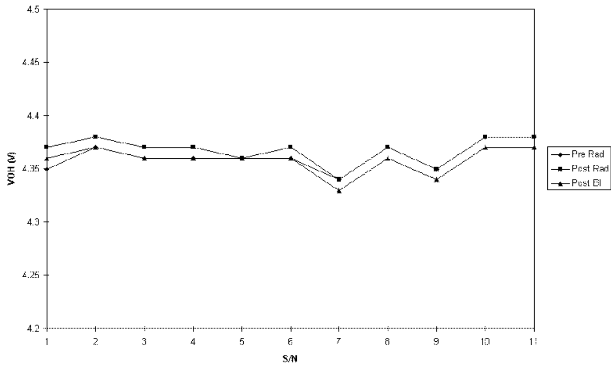
FIGURE 8. COMPARISON OF 64K PROM OUTPUT DRIVE VOLTAGE HIGH (VOH)
