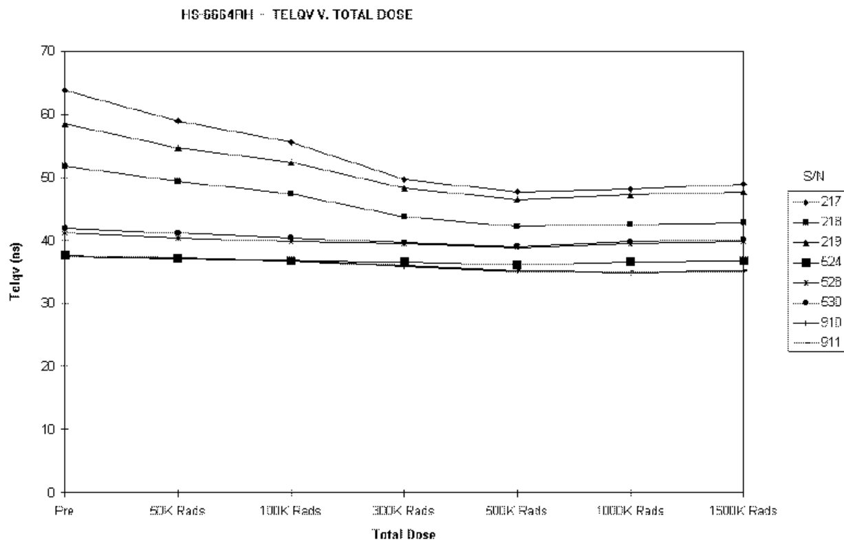
FIGURE 2. 64K PROM ACCESS TIME ( T_{ELQV} ) OVER TOTAL DOSE
