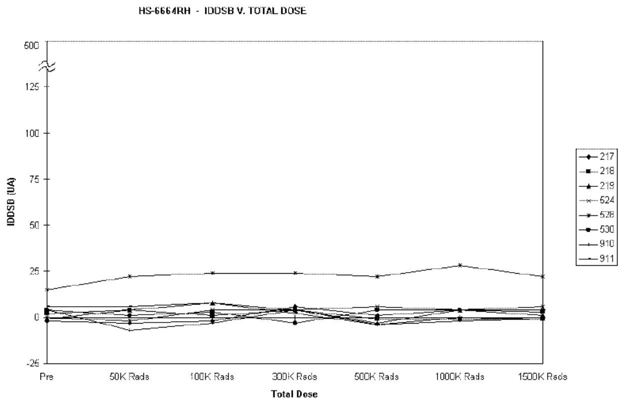
FIGURE 1. 64K PROM STANDBY CURRENT ( I_{DDSB} ) OVER TOTAL DOSE
