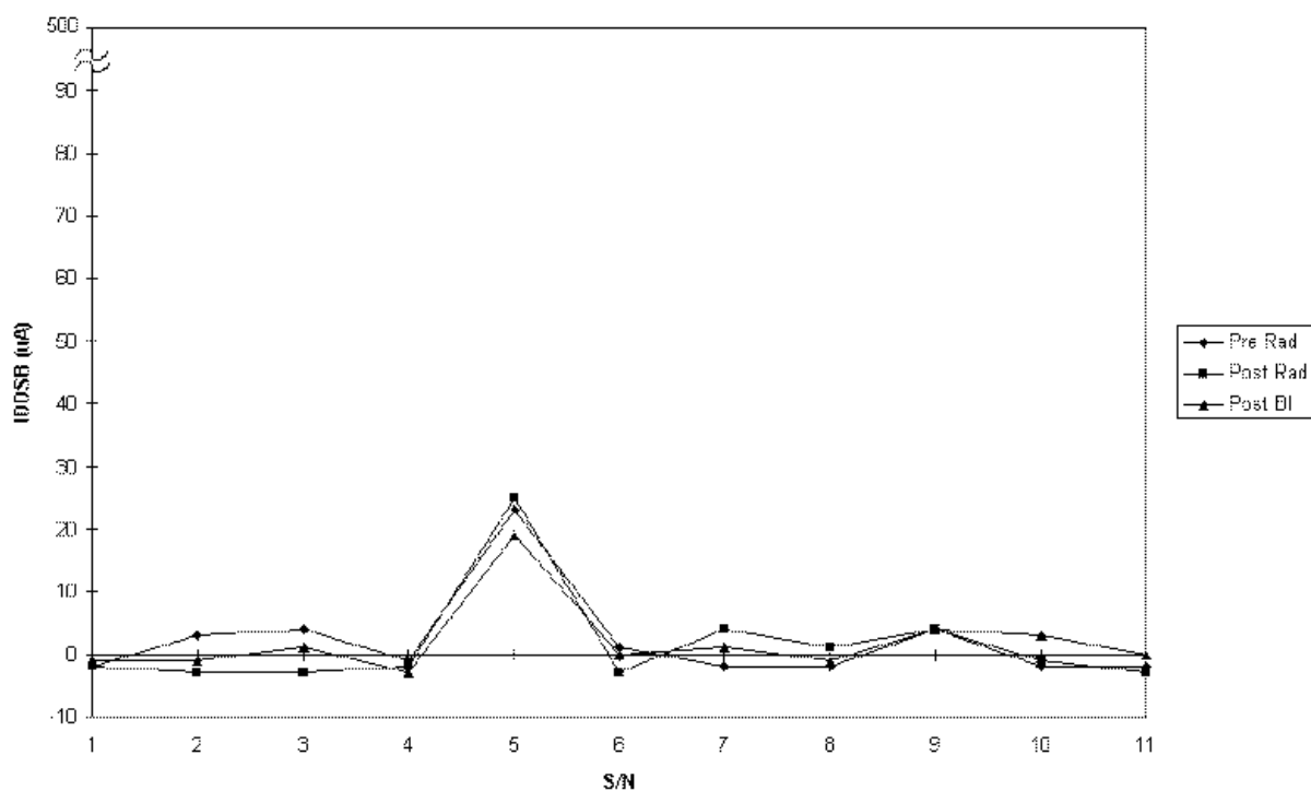
FIGURE 4. COMPARISON OF THE 64K PROM'S STANDBY CURRENT ( I_{DDSB} ) FROM PRE-RAD TO POST-RAD TO POST BURN-IN FOR 11 UNITS TESTED
