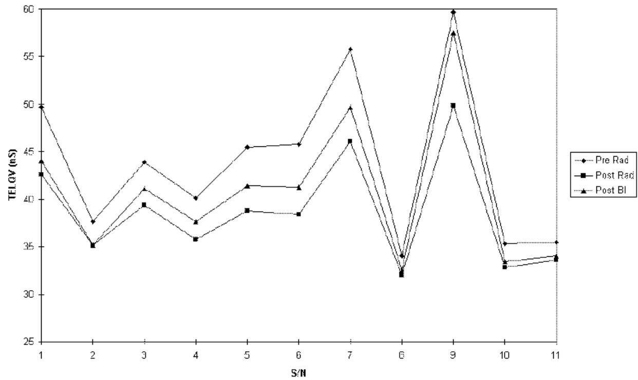
FIGURE 10. COMPARISON OF 64K PROM ACCESS TIME ( T_{ELQV} )
