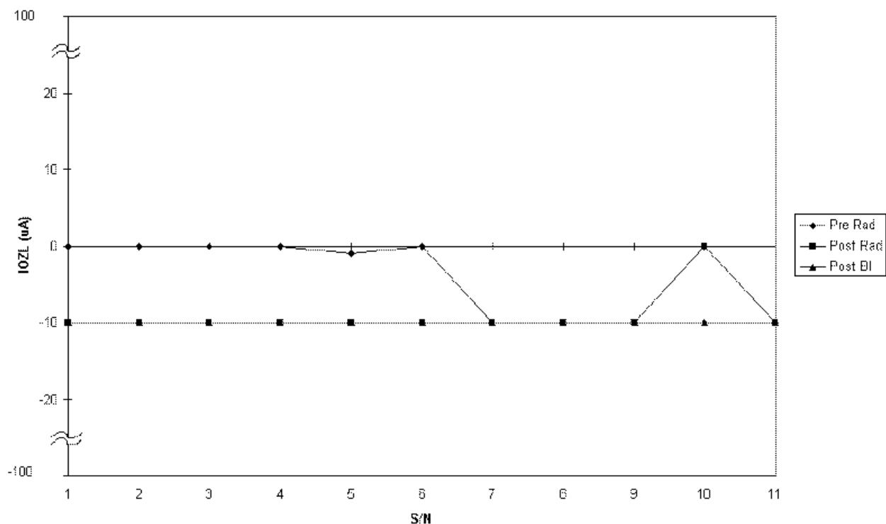
FIGURE 6. COMPARISON OF 64K PROM OUTPUT DRIVE CURRENT LOW ( I_{OZL} )
