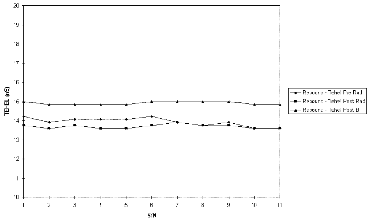
FIGURE 9. COMPARISON OF 64K PROM ENABLE HIGH TO ENABLE LOW TIME (TEHEL)
