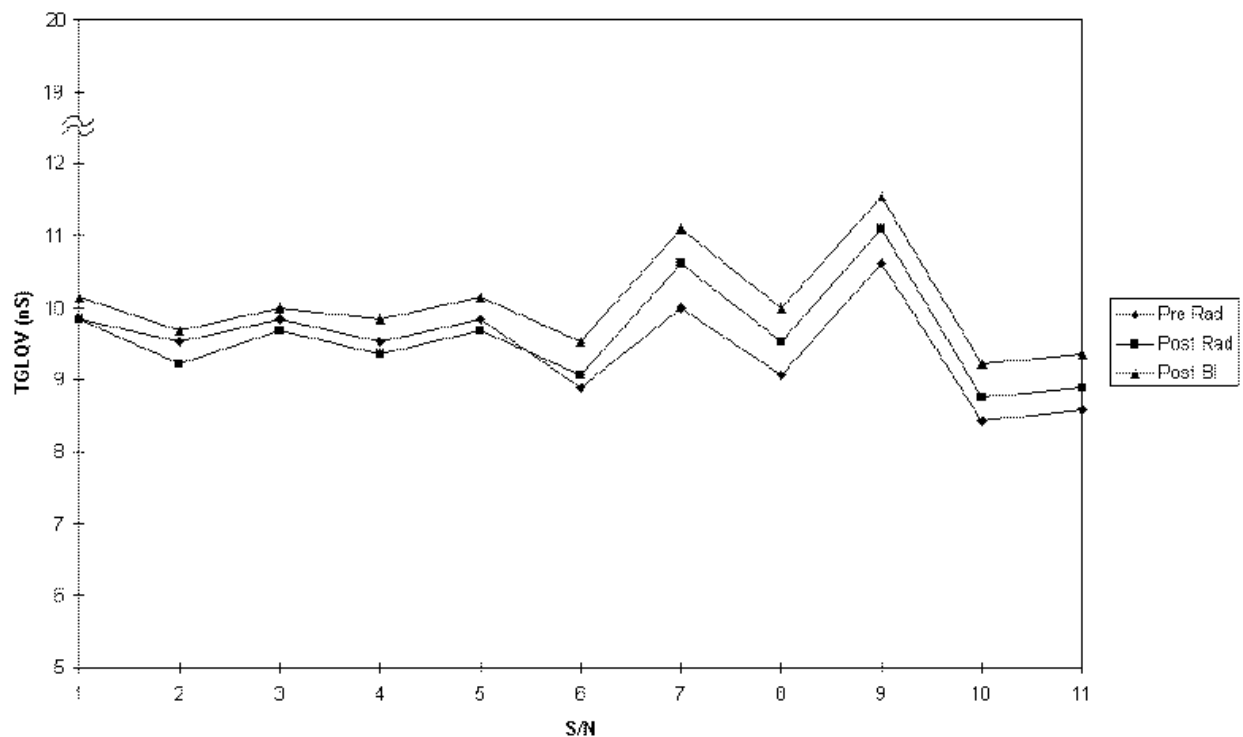
FIGURE 11. COMPARISON OF 64K PROM OUTPUT ENABLE TO OUTPUT VALID ( T_{GLQV} )
