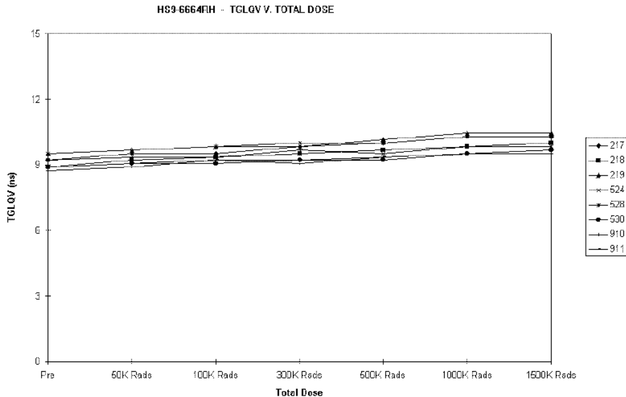
FIGURE 3. 64K PROM OUTPUT ENABLE TIME ( T_{GLQV} ) OVER TOTAL DOSE
