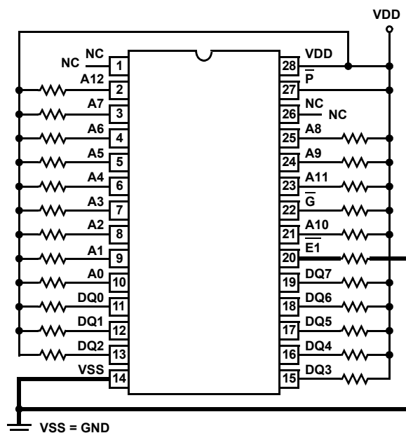
FIGURE 12. IRRADIATION CONFIGURATION HS1-6664RH (8K x 8 PROM DIP)
