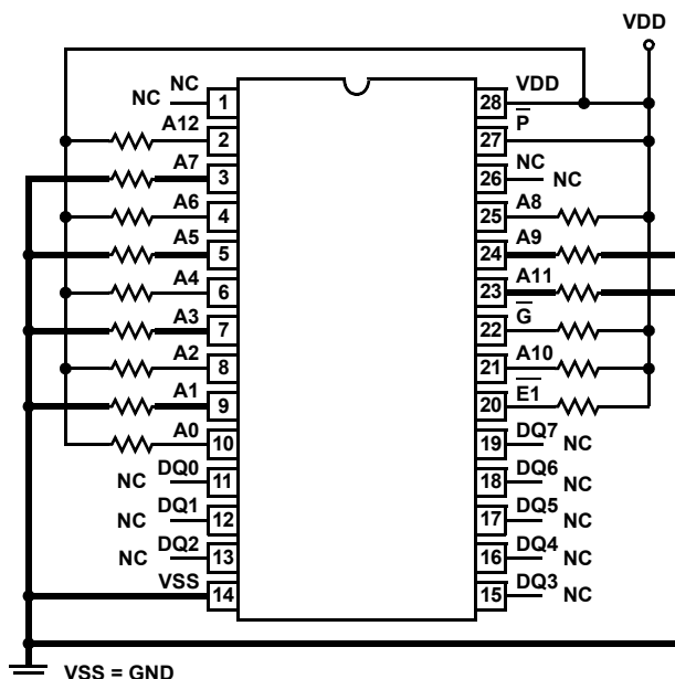
FIGURE 13. STATIC BURN-IN CONFIGURATION HS1-6664RH (8K x 8 PROM DIP), HS9-6664RH (8K X 8 PROM FLATPACK)
