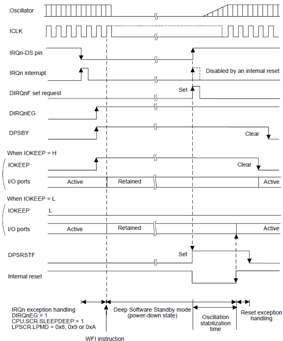
Figure 8. RA8M1 Deep Software Standby Entry and Exit Example
