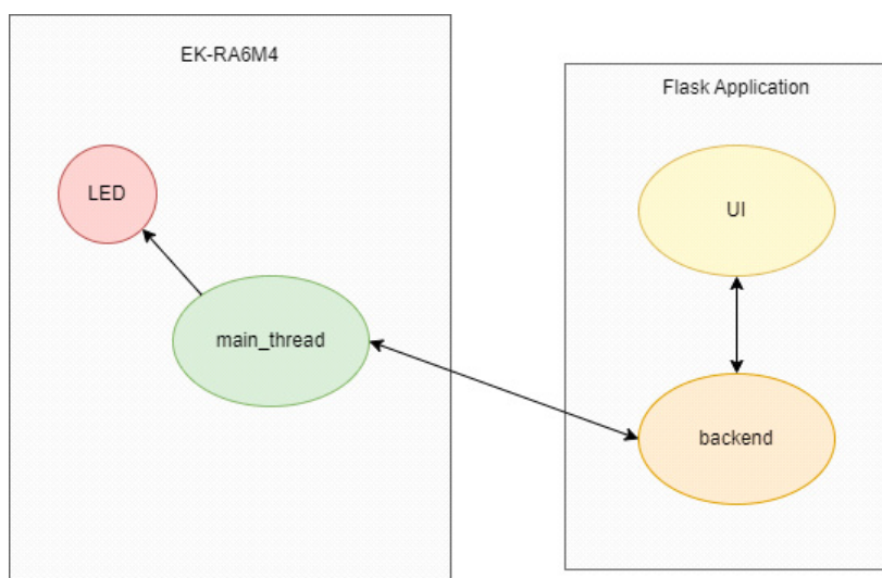
Figure 2. Architecture Diagram
