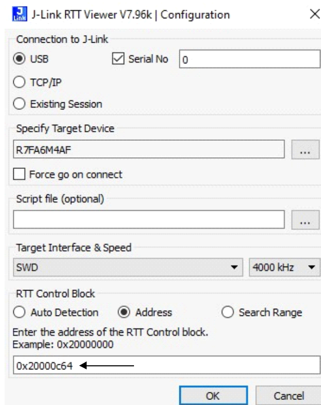
Figure 8. SEGGER RTT Configuration
