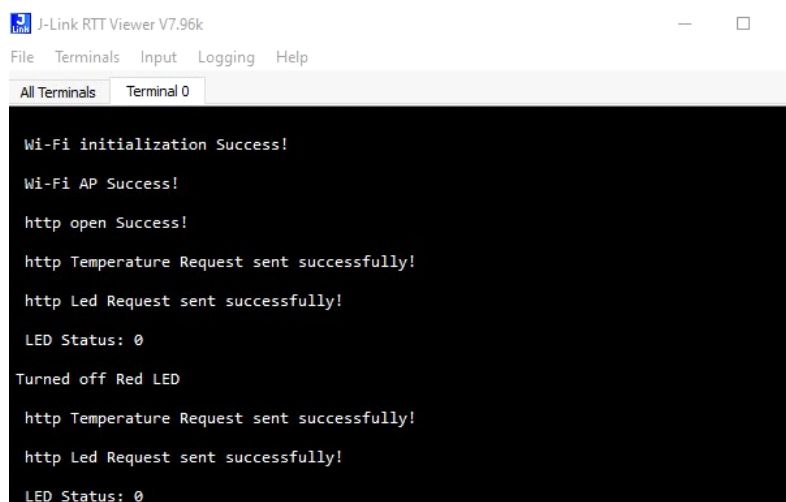
Figure 10. SEGGER RTT Logs
