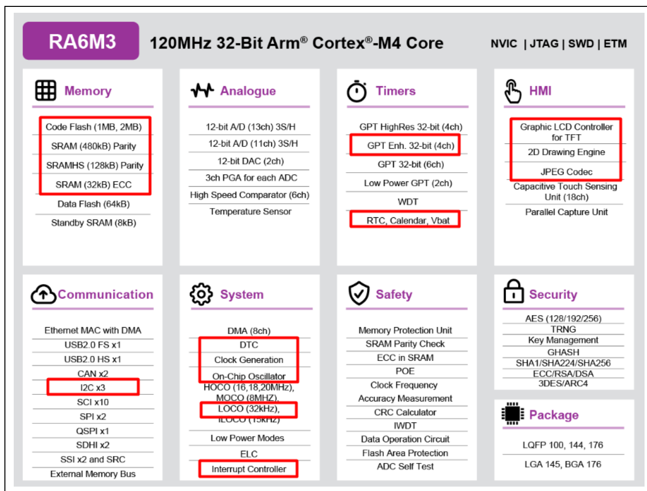
Figure 4. RA6M3 MCU Peripherals Used in the Graphics Application
