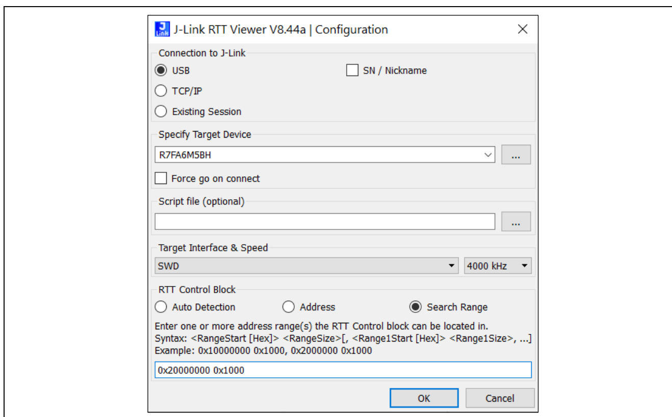
Figure 39. Configure SEGGER RTT Viewer
