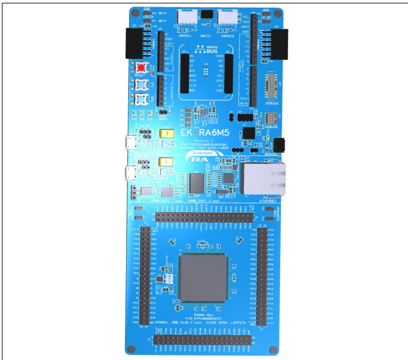
Figure 27. EK-RA6M5 Kit
