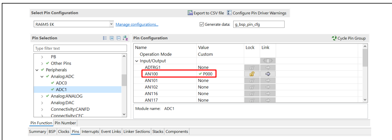
Figure 16. Configure P000 as AN100
