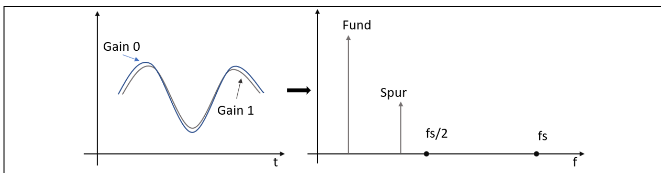
Figure 5. Sampled Data with Gain Mismatch
