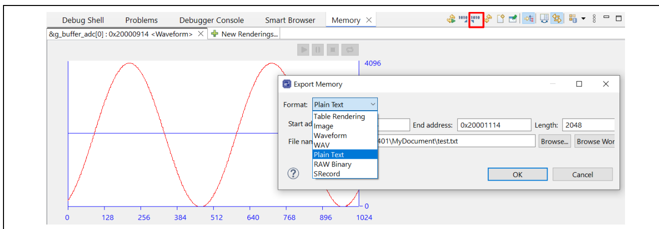
Figure 38. Select Data Format to Export Rendering Data
