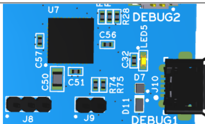
Figure 26. J8 and J9 on EK-RA6M5
