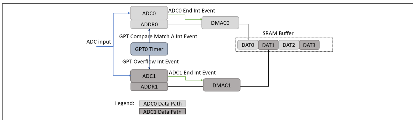
Figure 7. Block Diagram
