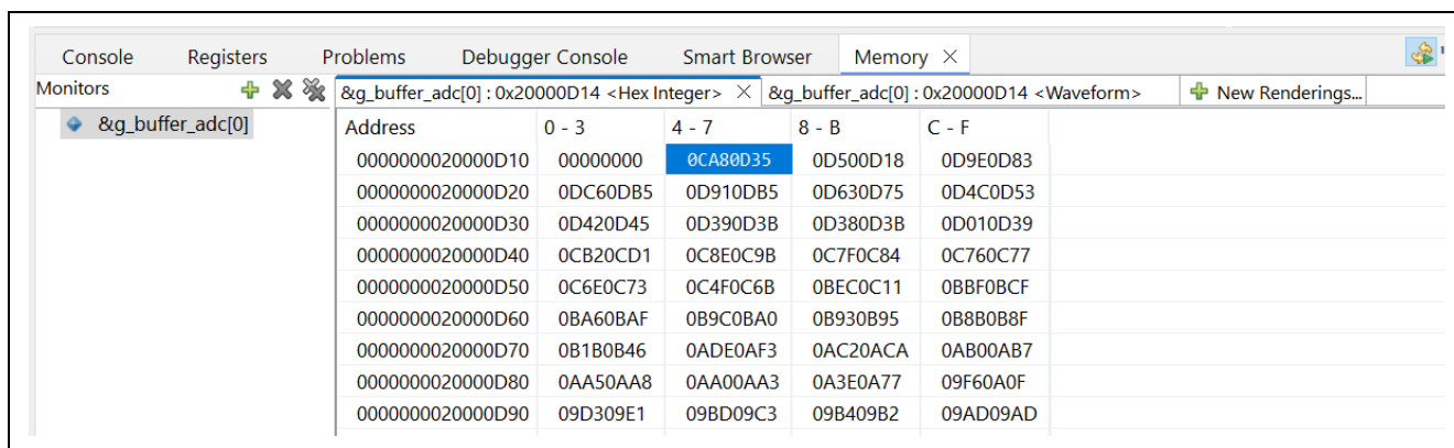
Figure 29. ADC Buffer in Hexadecimal
