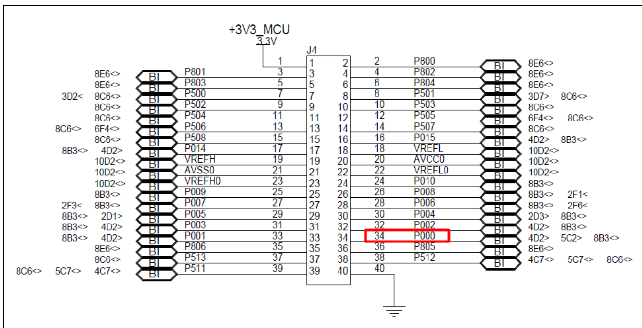
Figure 14. ADC Input Pin
