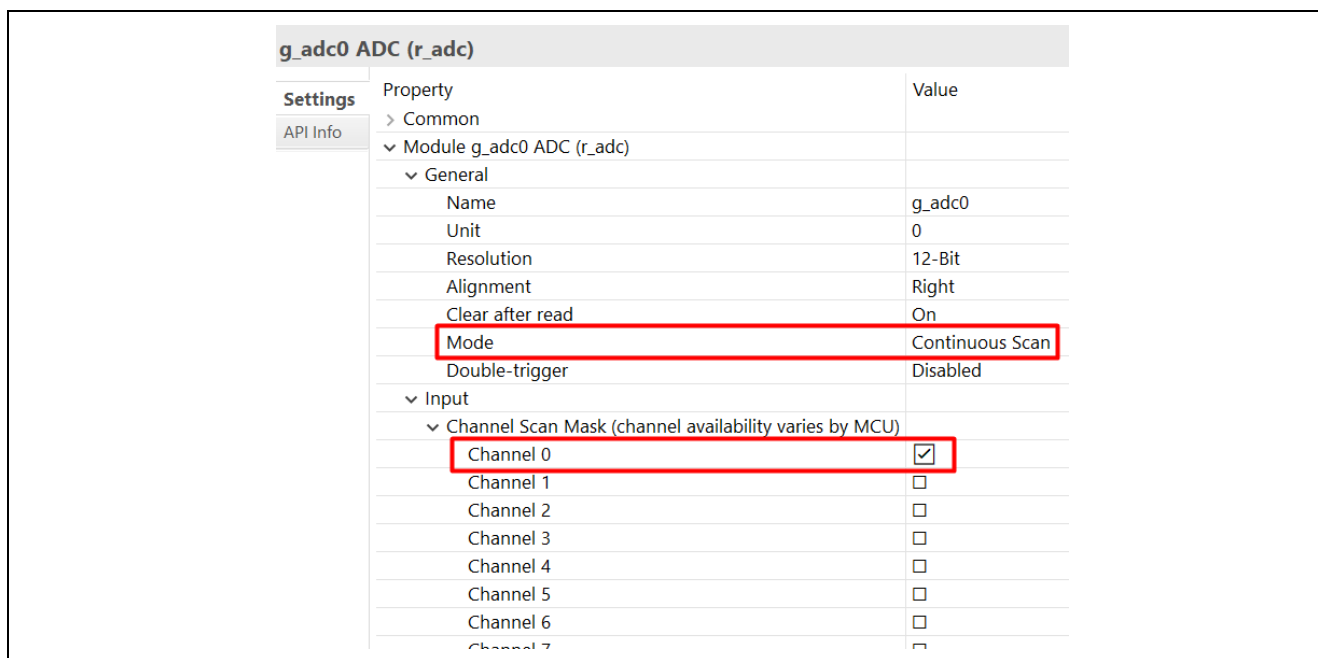
Figure 18. Configure ADC0 in Continuous Scan Mode, Channel 0 as Input
