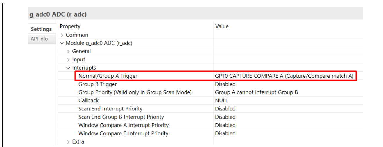
Figure 19. Set Trigger to Start ADC0 Conversion
