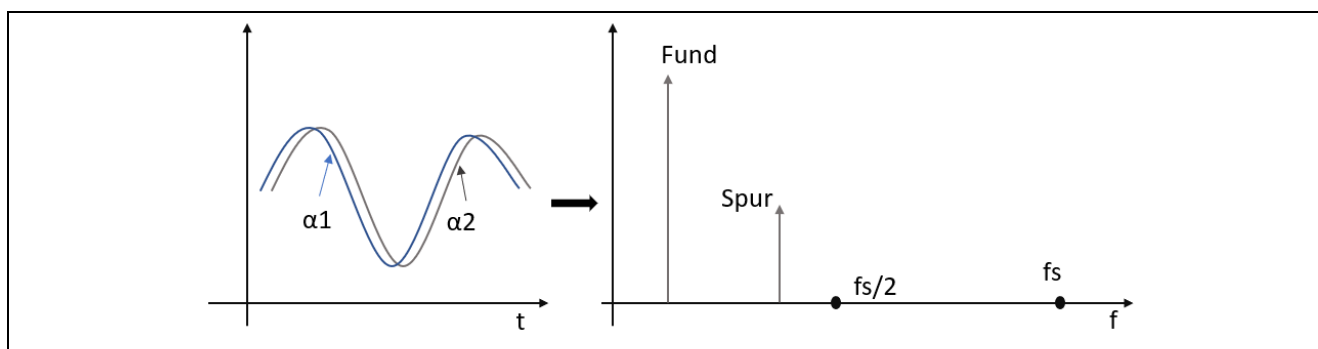
Figure 2. Sampled Data Spectrum due to Timing Error
