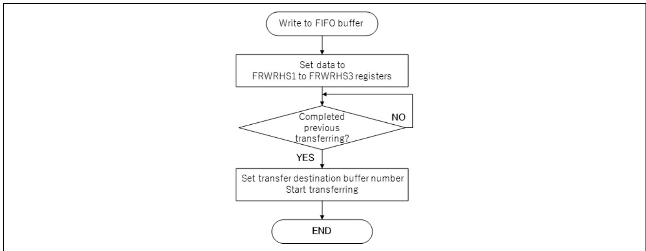
Figure 9-2 Control Setting Procedure
