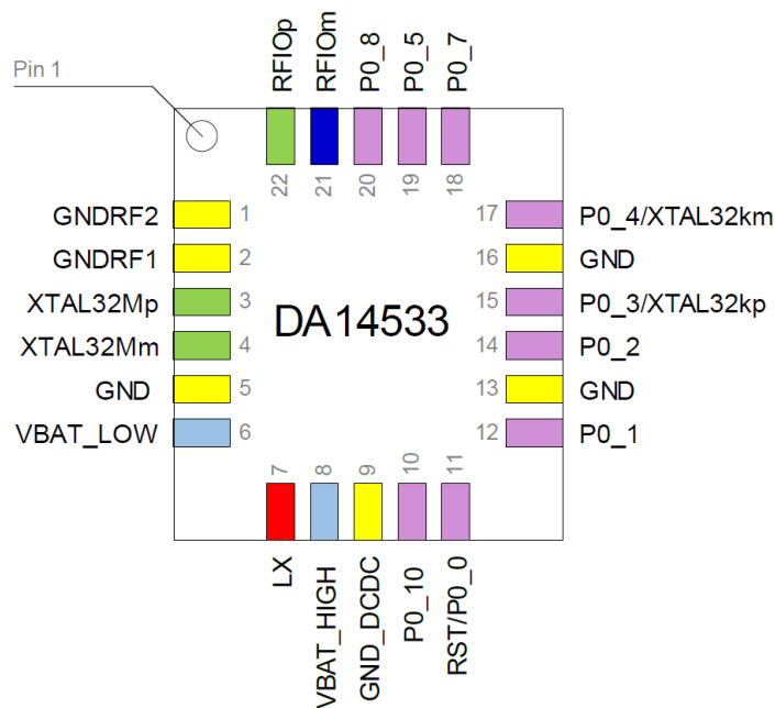
(Transparent top view) Figure 2. WFFCQFN22 pin assignment (top view)
