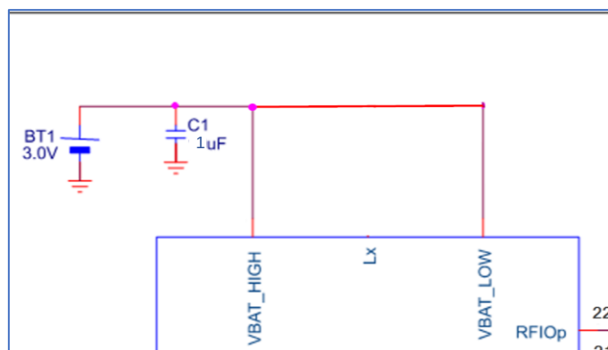
Figure 8. Bypass configuration
