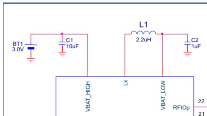
Figure 7. Buck configuration
