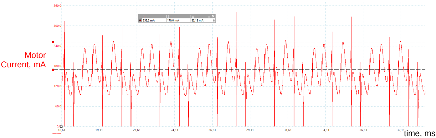
Figure 12: Motor No-Load Current, Power Supply 6.0 V
