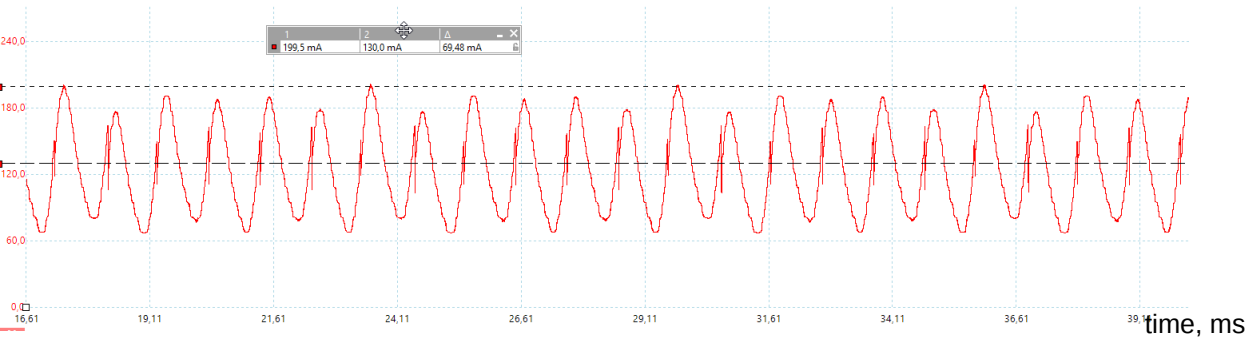
Figure 10: Motor No-Load Current, Power Supply 3.6 V
