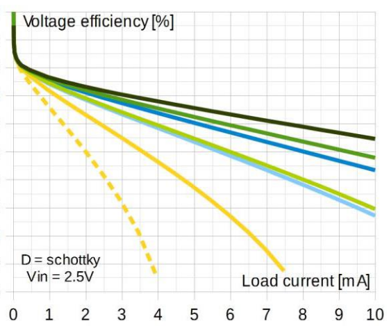
Figure 64: Voltage Efficiency 2.5 V Schottky
