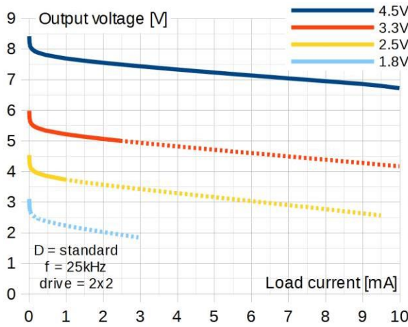
Figure 11: Output Voltage vs Load Silicon
