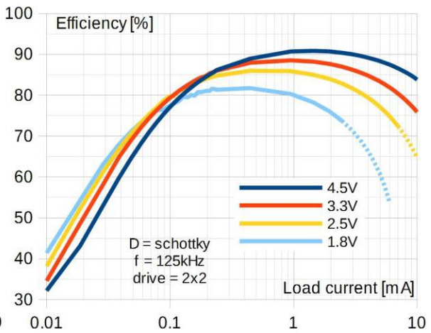
Figure 20: Efficiency vs Load Schottky SC:LG
