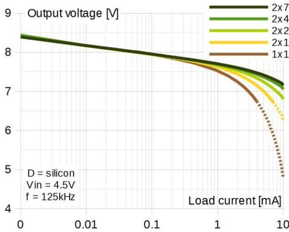
Figure 31: Load Regulation 5 V Silicon SC:LG
