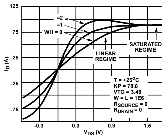
FIGURE 28. THE WH ADJUSTMENT
