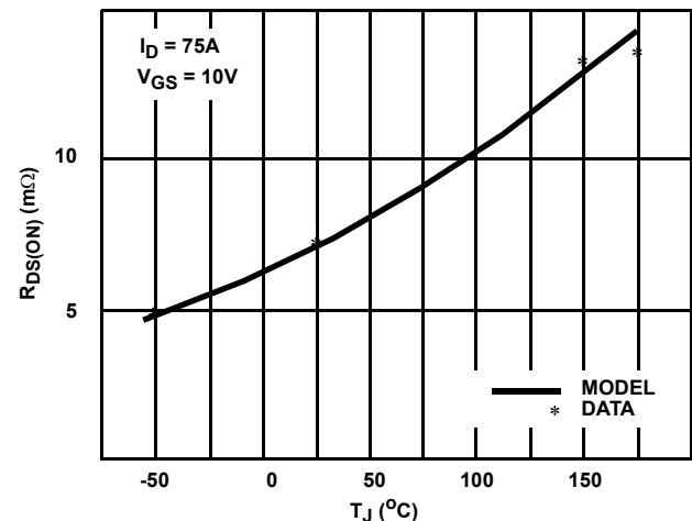
FIGURE 14. ON RESISTANCE vs TEMPERATURE
