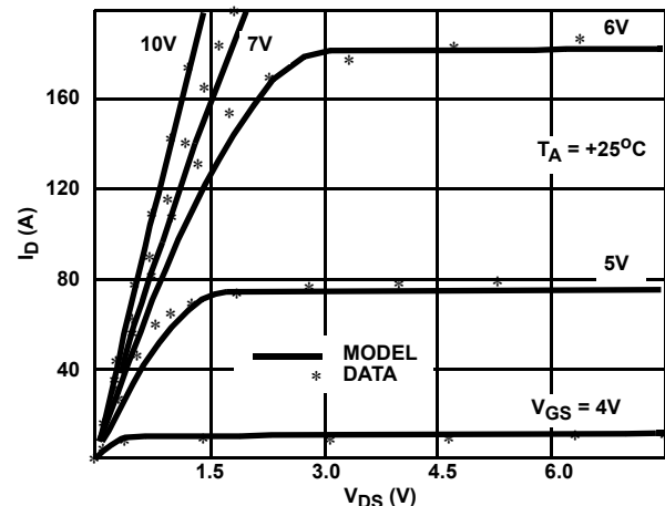
FIGURE 9. OUTPUT CURVES
