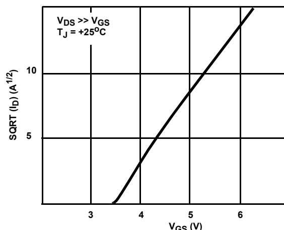
FIGURE 21. SQUARE ROOT OF I_D
