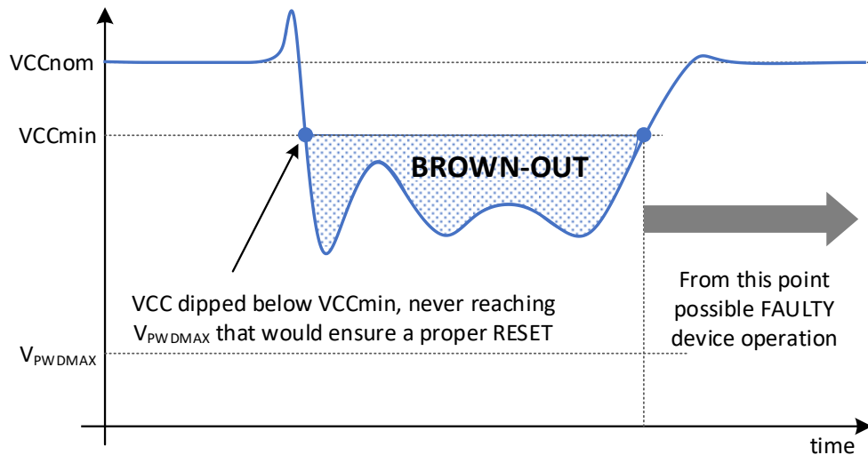
Figure 6: Brown-out Condition
