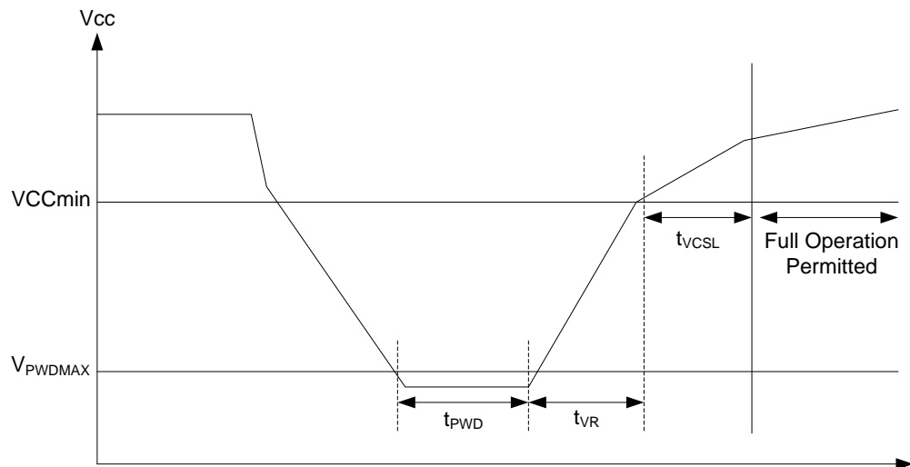
Figure 7: Recovery from Brown-Out Condition
