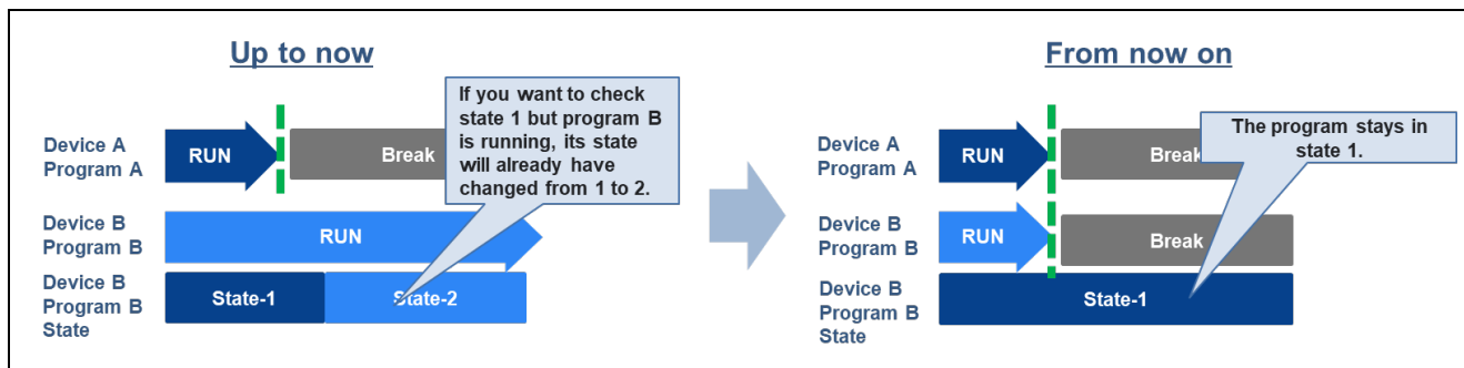
Figure 1-3 Synchronous Execution and Synchronous Break
