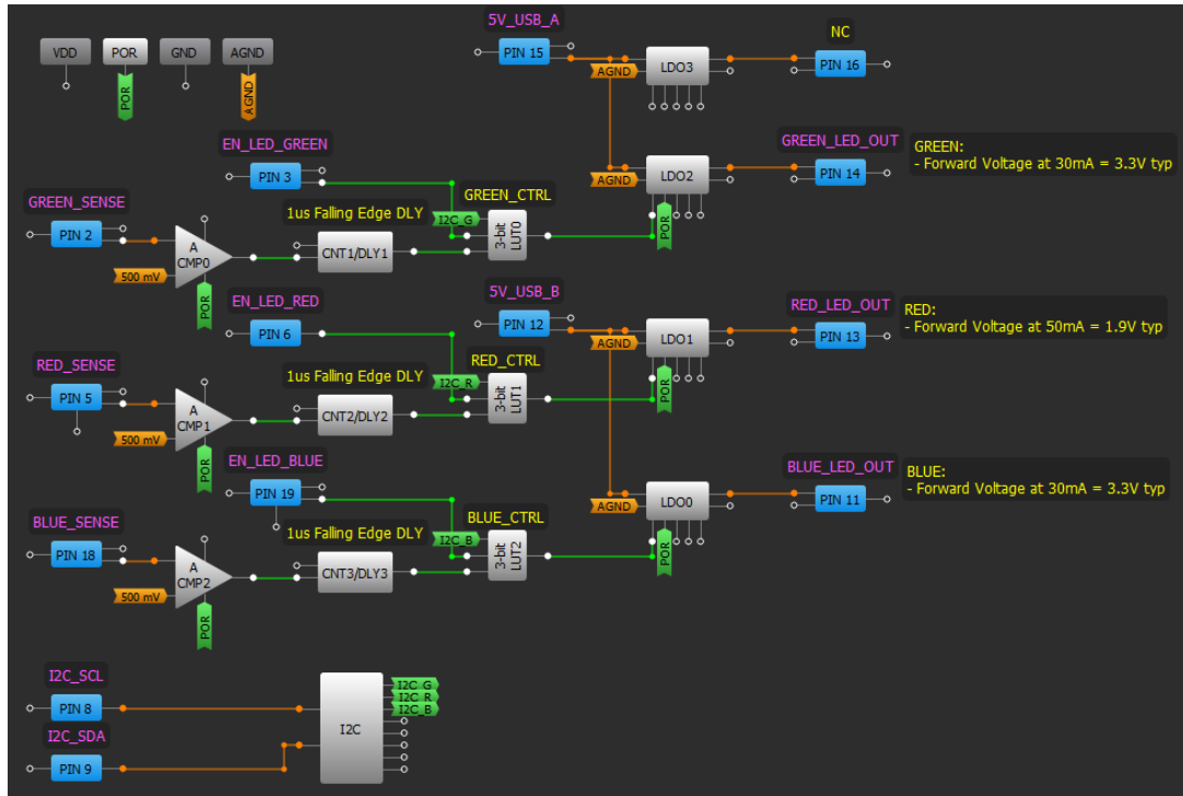
Figure 3: GreenPAK Constant brightness RGB Driver Design
