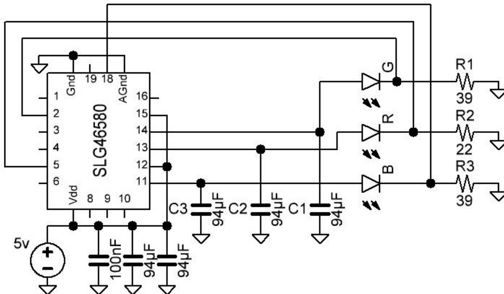
Figure 1: Constant Brightness RGB Driver Circuit Schematic
