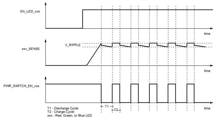
Figure 2: Constant brightness Functional Waveform
