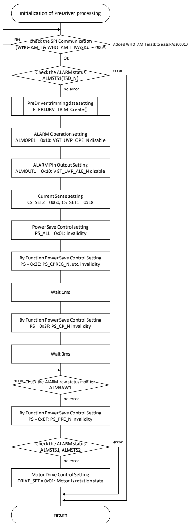
Figure 3-7 Flow chart (Initialization of PreDriver processing)
