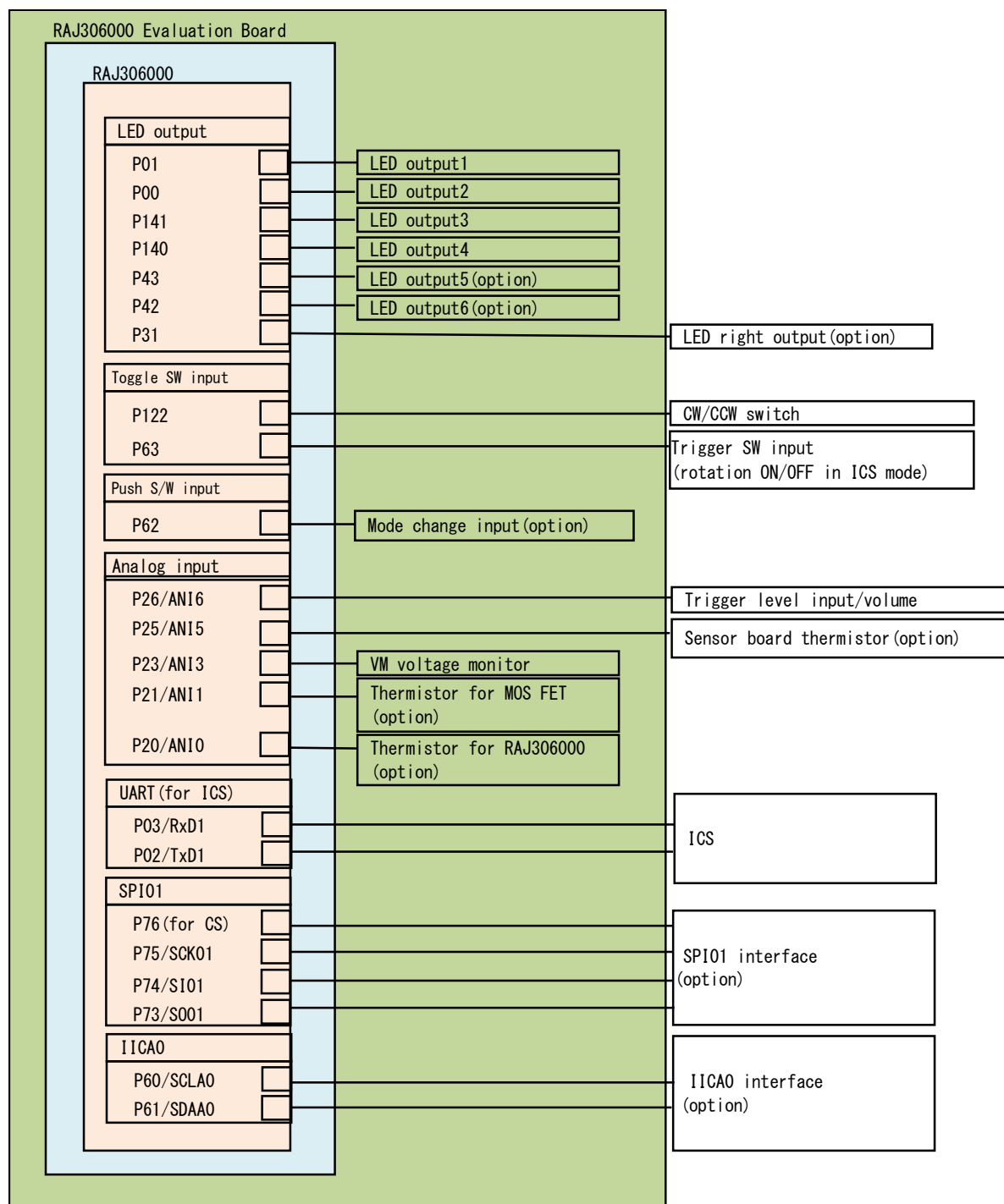
Figure 2-3 Hardware Configuration Diagram (RL78/G1F, Peripheral)
