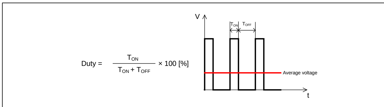
Figure 3-2 PWM control
