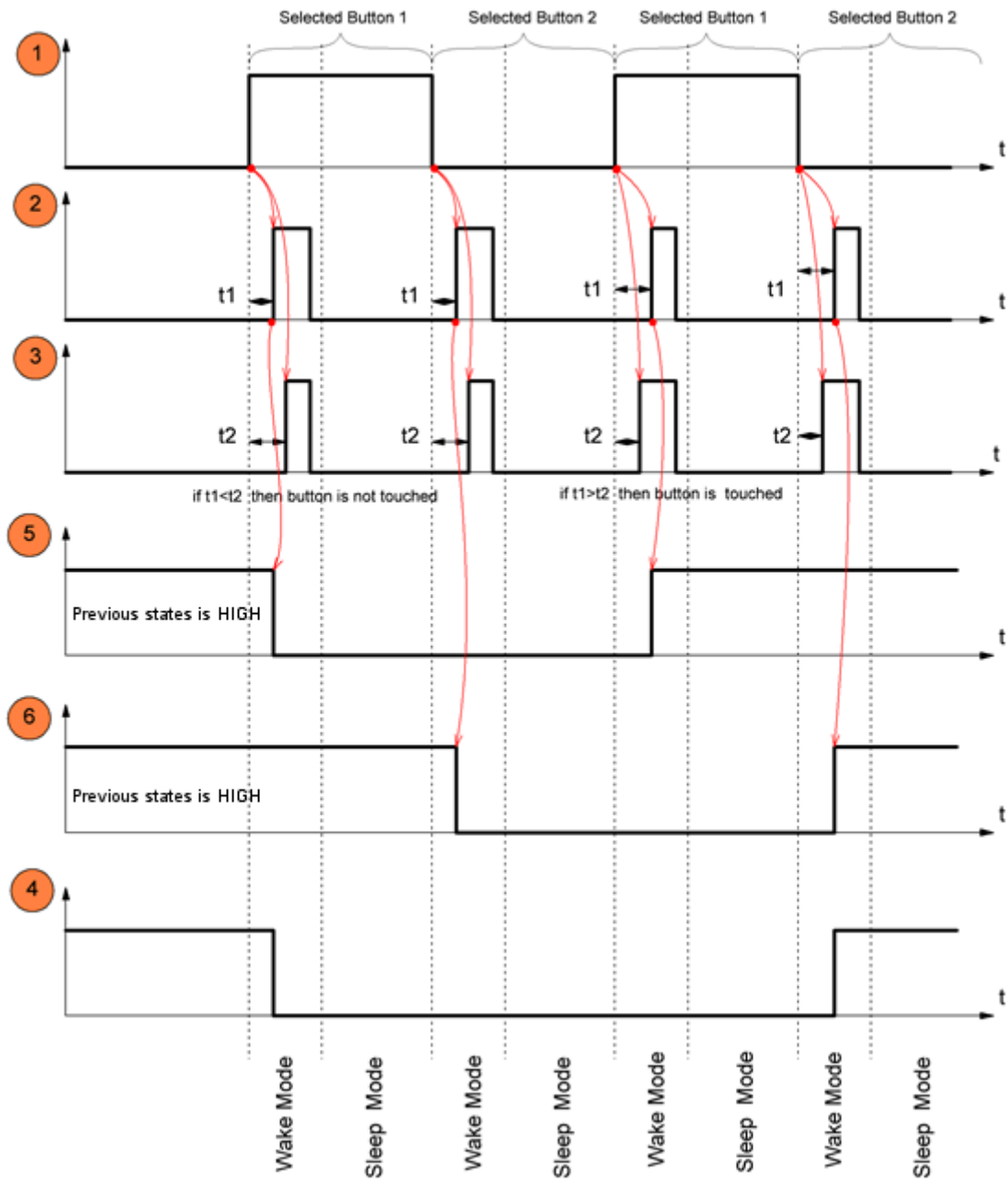
Figure 5. Touch sense timing diagram
