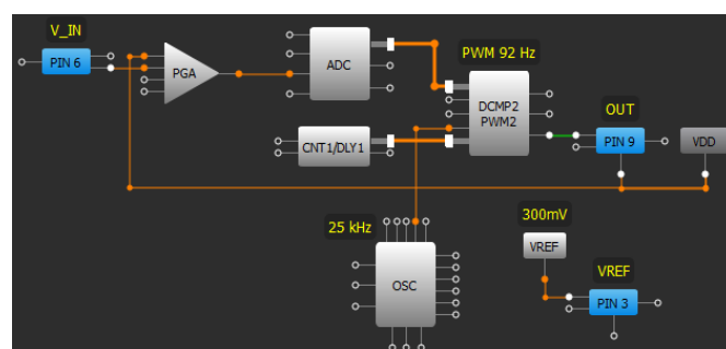
Fig. 3. Servo Control schematic
