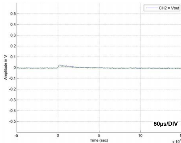
FIGURE 18. COMPOSITE PLOT OF THE 2 SET FOR DUT2 RUN 206: C_{OUT} = 1\mu\text{F} , C_{COMP} = 10\text{nF} , I_{OUT} = 10\text{mA} , V_{IN} = 30\text{V} , LET = 8.5
