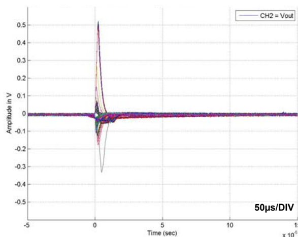
FIGURE 14. COMPOSITE PLOT OF 1021 SET FOR DUT1 RUN 303: C OUT = 0.1 \mu F, C COMP = 1nF, I OUT = -5mA, V IN = 30V, LET = 28
