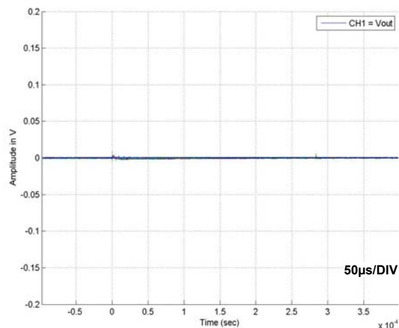
FIGURE 28. COMPOSITE PLOT OF 435 SET FROM RUN 313 DUT3: C_{OUT} = 10\mu F , C_{COMP} = 10nF , I_{OUT} = -5mA , V_{IN} = 30V , LET = 28
