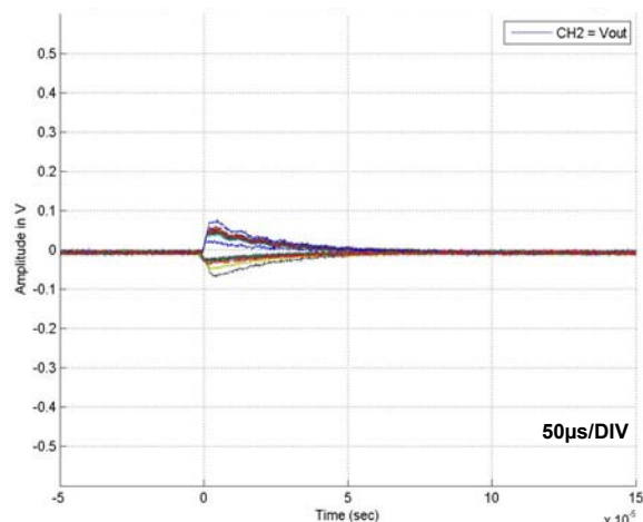
FIGURE 27. COMPOSITE PLOT OF 38 SET FROM RUN 313 DUT2: C_{OUT} = 1\mu F , C_{COMP} = 10nF , I_{OUT} = -5mA , V_{IN} = 30V , LET = 28 .
