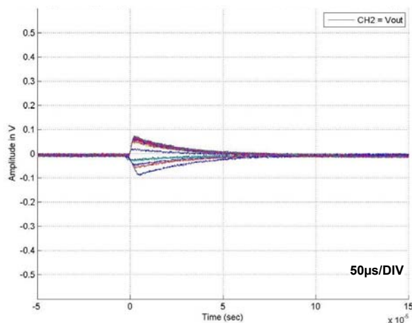
FIGURE 17. COMPOSITE PLOT OF 33 SET FOR DUT2 RUN 306: C_{OUT} = 1\mu\text{F} , C_{COMP} = 10\text{nF} , I_{OUT} = 10\text{mA} , V_{IN} = 30\text{V} , LET = 28
