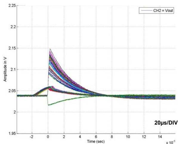
FIGURE 12. COMPOSITE (100) PLOT OF SET FOR ISL71091SEH20 AT LET = 28 V_{IN} = 16.5V , I_{OUT} = 1mA , C_{OUT} = 1\mu F , C_{COMP} = 1nF . TRIGGER AT \pm 20mV .
