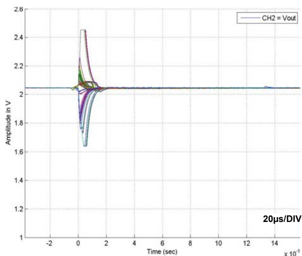
FIGURE 13. COMPOSITE PLOT OF 100 SET FOR ISL71091SEH20 at LET = 60, V_{IN} = 5.5V , I_{OUT} = 1mA , C_{OUT} = 0.1\mu F , C_{COMP} = 1nF . TRIGGER AT \pm 20mV AND SCOPE TRUNCATING SET AT \pm 400mV .
