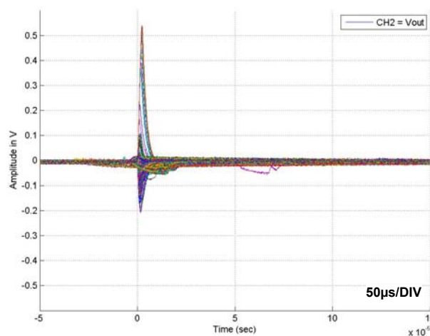
FIGURE 25. COMPOSITE PLOT OF 952 SET FROM RUN 313 ON DUT1: C_{OUT} = 0.1\mu\text{F} , C_{COMP} = 1\text{nF} , I_{OUT} = 10\text{mA} , V_{IN} = 30\text{V} , LET = 28
