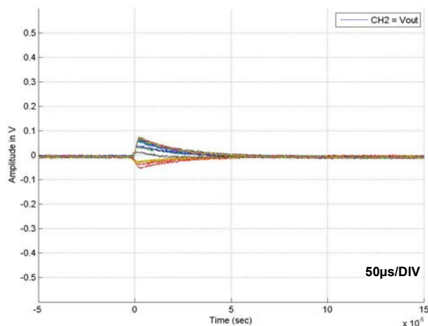
FIGURE 16. COMPOSITE PLOT OF 34 SET FOR DUT2 RUN 303: C_{OUT} = 1\mu\text{F} , C_{COMP} = 10\text{nF} , I_{OUT} = -5\text{mA} , V_{IN} = 30\text{V} , LET = 28
