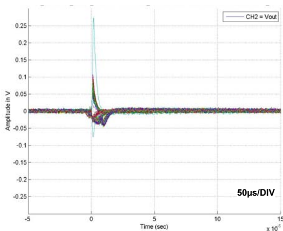
FIGURE 26. COMPOSITE PLOT OF 154 SET FROM RUN 213 DUT1: C_{OUT} = 0.1\mu F , C_{COMP} = 1nF , I_{OUT} = -5mA , V_{IN} = 30V , LET = 8.5 .
