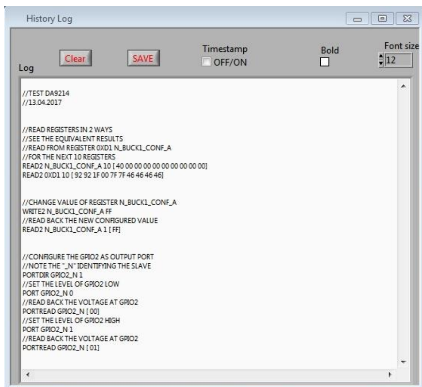
Figure 25: History Log
