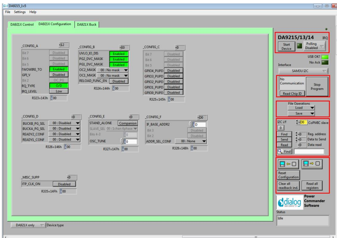
Figure 5: Initial Interface
