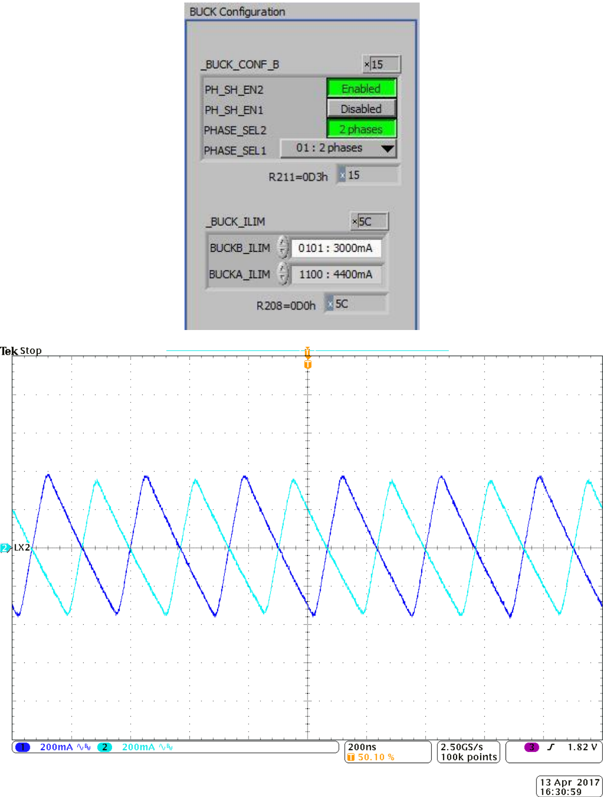
Figure 14: Inductor Current of Phase-1 and Phase-2, Phase-Shedding Disabled
