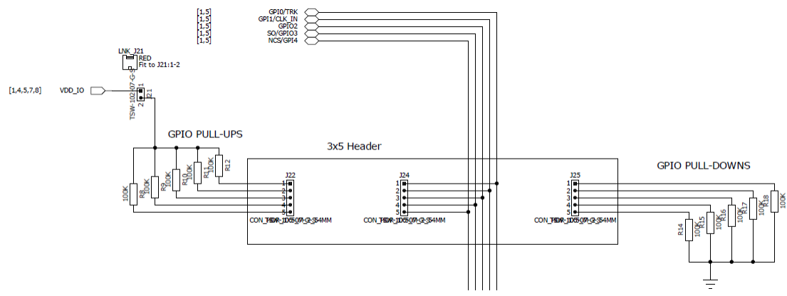
Figure 24: GPIOs Control Schematic
