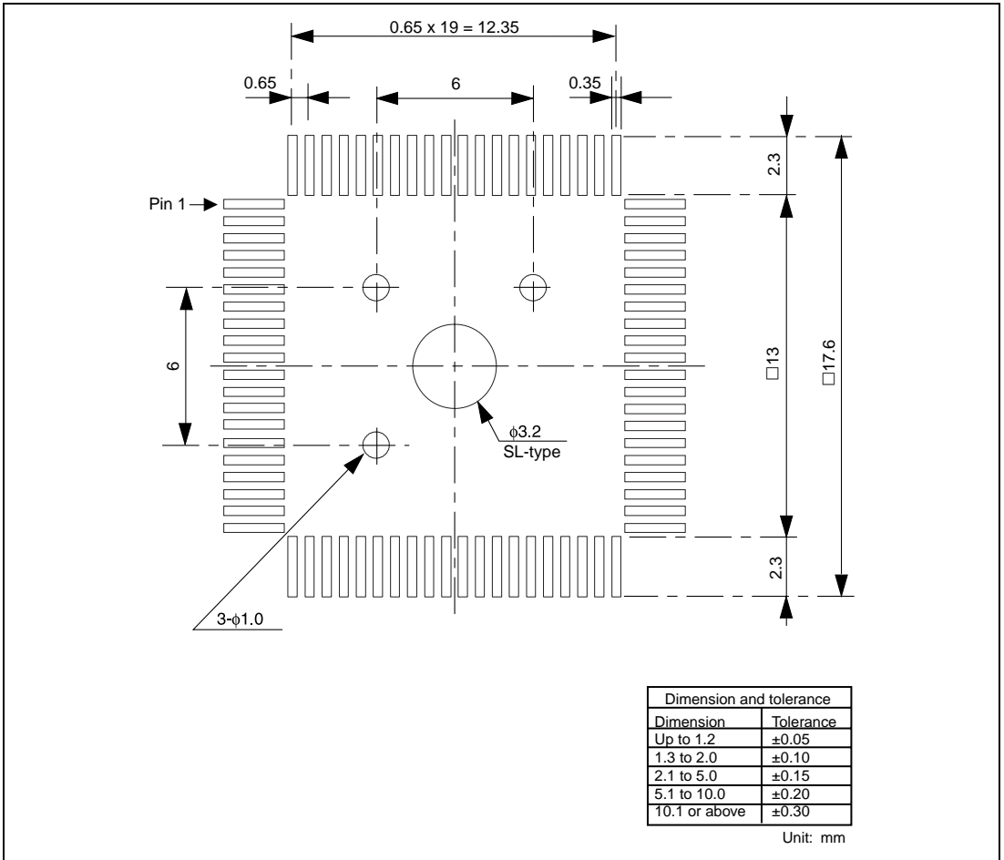
Figure 4 Recommended Dimensions for Mount Pad
