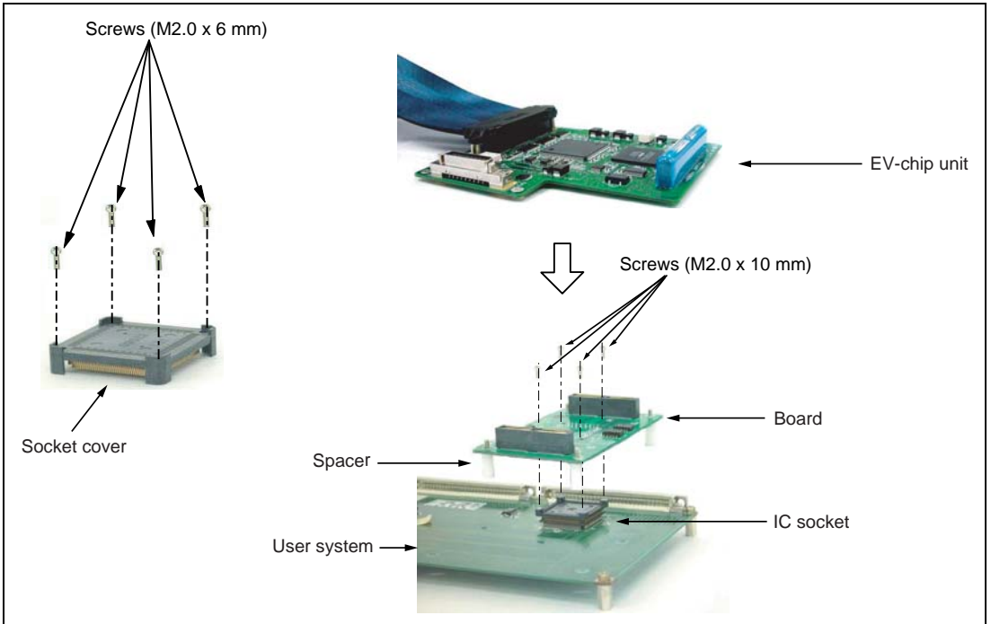
Figure 1 User System Interface Board for the SH7136 PLQP0080JA-A Package
