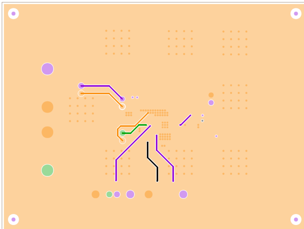
Figure 7. Third Layer
