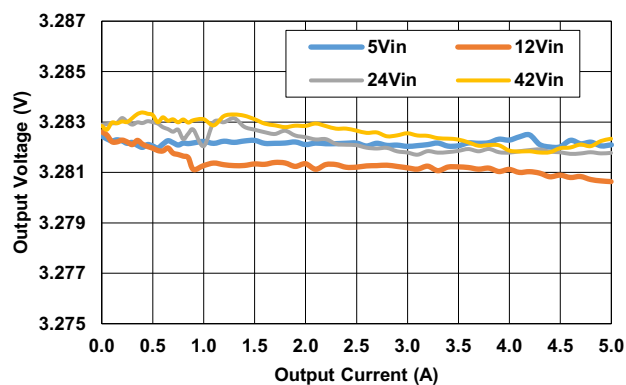
Figure 10. Load Regulation
