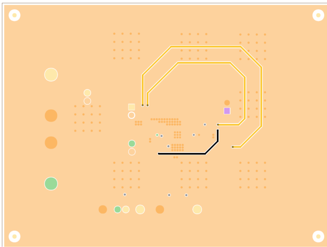
Figure 8. Bottom Layer
