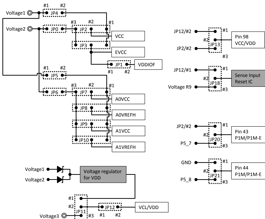
Figure 3 Voltage Distribution on the PiggyBack Board
