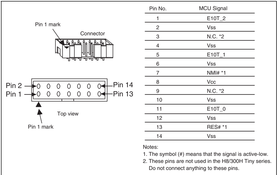
Figure 3.1 Pin Assignments of the Connector
