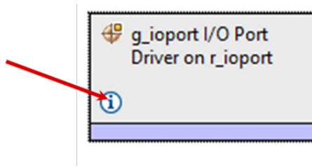
Figure 42: Information icon
