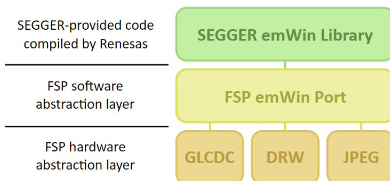
Figure 186: SEGGER emWin FSP Port Block Diagram
