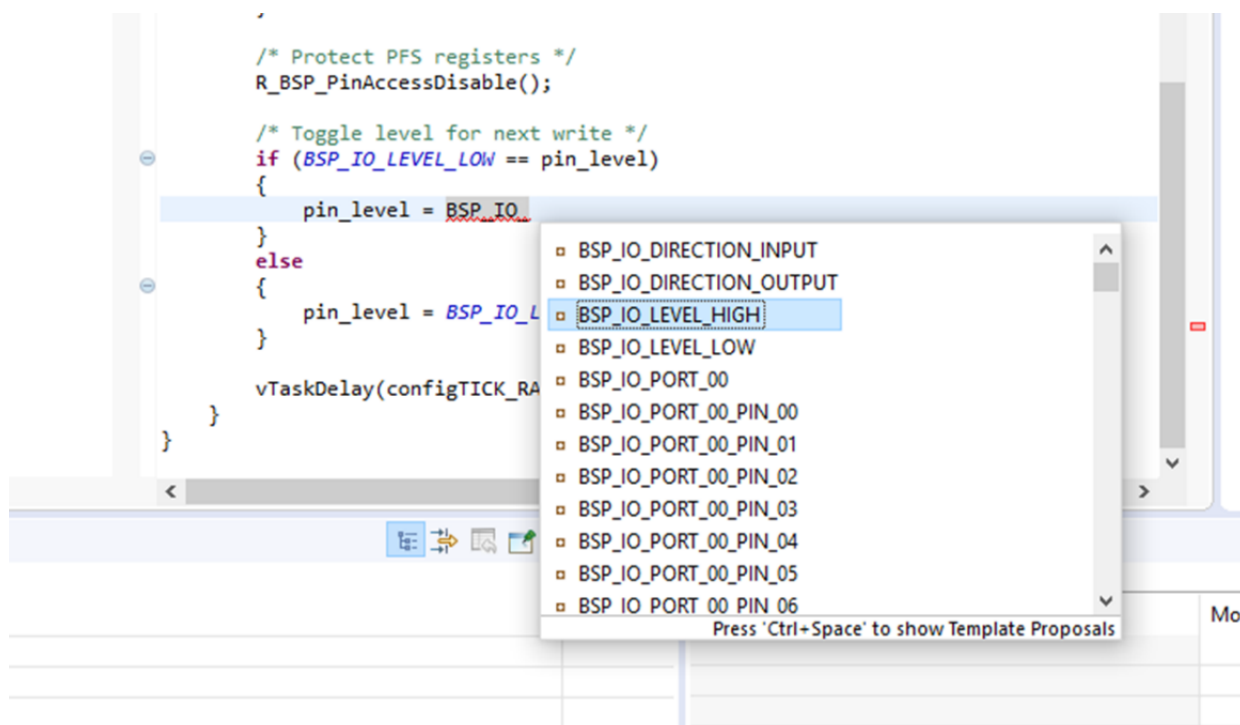
Figure 36: Autocomplete example
