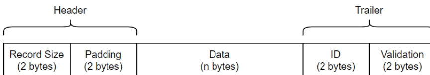
Figure 196: Record Format
