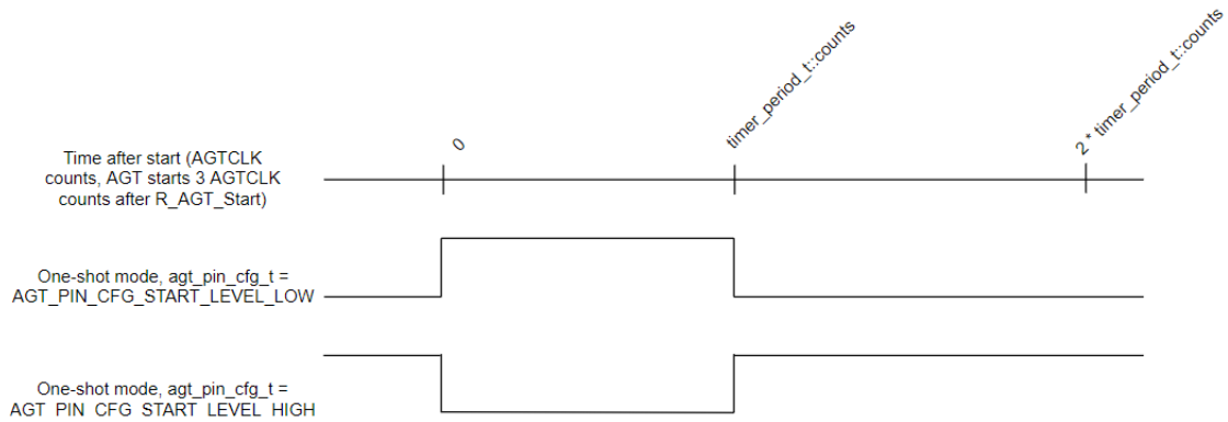
Figure 142: AGT One-Shot Output
