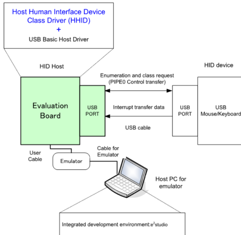
Figure 169: Example Operating Environment
