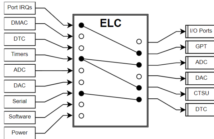
Figure 149: Event Link Controller Conceptual Diagram
