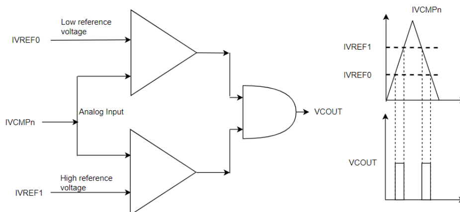
Figure 141: ACMPLP Window Mode Operation
