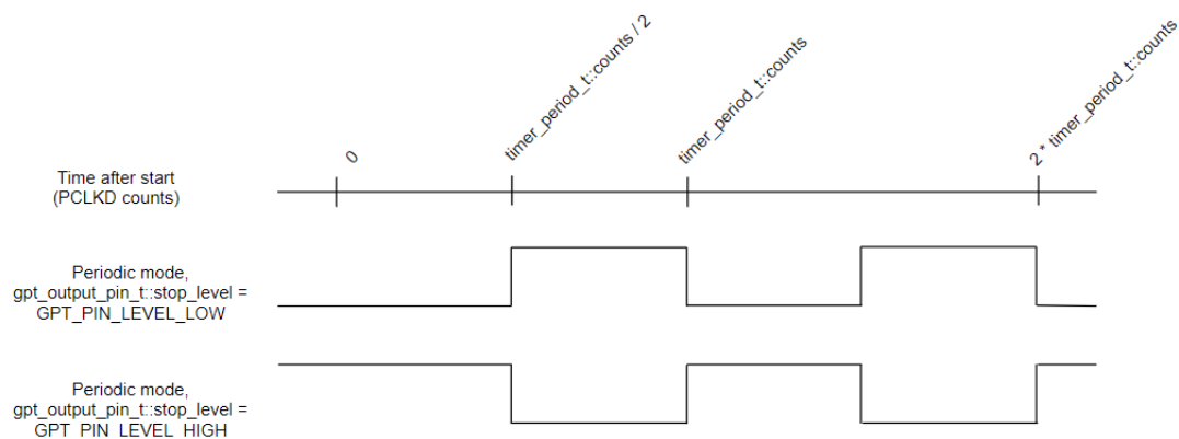
Figure 156: GPT Periodic Output
