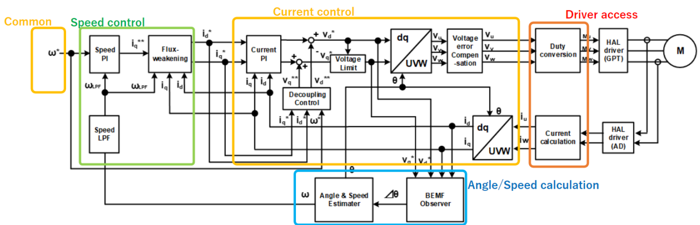
Figure 191: Image of Speed Module(green block)
