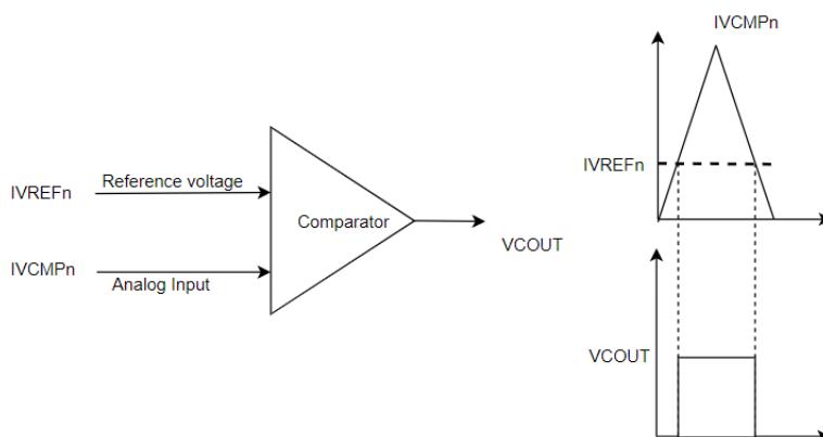
Figure 140: ACMPLP Standard Mode Operation
