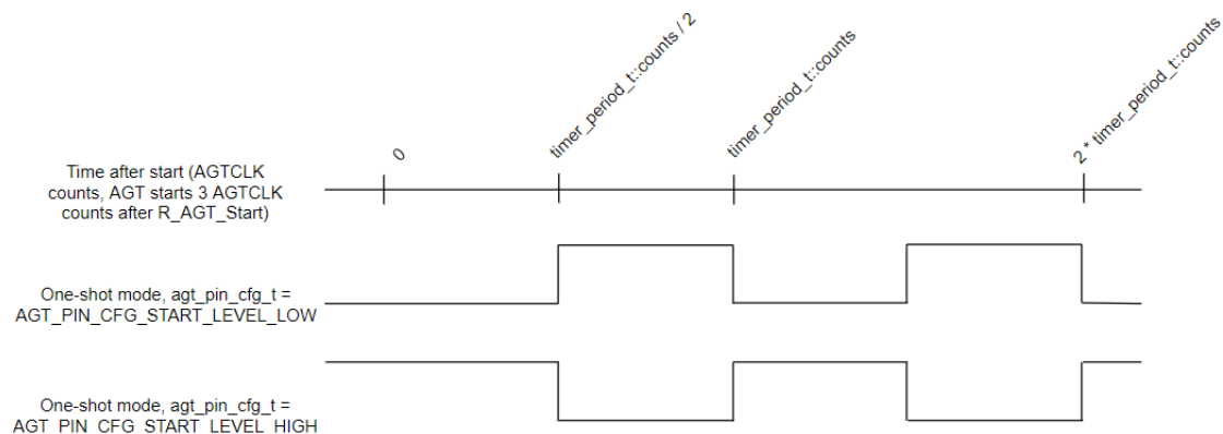
Figure 143: AGT Periodic Output
