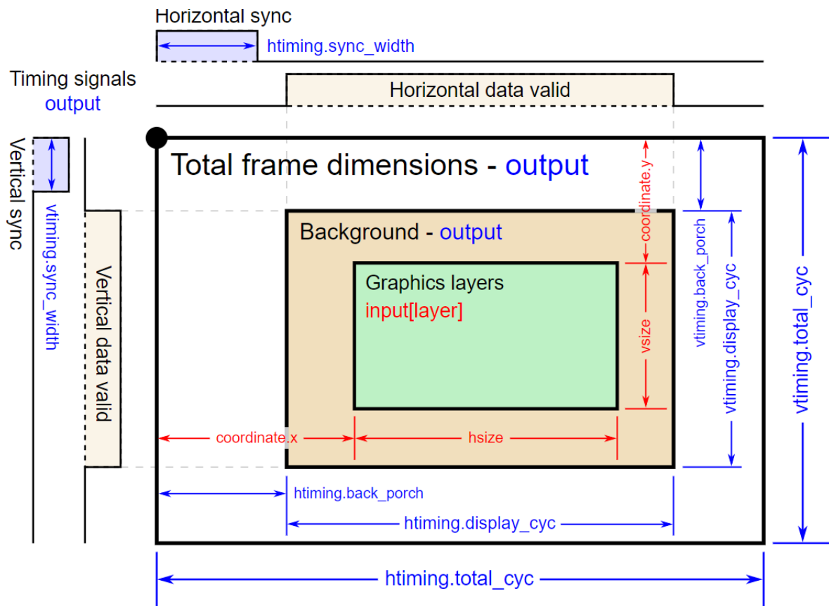
Figure 154: GLCDC layers and timing
