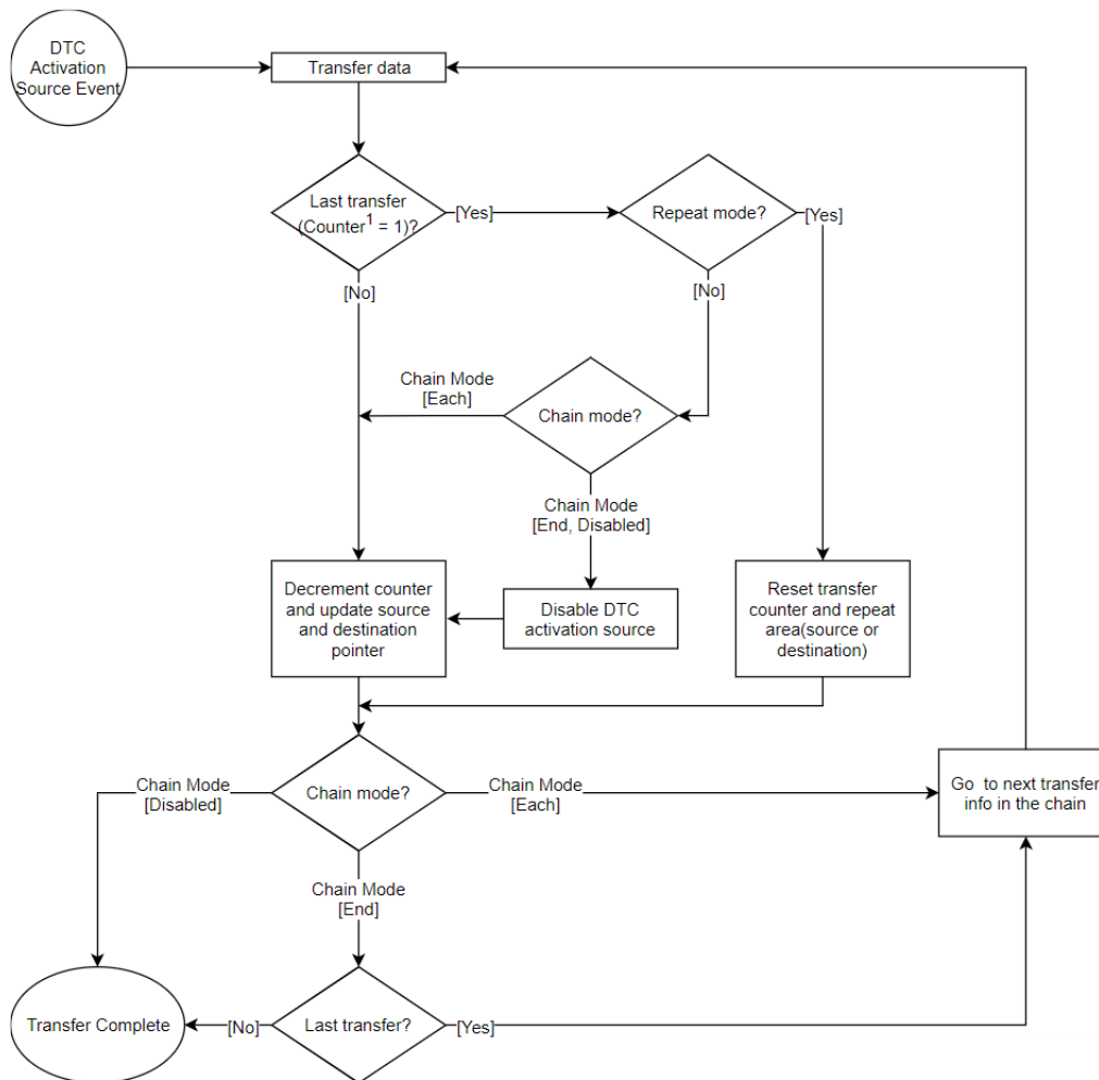
Figure 148: DTC Transfer Flowchart
