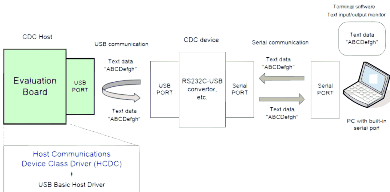
Figure 168: Data Transfer (Loopback)
