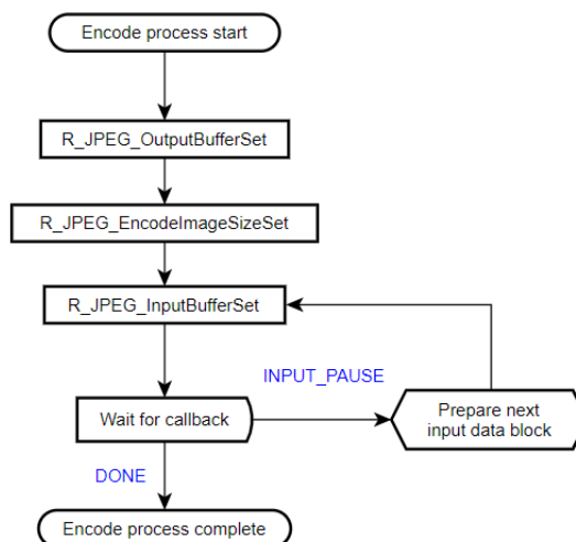
Figure 161: JPEG Encode Operational Flow
