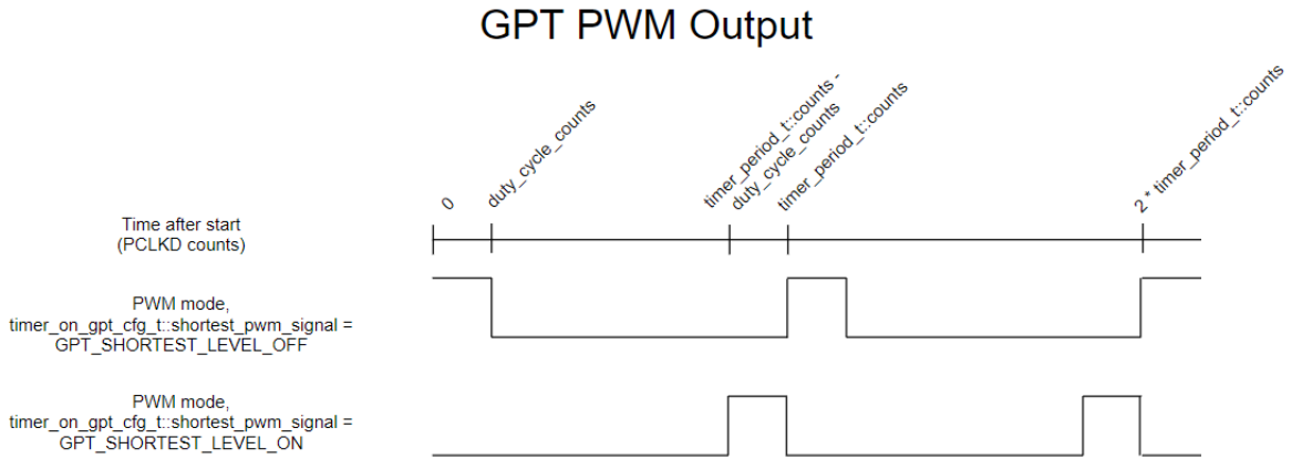
Figure 157: GPT PWM Output
