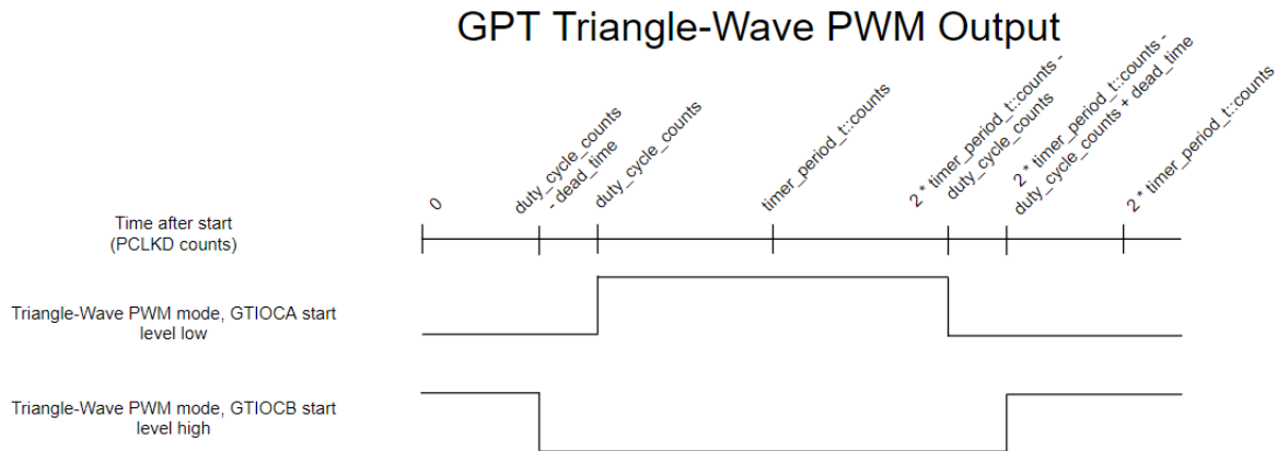
Figure 158: GPT Triangle-Wave PWM Output
