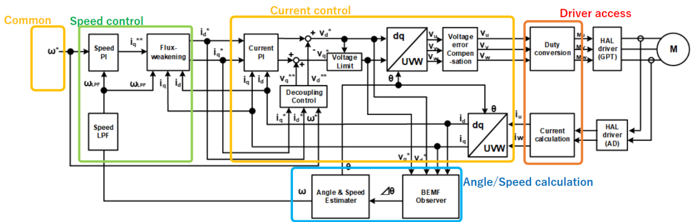
Figure 187: Image of Current Control Module(yellow block)
