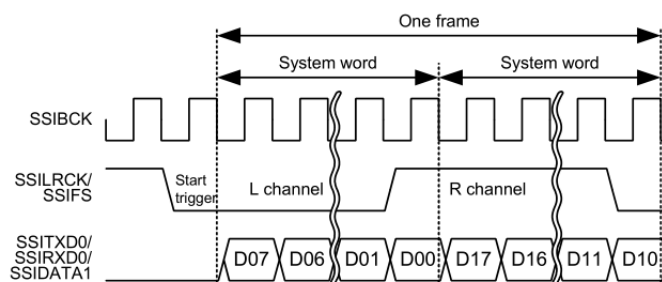
Figure 162: SSI Frame Diagram (8-bit word, 8-bit samples)
