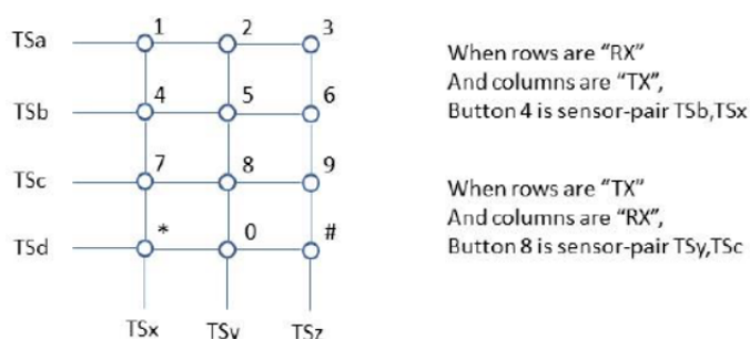
Figure 146: Mutual Button Image
