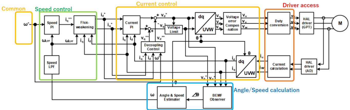
Figure 189: Image of Angle and Speed Estimation Module(blue block)
