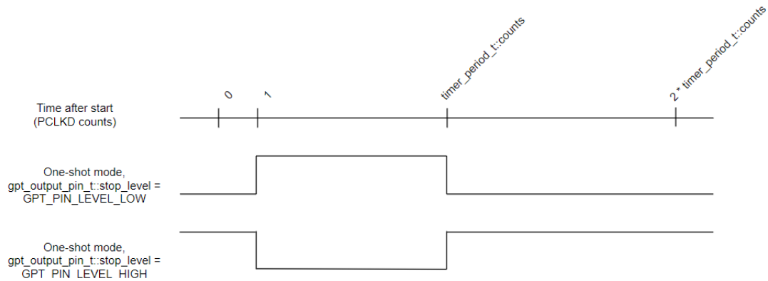
Figure 155: GPT One-Shot Output
