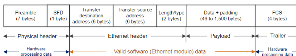
Figure 151: Frame Format Image
