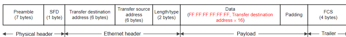
Figure 153: Magic Packet Frame Format Image
