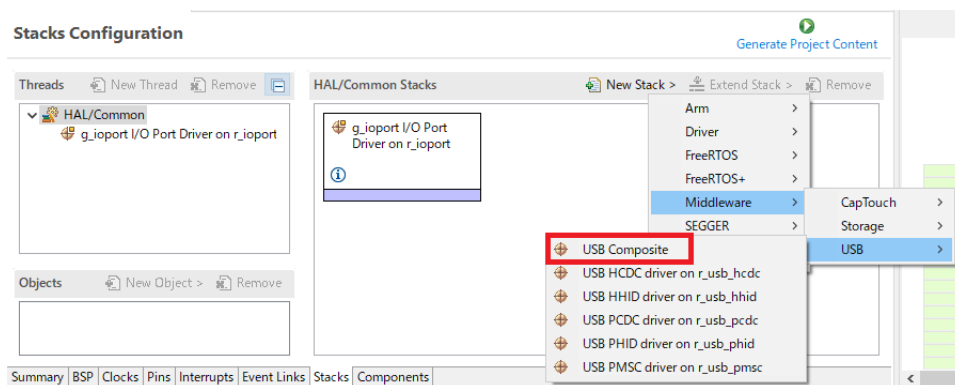
Figure 163: Select USB Composite
