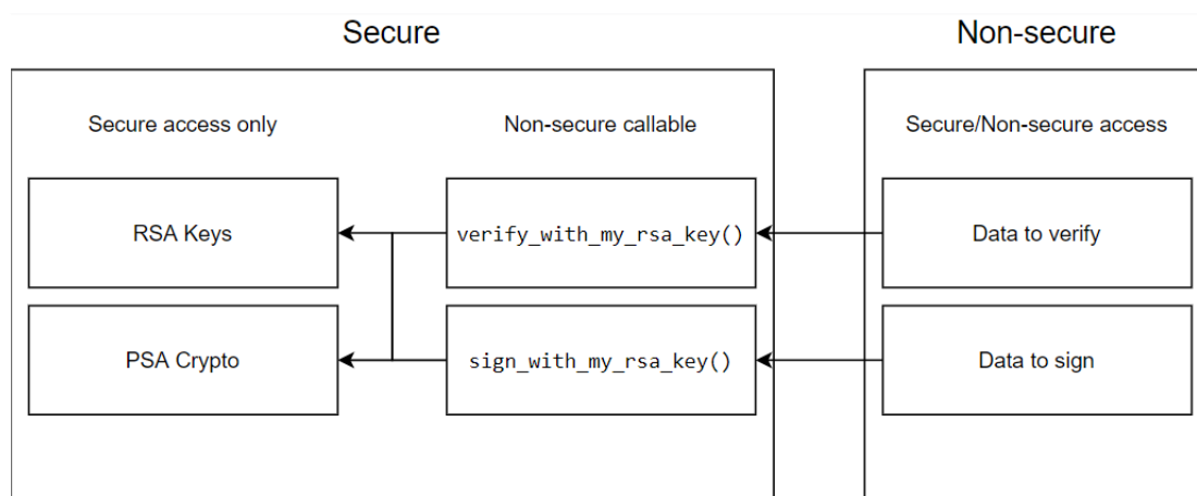
Figure 192: PSA Crypto Non-secure callable example
