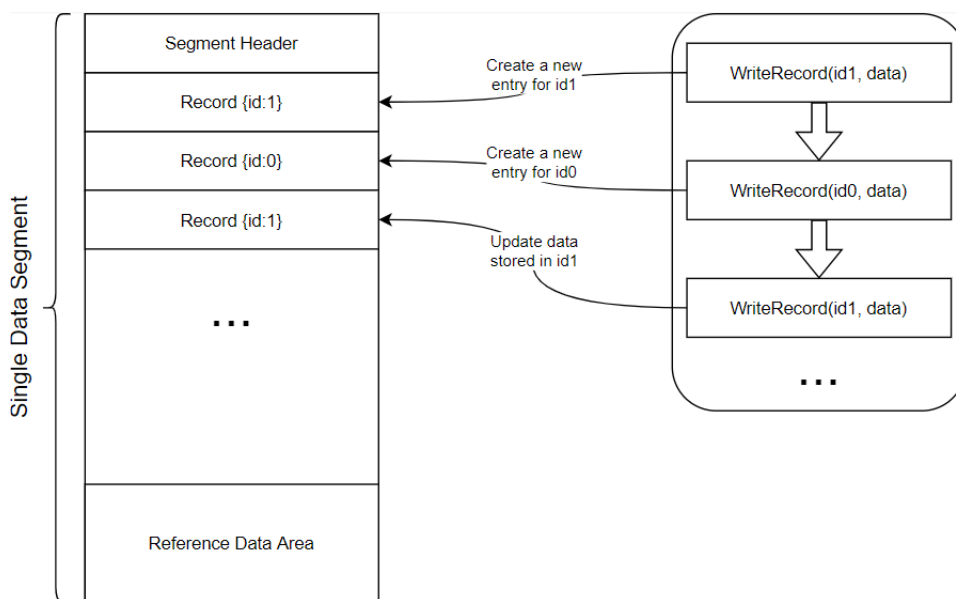
Figure 194: Segment Data Format
