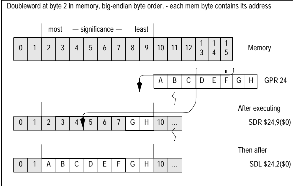
Figure 2.16 Unaligned Doubleword Store with SDR and SDL
