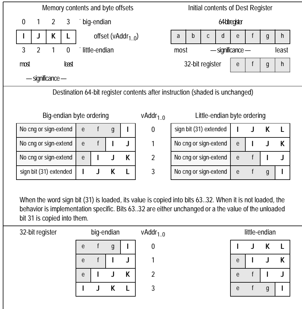
Figure 2.14 Bytes Loaded by LWR Instruction
