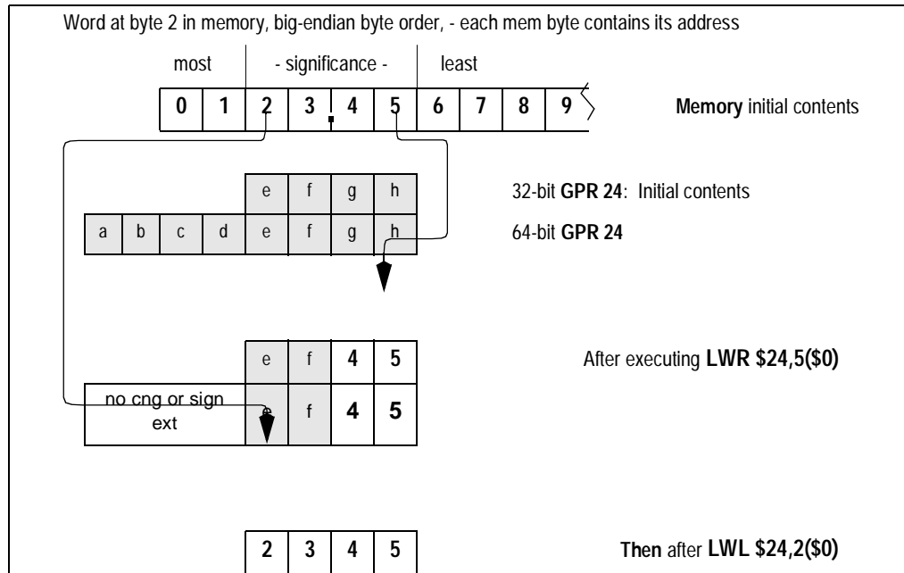
Figure 2.13 Unaligned Word Load using LWR and LWL
