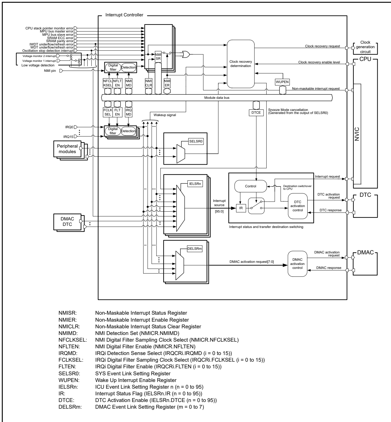
Figure 10.1 ICU block diagram
