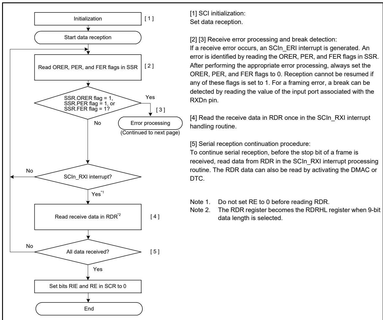
Figure 32.17 Example flow of serial reception in asynchronous mode with non-FIFO selected (1)
