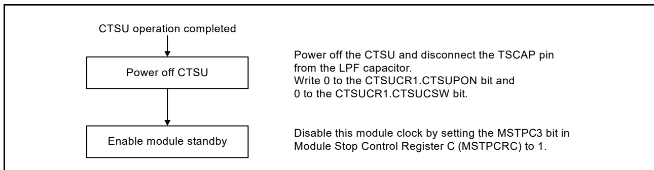
Figure 49.10 CTSU stopping flow
