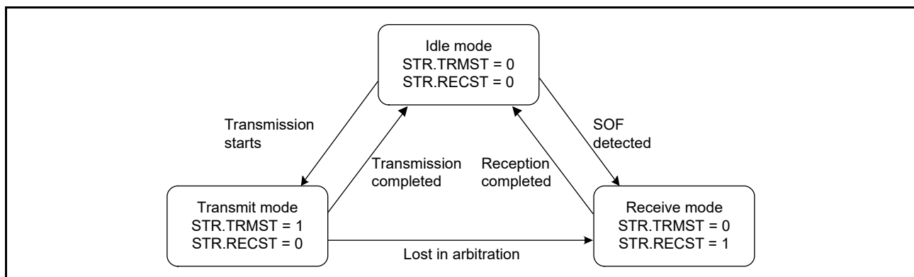
Figure 35.10 Sub-modes of CAN operation mode
