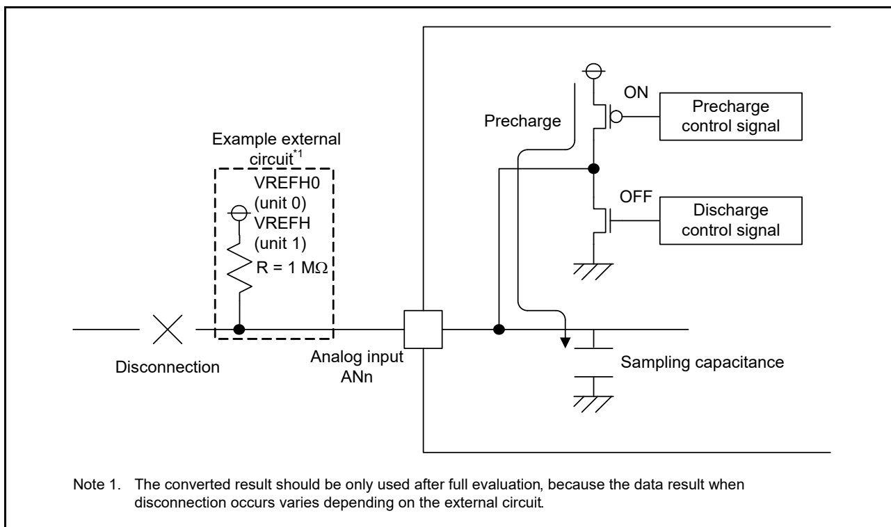
Figure 45.37 Example of disconnection detection when precharge is selected
