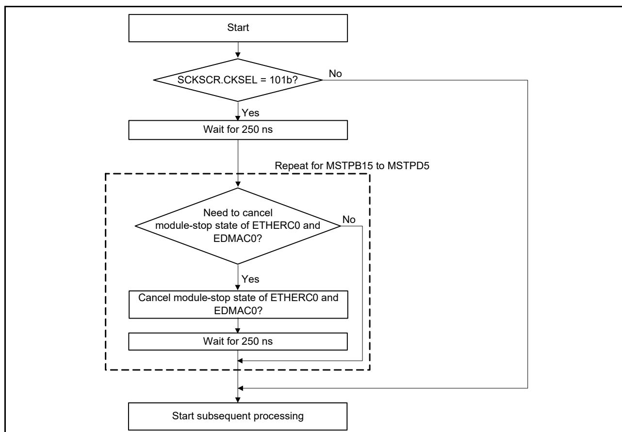
Figure 12.3 Example flow for canceling Software Standby mode
