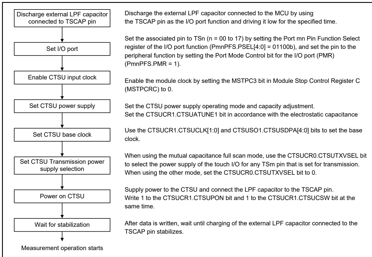
Figure 49.9 CTSU initial settings flow
