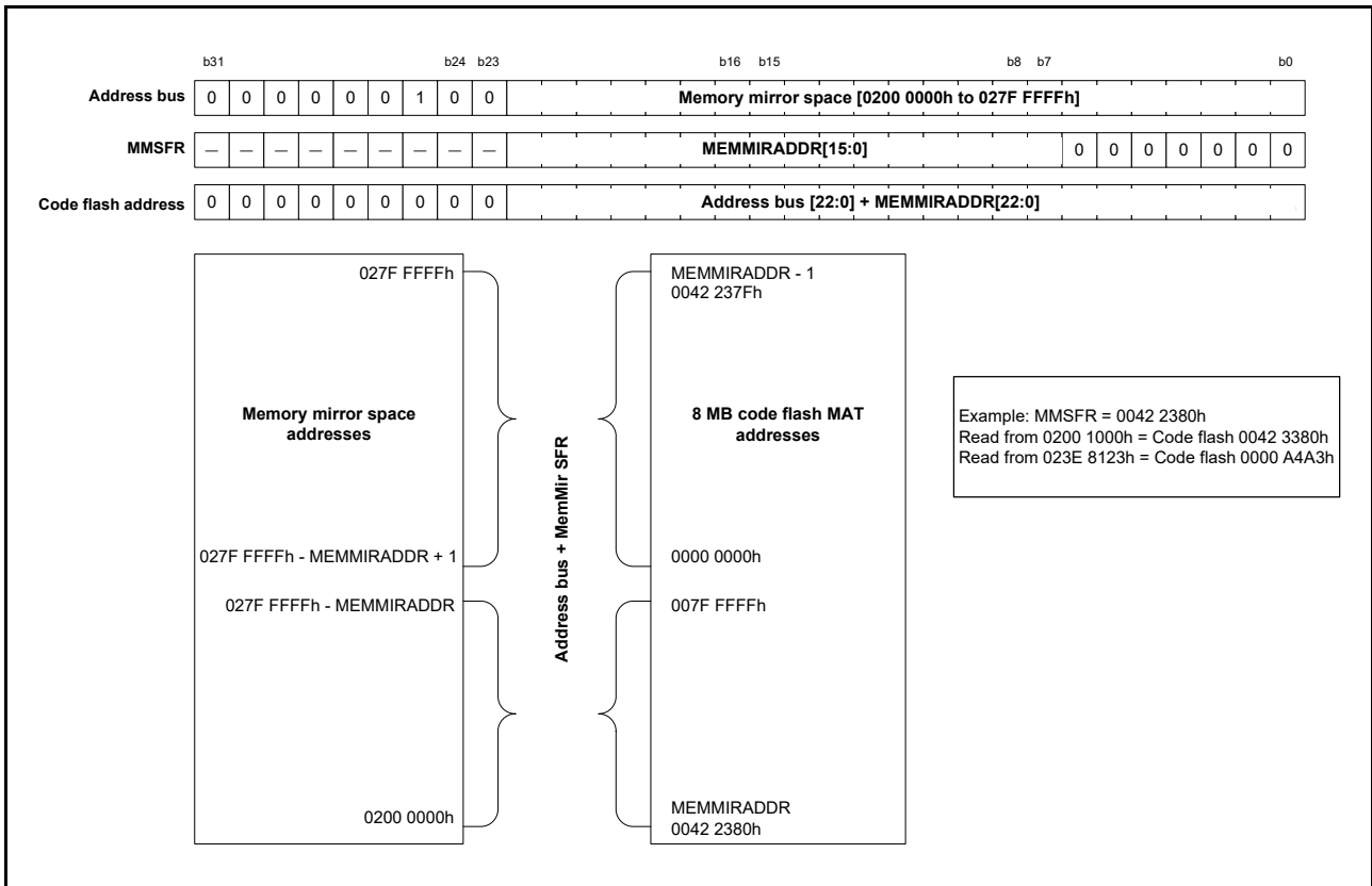
Figure 5.1 MMF operation
