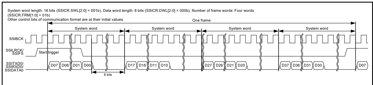
Figure 39.42 TDM format (with padding: system word length > data word length)
