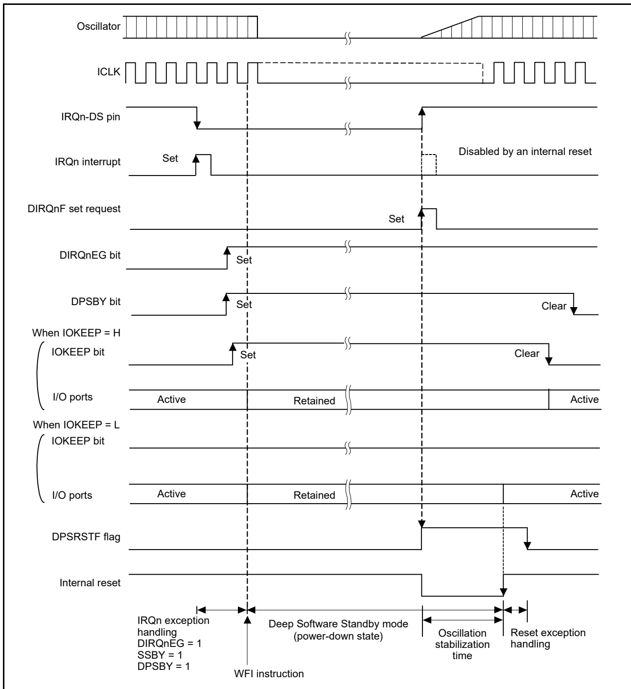
Figure 12.10 Example of Deep Software Standby mode application
