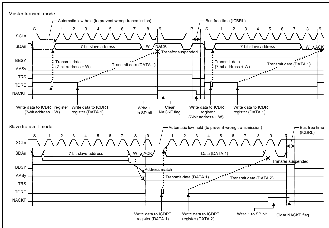
Figure 34.39 Suspension of data transfer when NACK is received, when NACKCE = 1
