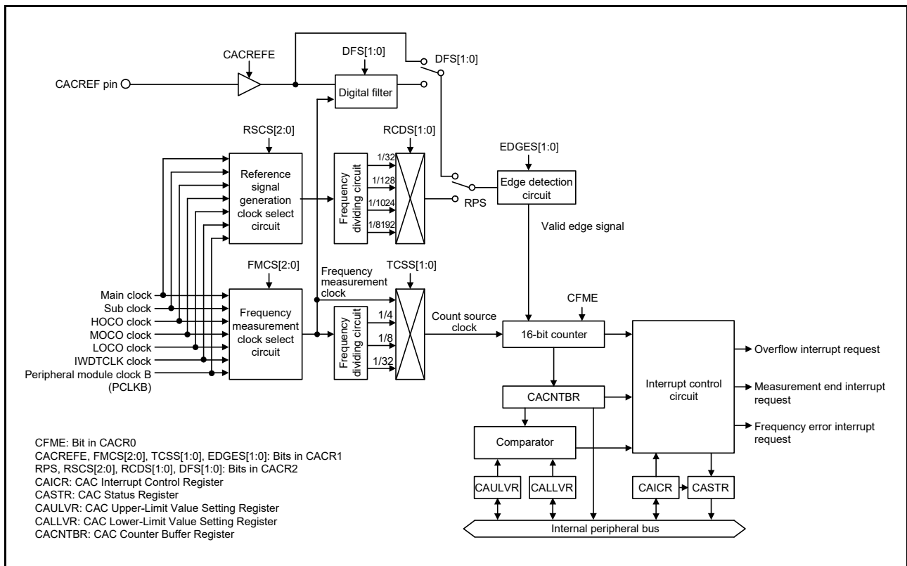
Figure 11.1 CAC block diagram
