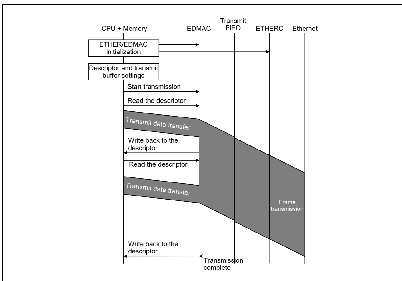
Figure 30.5 Example of transmission flow
