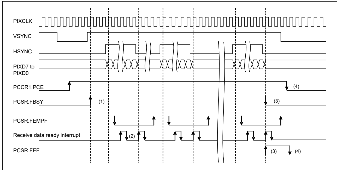
Figure 42.11 Example of reception operations
