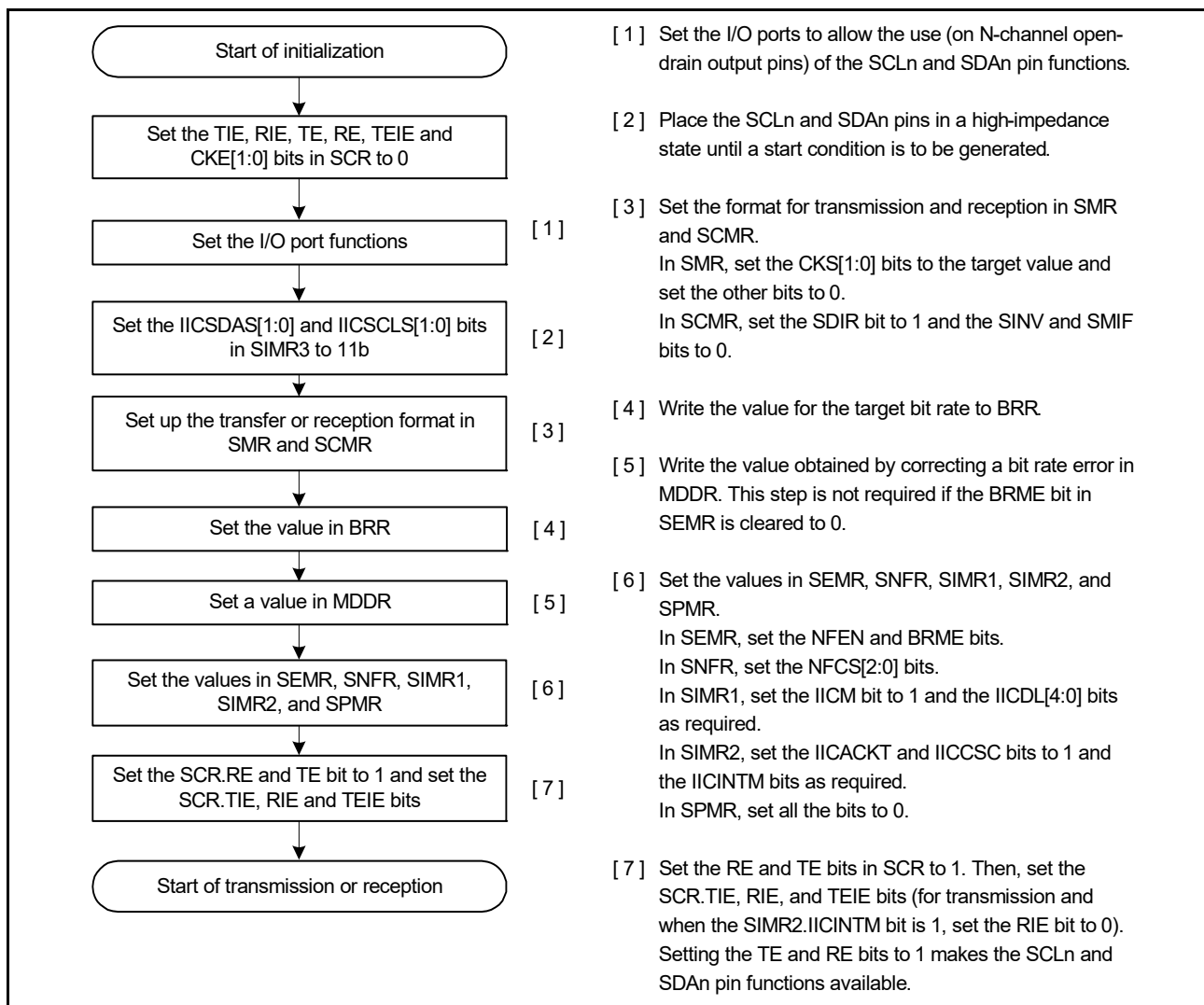
Figure 32.63 Example flow of SCI initialization in simple IIC mode
