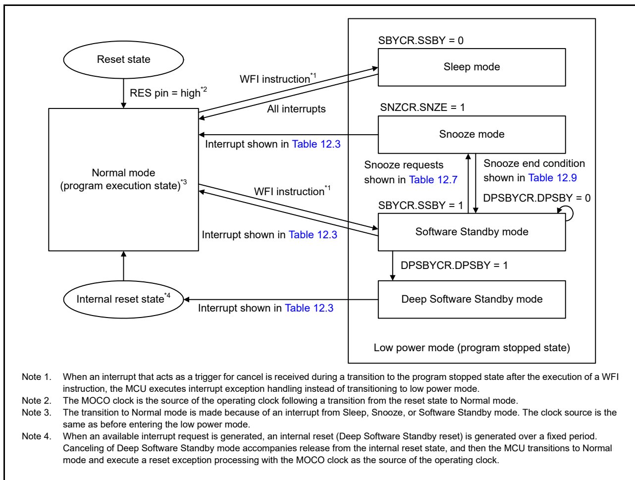
Figure 12.1 Mode transitions
