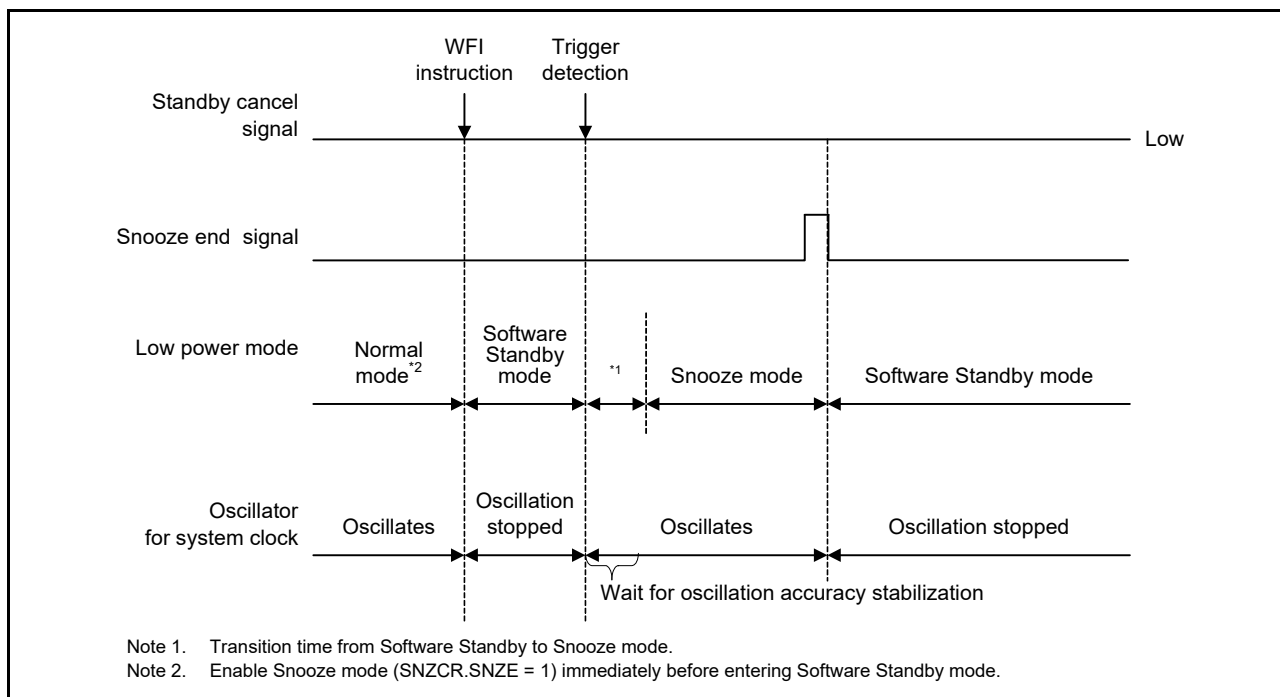
Figure 12.7 Canceling of Snooze mode when interrupt request signal is not generated
