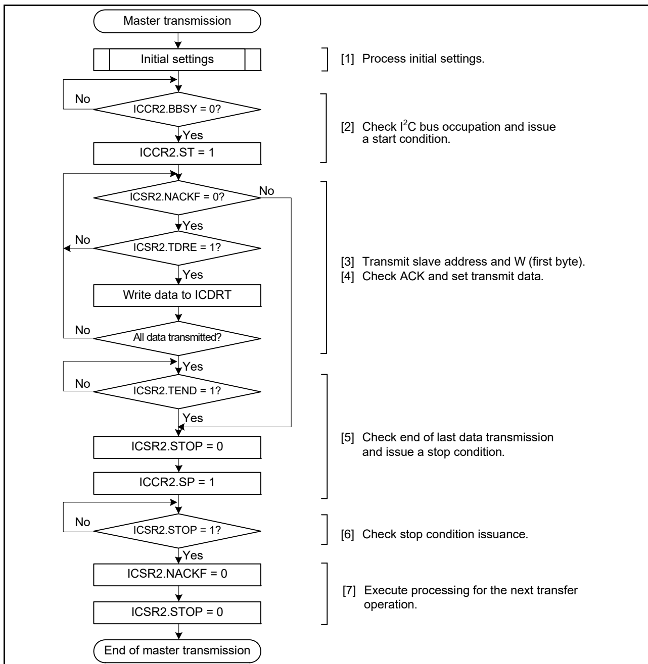
Figure 34.6 Example master transmission flow
