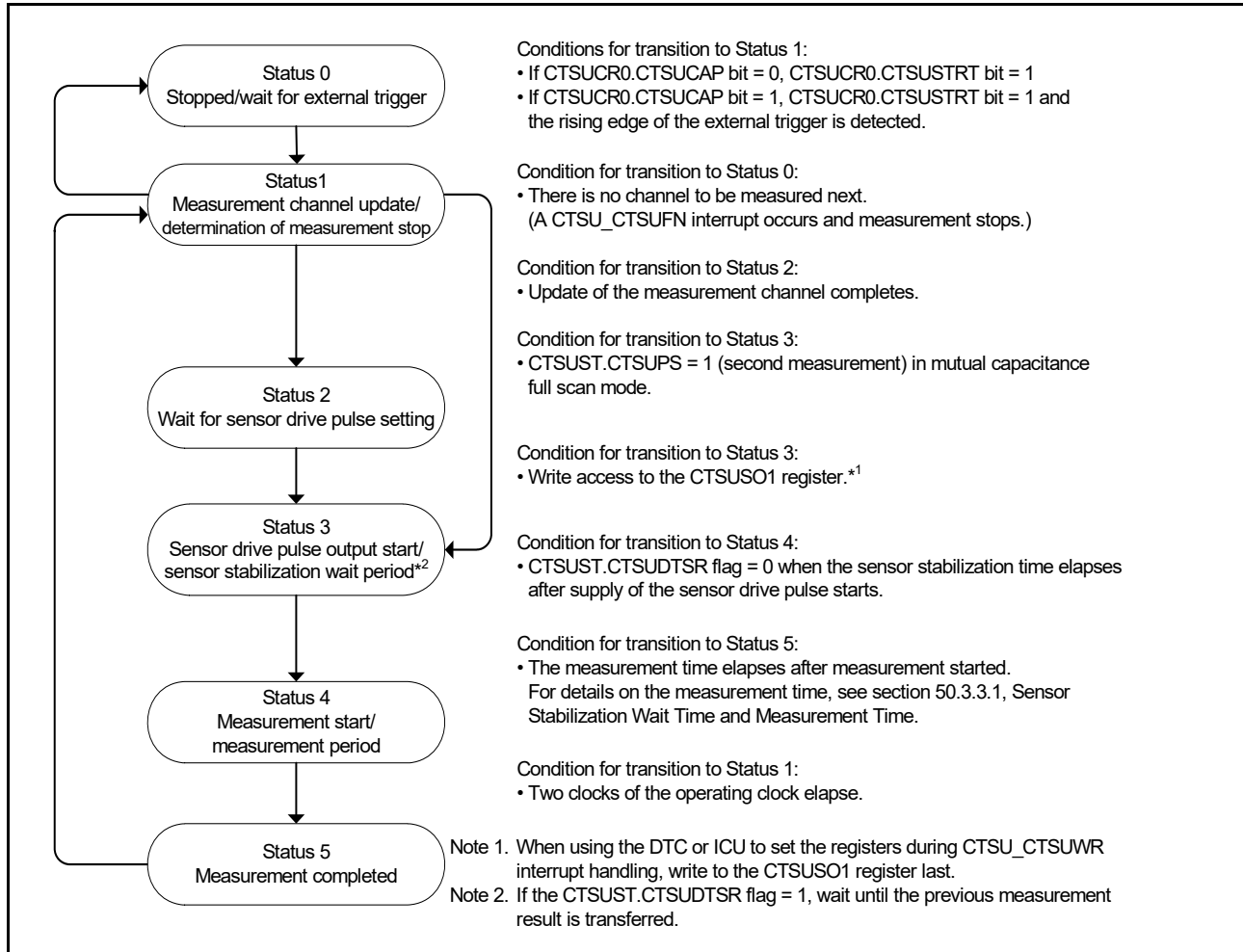
Figure 49.11 Status operation transitions
