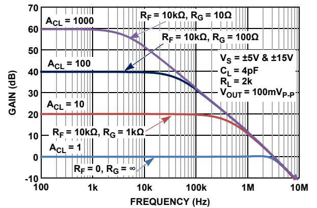
FIGURE 14. FREQUENCY RESPONSE vs CLOSED LOOP GAIN
