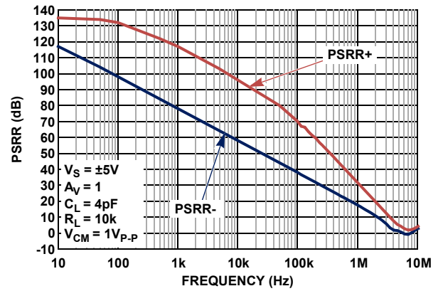
FIGURE 12. PSRR vs FREQUENCY, V_S = \pm 5V
