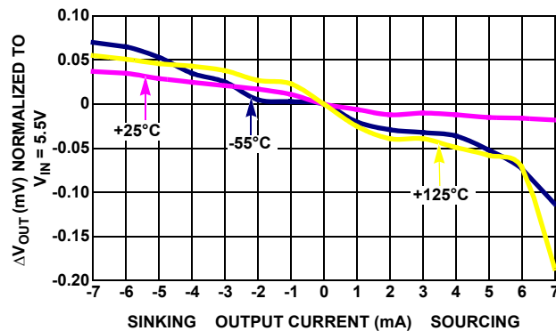
FIGURE 34. LOAD REGULATION
