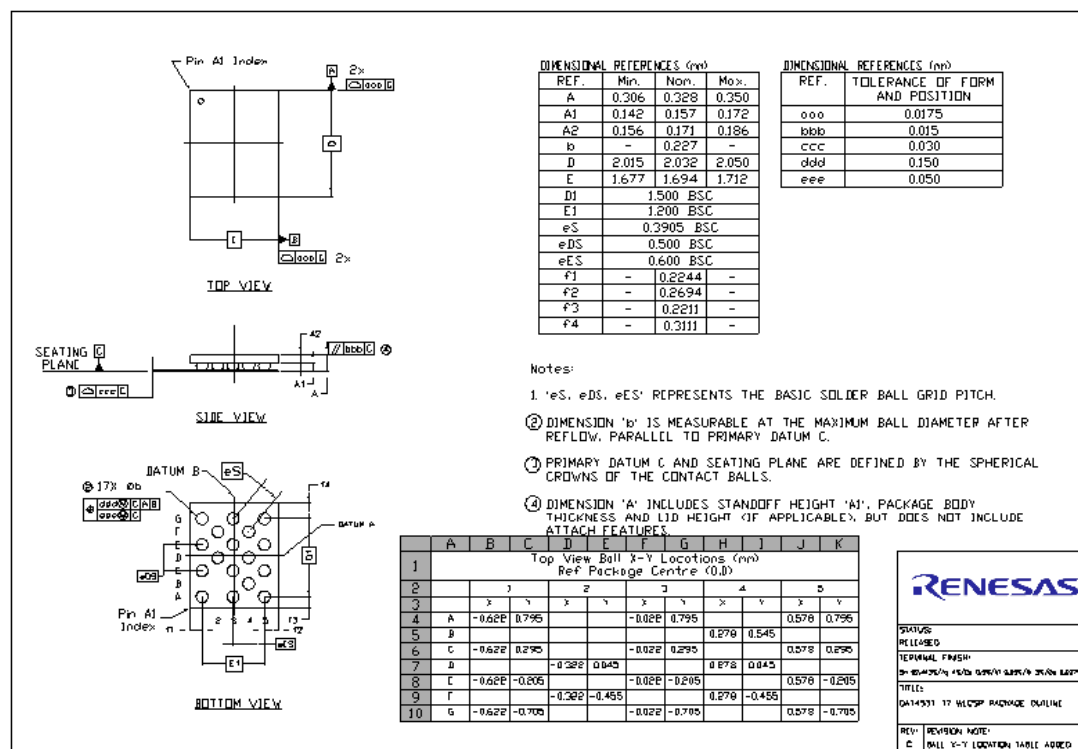
Figure 86. FCGQFN24 package outline drawing
