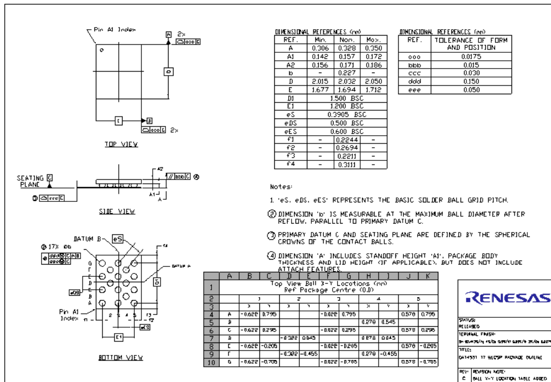
Figure 85. WLCSP17 package outline drawing
