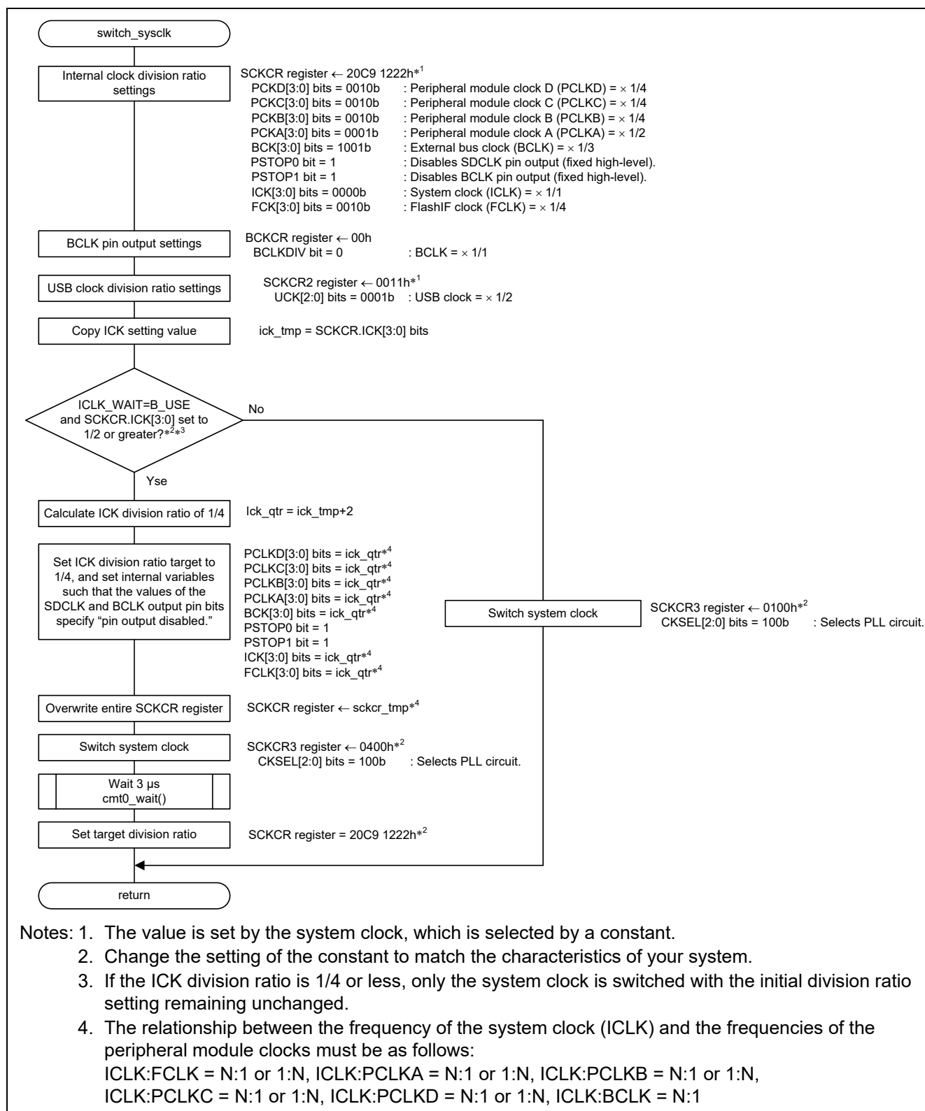
Figure 3.14 System Clock Switching
