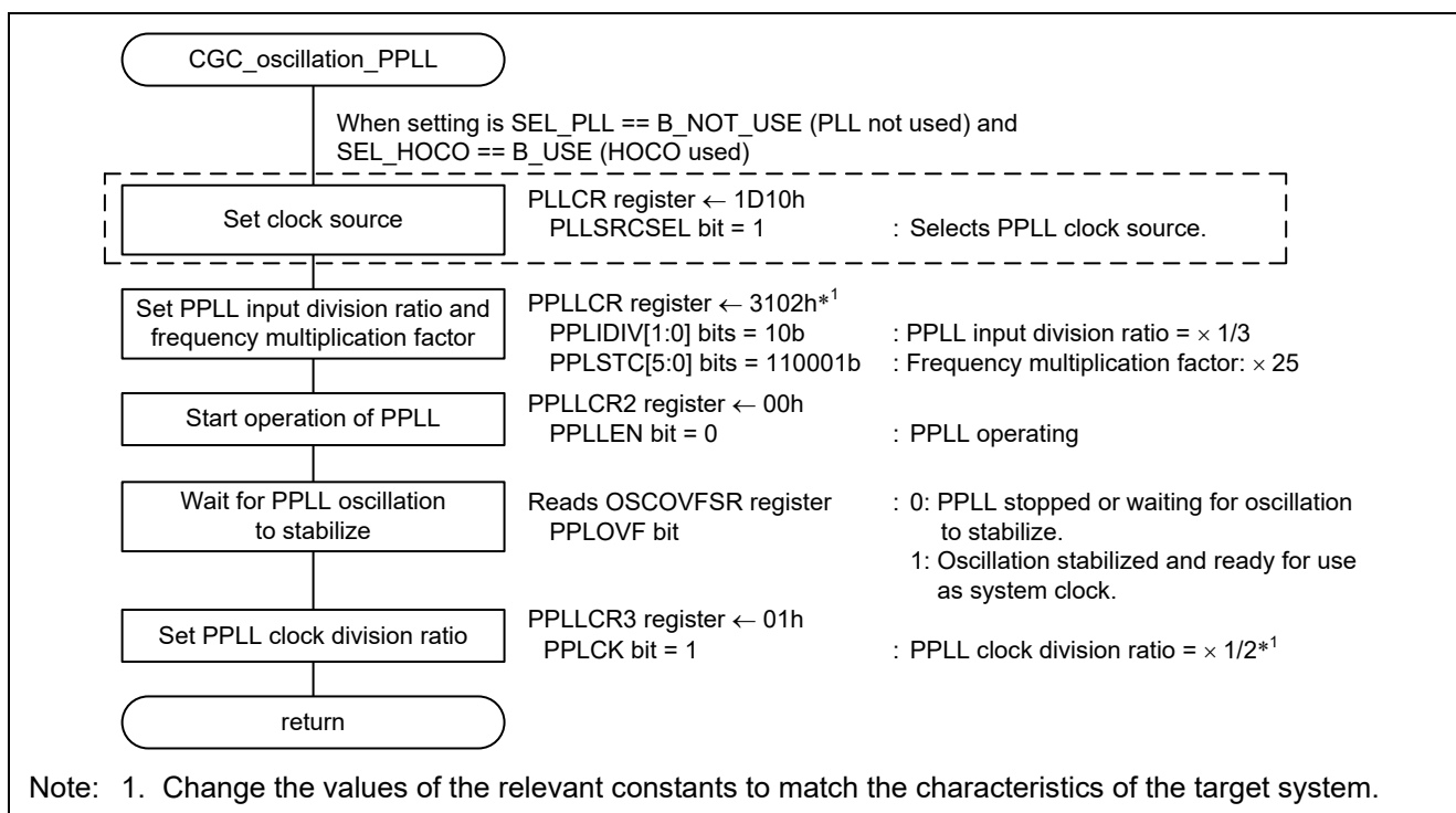
Figure 3.10 PPLL Clock Oscillation Enable
