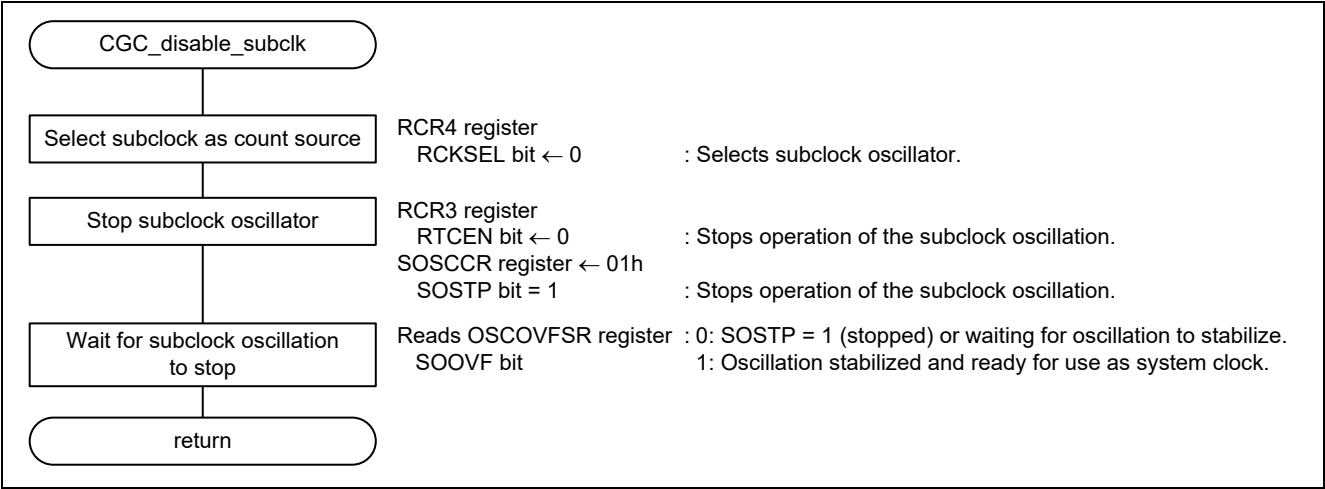
Figure 3.13 Subclock Disable
