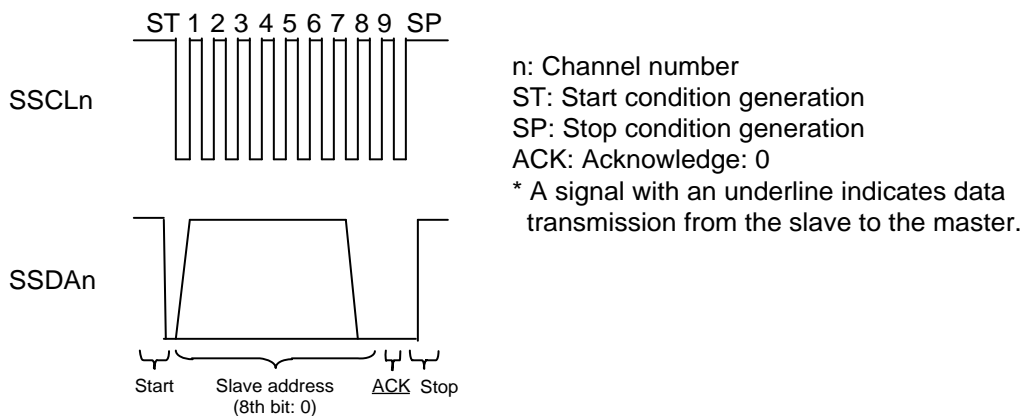
Figure 1.4 Signals for Pattern 3 of Master Transmission
