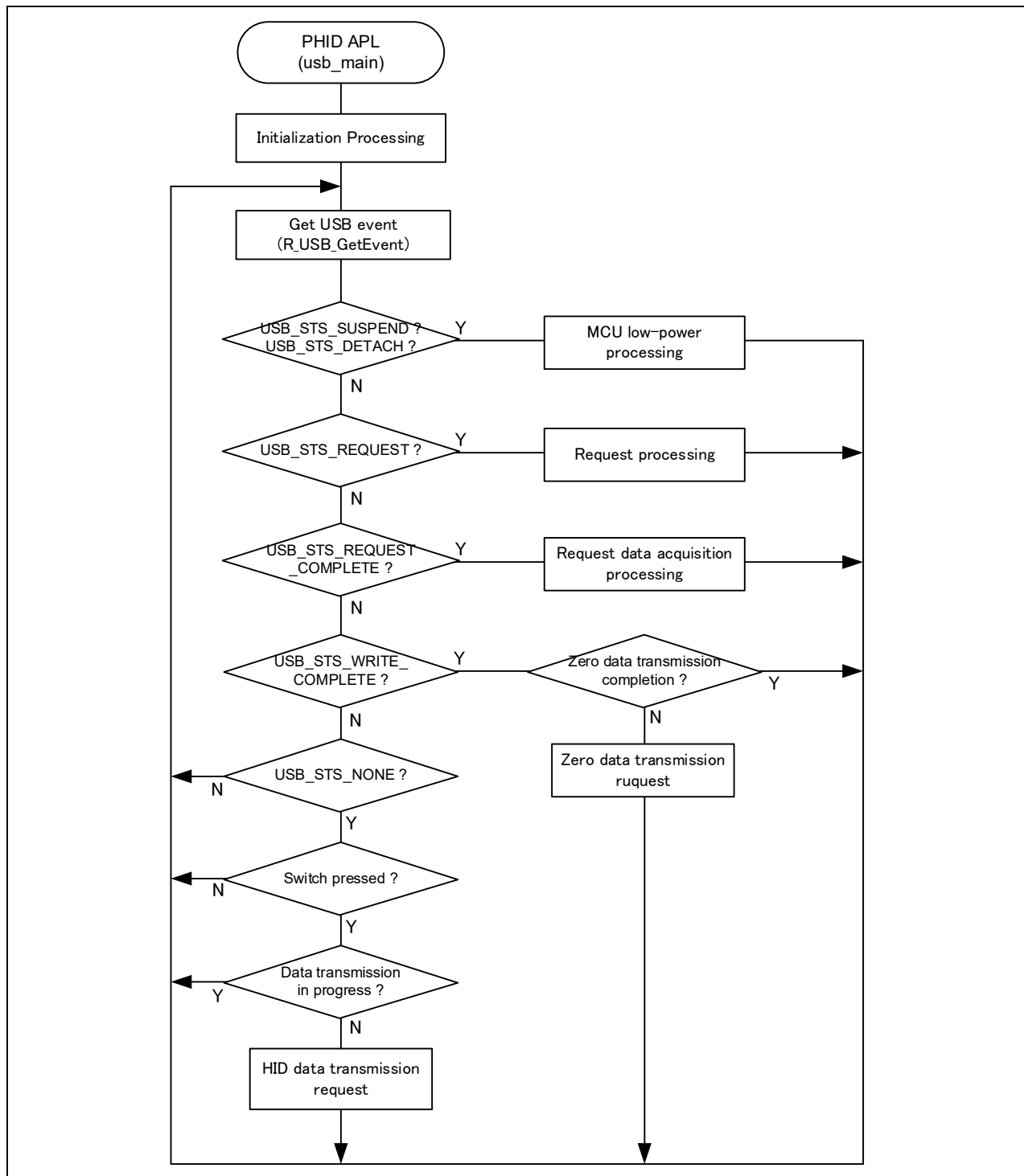
Figure 4-1 Main Loop Processing (Keyboard mode)
