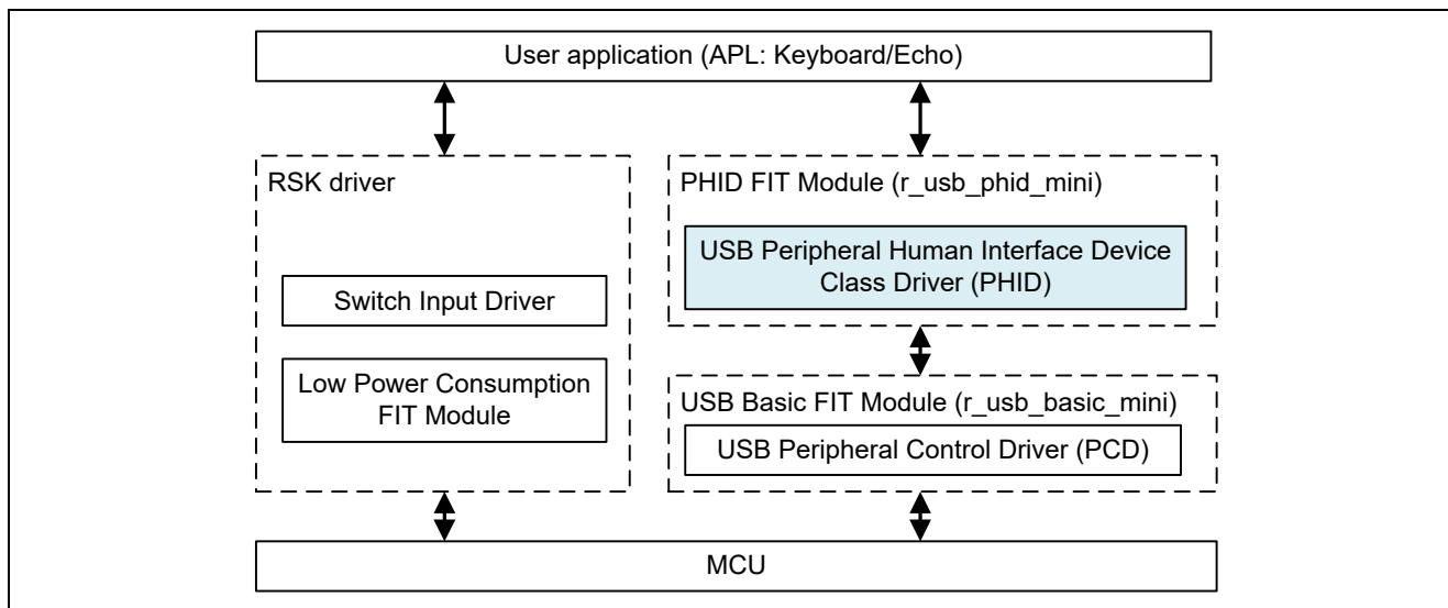
Figure 2-1 Module Configuration
